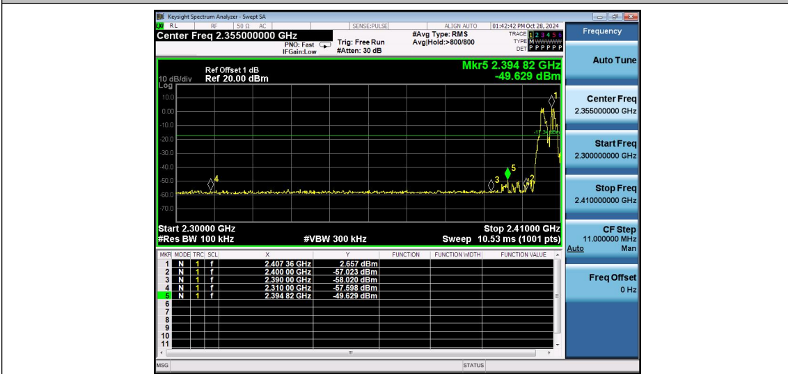
2.4G-Ant1-Hop-PASS
