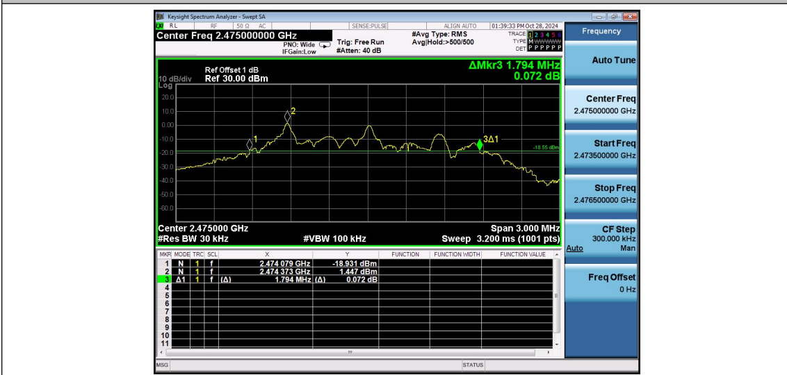
2.4G-Ant1-2475
