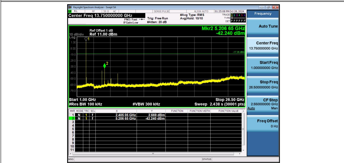
2.4G-Ant1-2405-1000~26500-PASS
