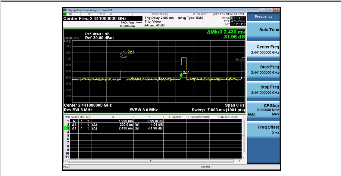
NTNV-2.4G-Ant1-2441
