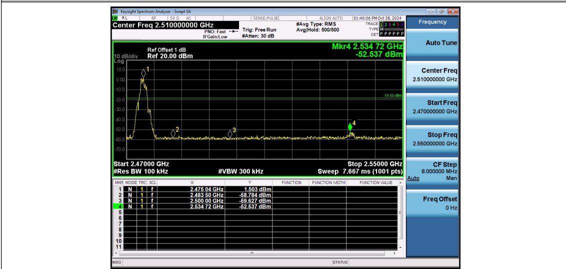
2.4G-Ant1-2475-PASS
