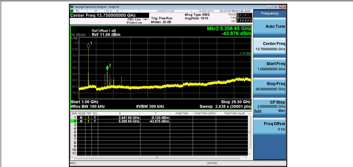
2.4G-Ant1-2441-1000~26500-PASS
