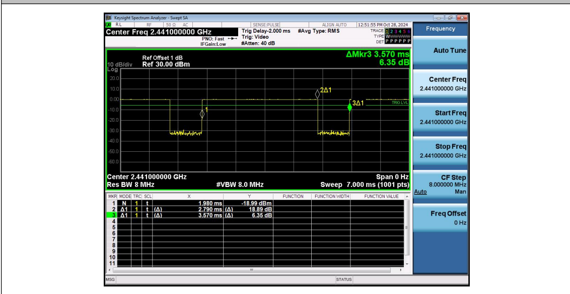
NTNV-DH5-Ant1-2441
