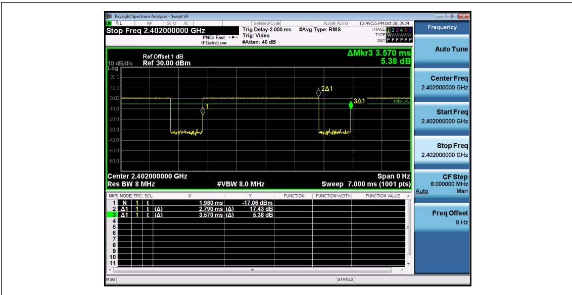
NTNV-DH5-Ant1-2402
