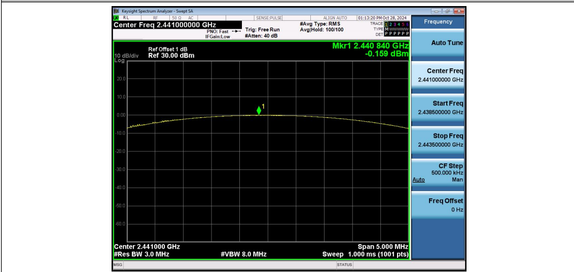
DH5-Ant1-2441-PASS
