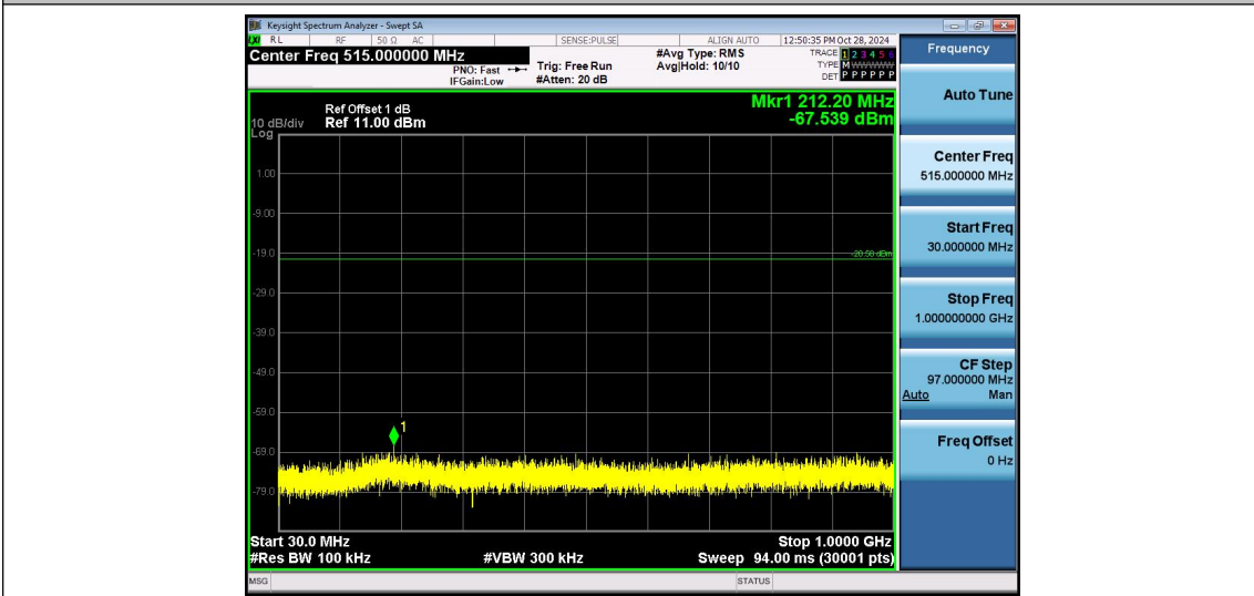
DH5-Ant1-2402-30~1000-PASS
