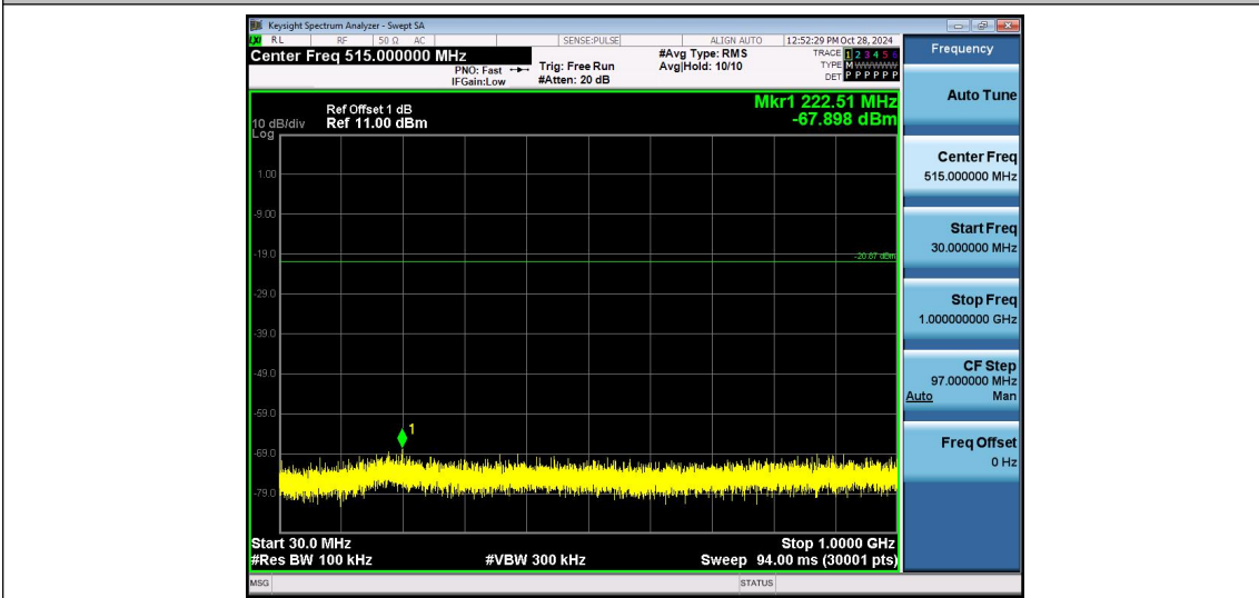
DH5-Ant1-2441-30~1000-PASS
