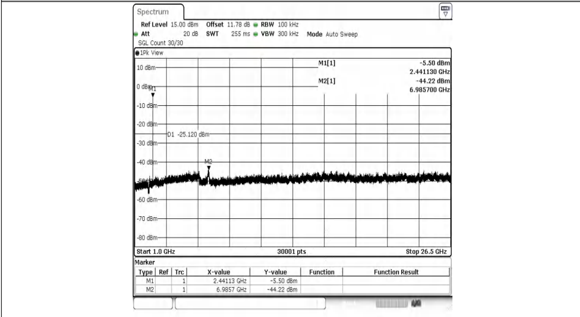
3DH5-Ant1-2441-1000~26500-PASS
