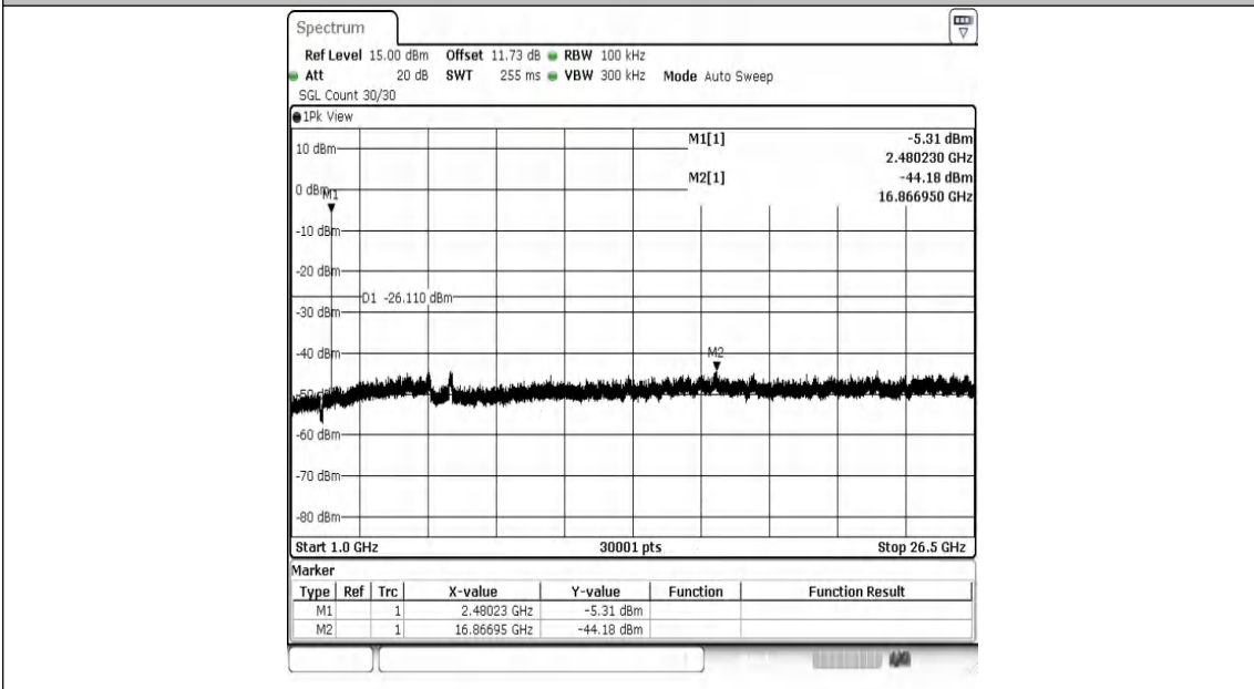
2DH5-Ant1-2480-1000~26500-PASS
