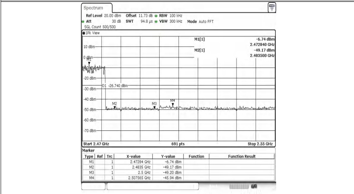
2DH5-Ant1-Hop_2480-PASS
