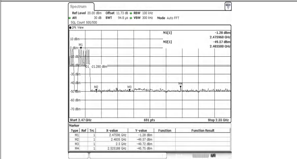
DH5-Ant1-Hop_2480-PASS
