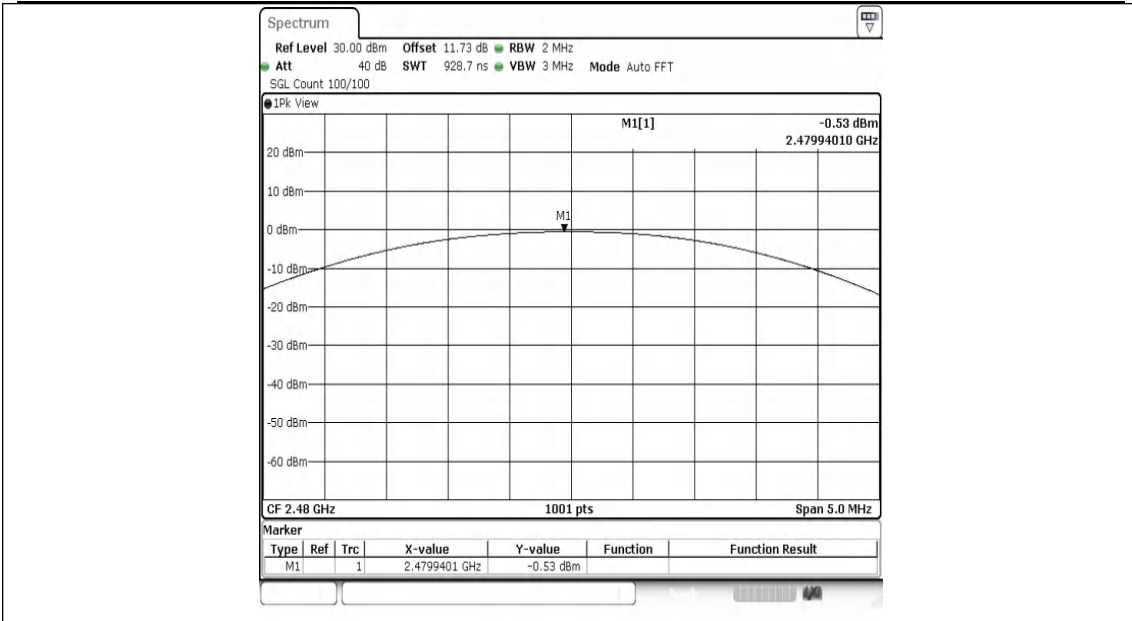
DH5-Ant1-2480-PASS
