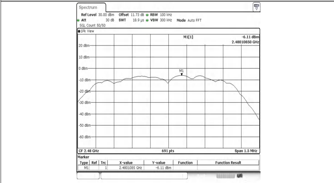
2DH5-Ant1-2480-0~Reference-PASS
