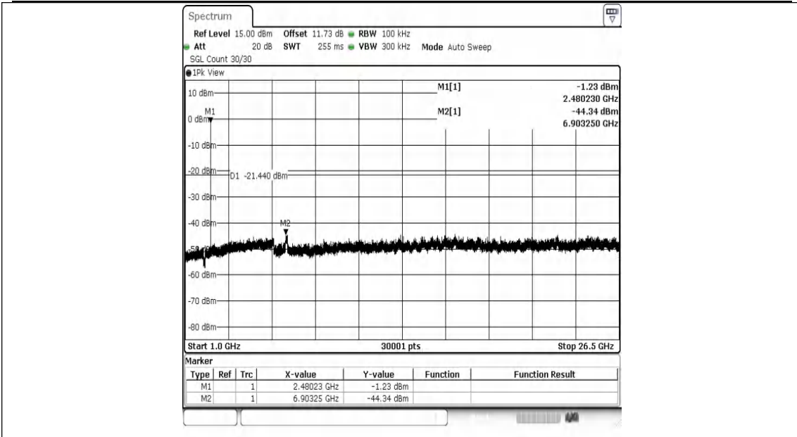
DH5-Ant1-2480-1000~26500-PASS
