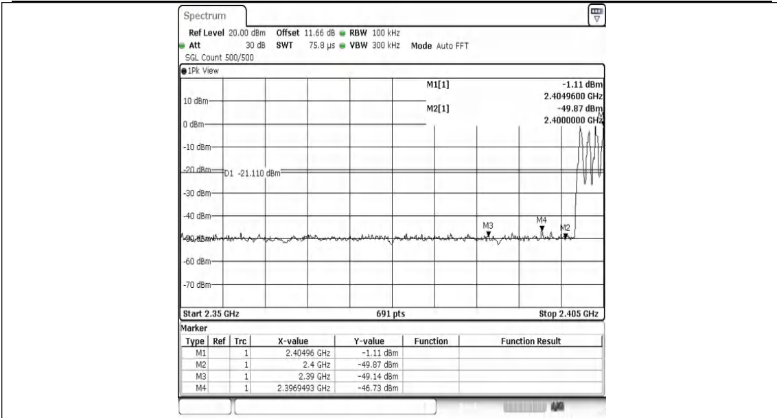
DH5-Ant1-Hop_2402-PASS
