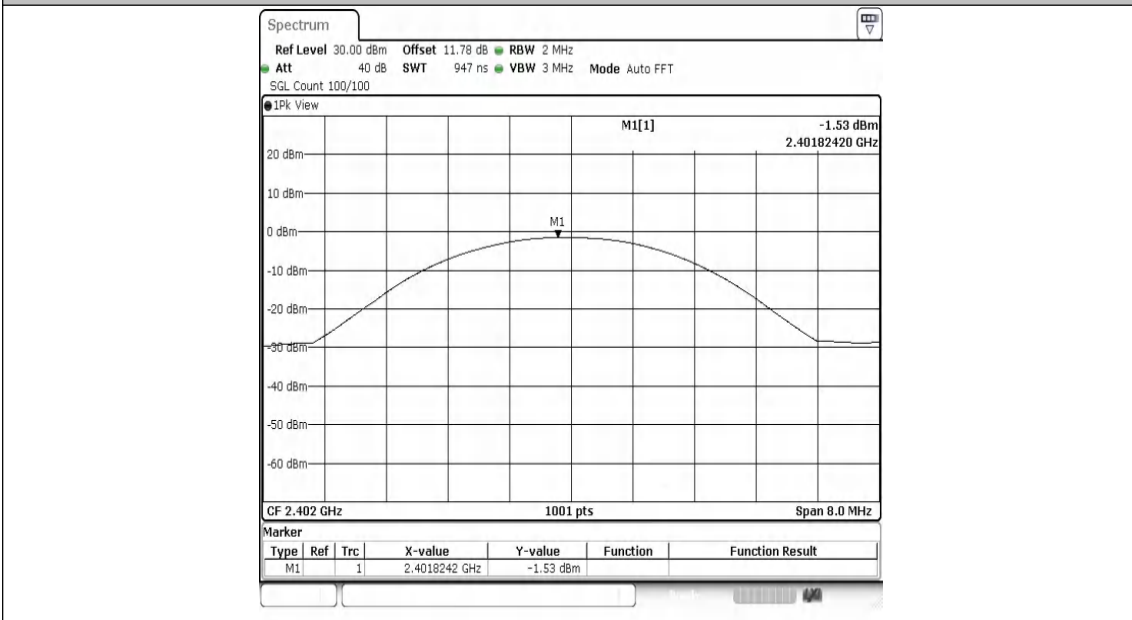
2DH5-Ant1-2402-PASS
