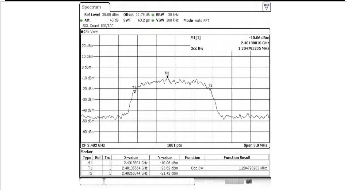
3DH5-Ant1-2402
