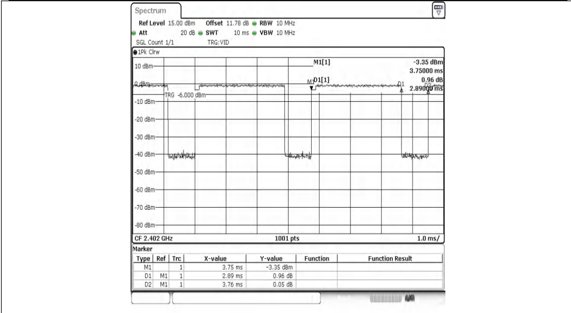
NTNV-3DH5-Ant1-2402
