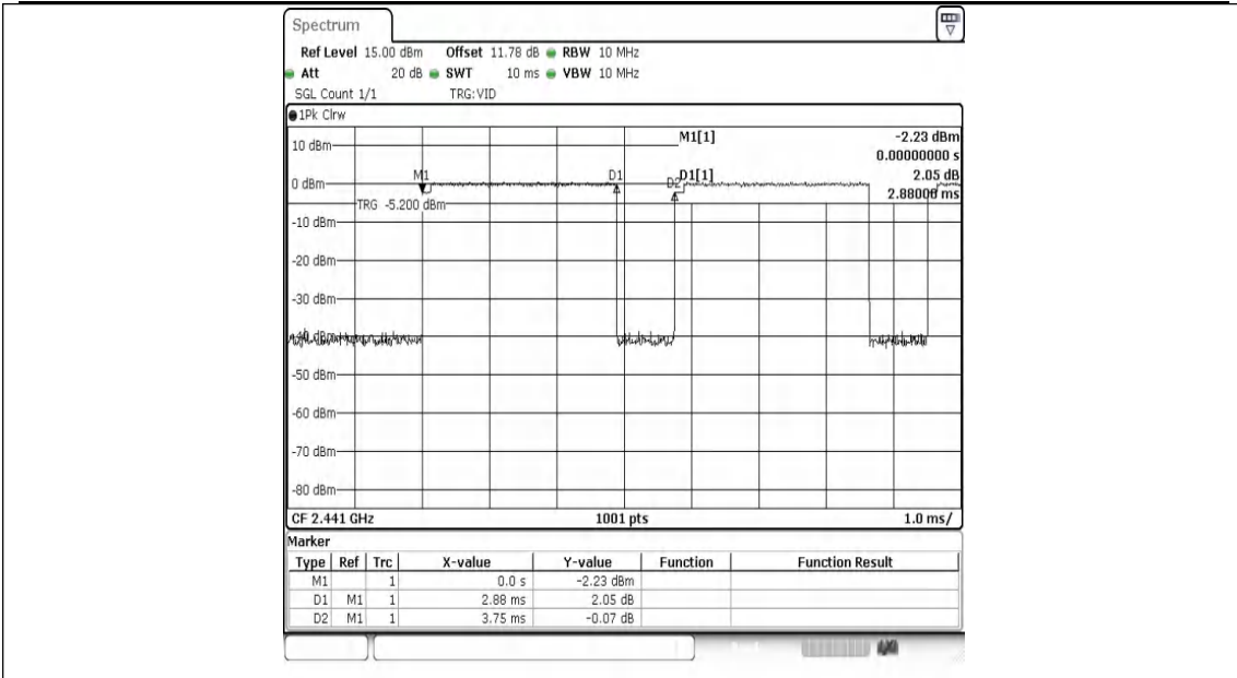
NTNV-2DH5-Ant1-2441
