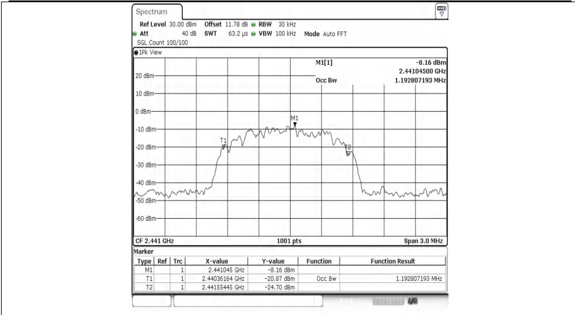
2DH5-Ant1-2441
