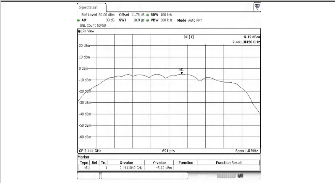
3DH5-Ant1-2441-0~Reference-PASS
