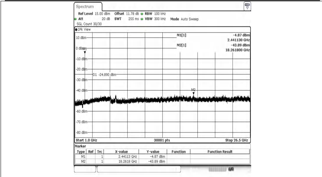
2DH5-Ant1-2441-1000~26500-PASS
