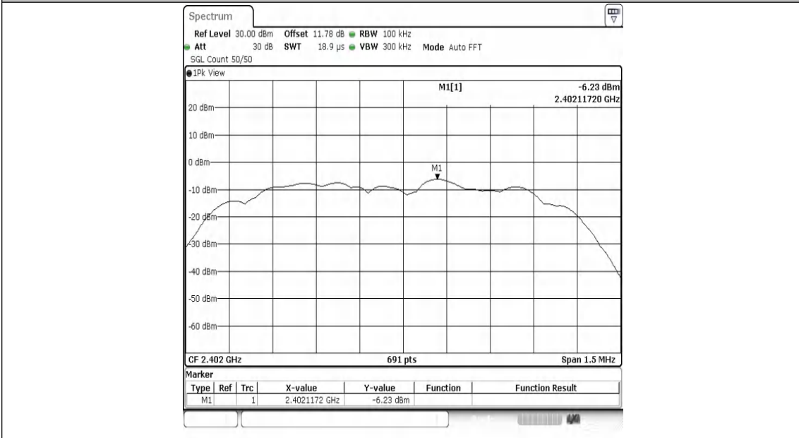
2DH5-Ant1-2402-0~Reference-PASS
