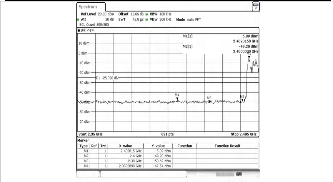
2DH5-Ant1-Hop_2402-PASS
