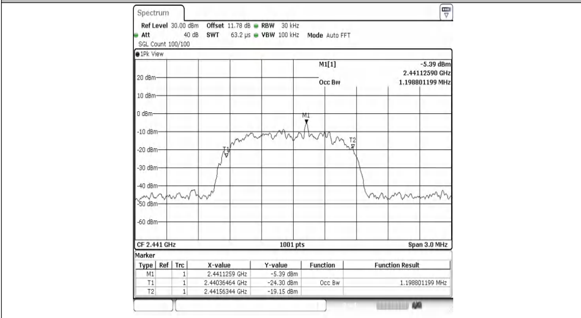
3DH5-Ant1-2441
