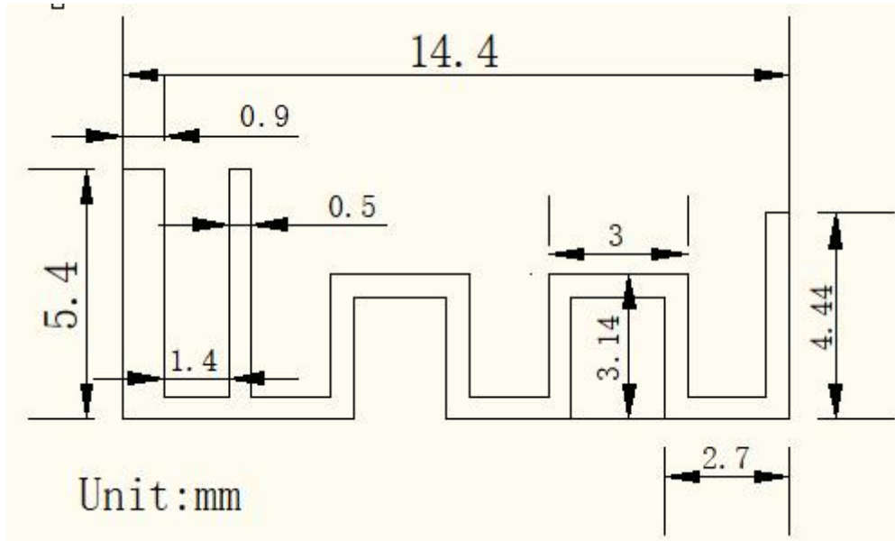
Size of antenna
