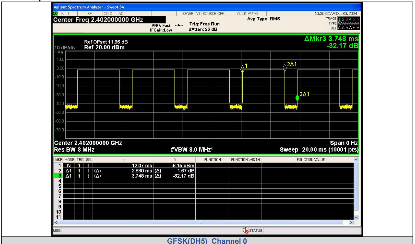
GFSK(DH5)_Channel 0
