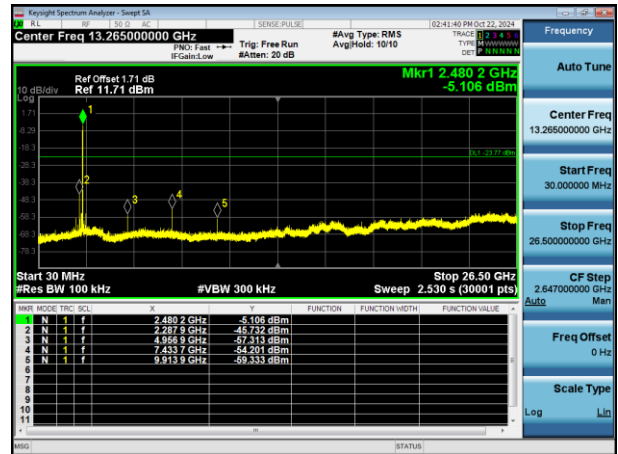
Spurious Emissions
