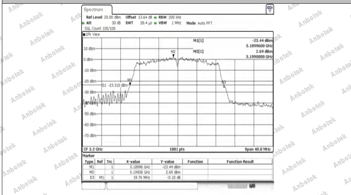
11N20SISO-Ant1-5200
