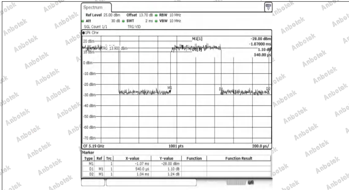
NTVN-11AX40SISO-Ant1-5190
