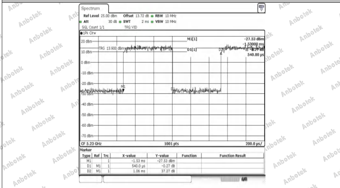
NTVN-11AX40SISO-Ant1-5230
