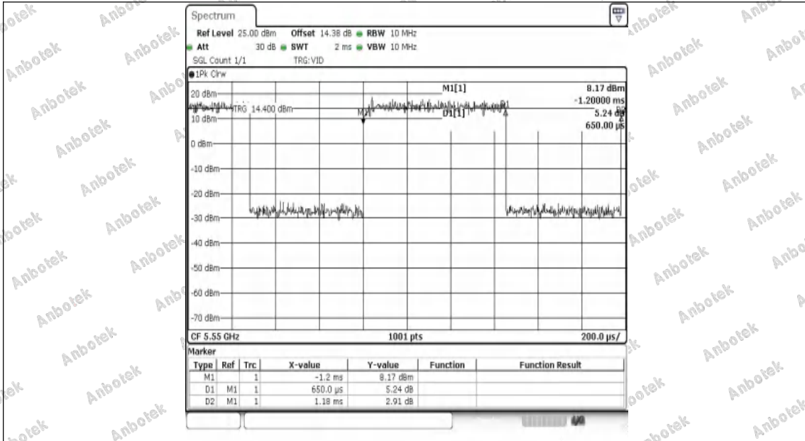
NTNV-11AC40SISO-Ant1-5550
