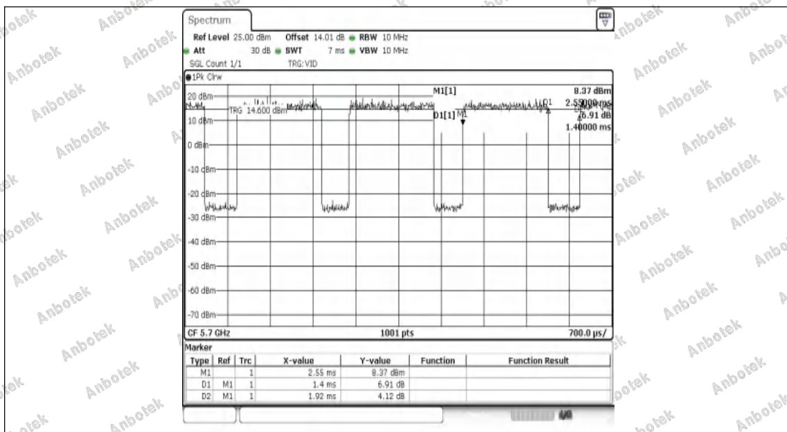
NTVN-11A-Ant1-5700
