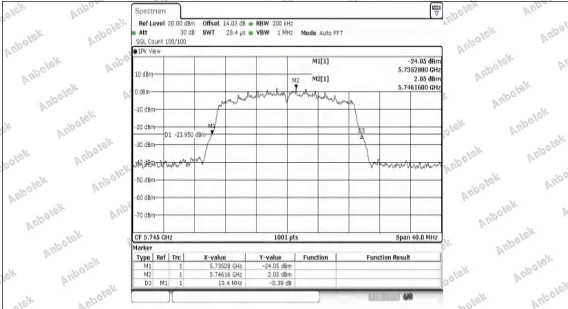
11AC20SISO-Ant1-5745
