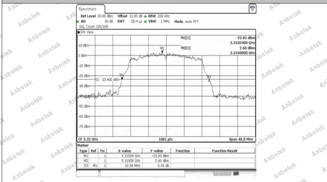
11A-Ant1-5320
