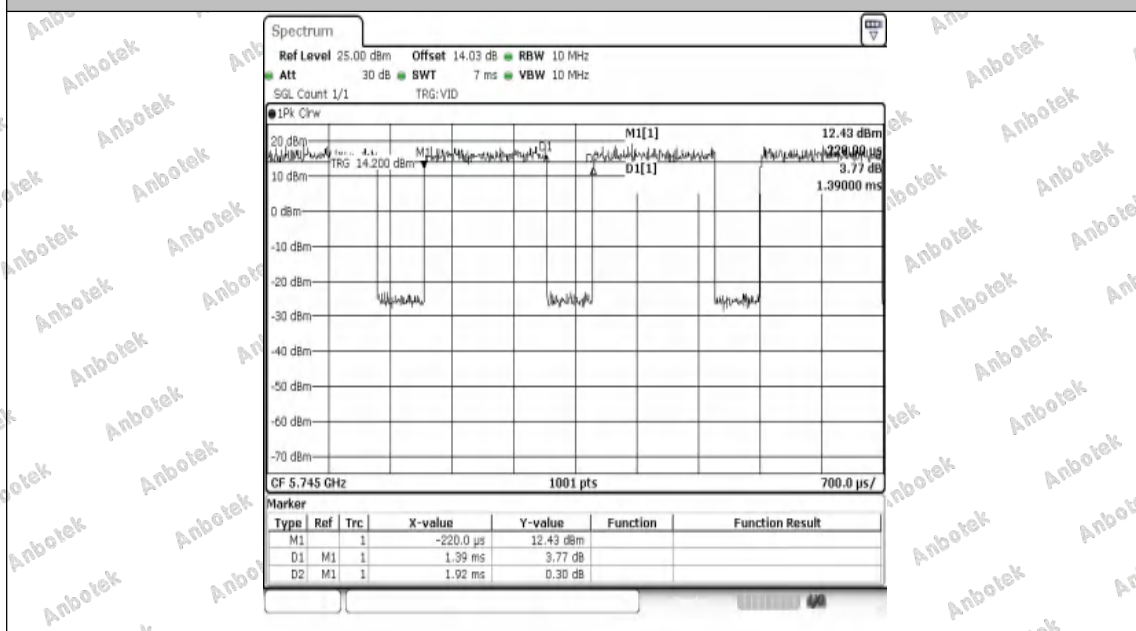
NTVN-11A-Ant1-5745
