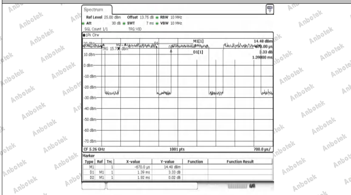
NTVN-11A-Ant1-5260
