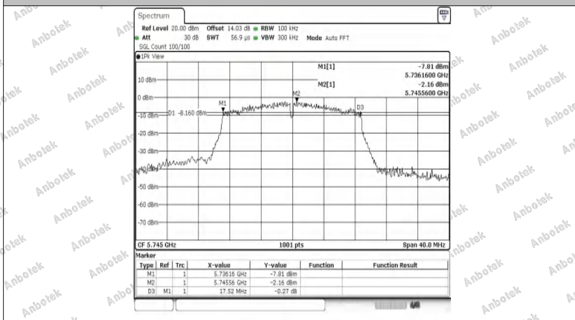
11N20SISO-Ant1-5745-PASS
