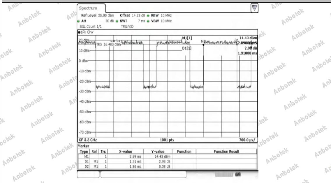
NTNV-11AC20SISO-Ant1-5500
