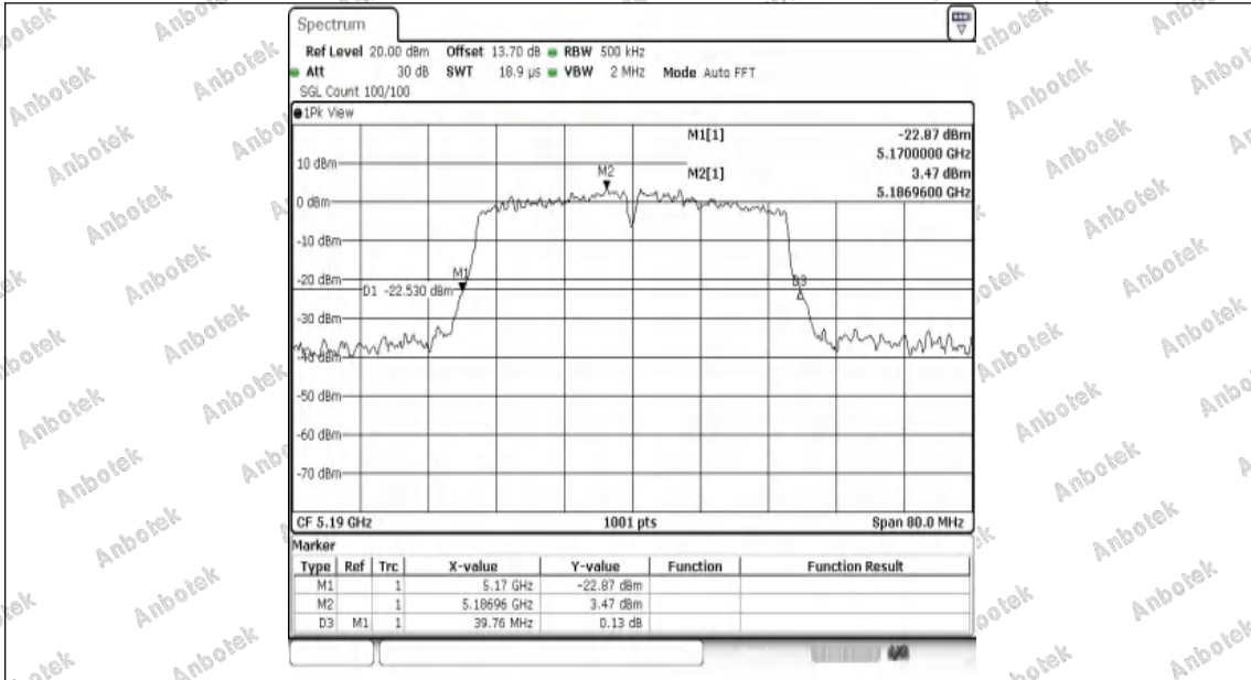
11N40SISO-Ant1-5190
