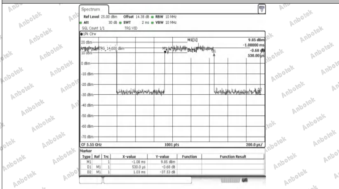
NTNV-11AX40SISO-Ant1-5550
