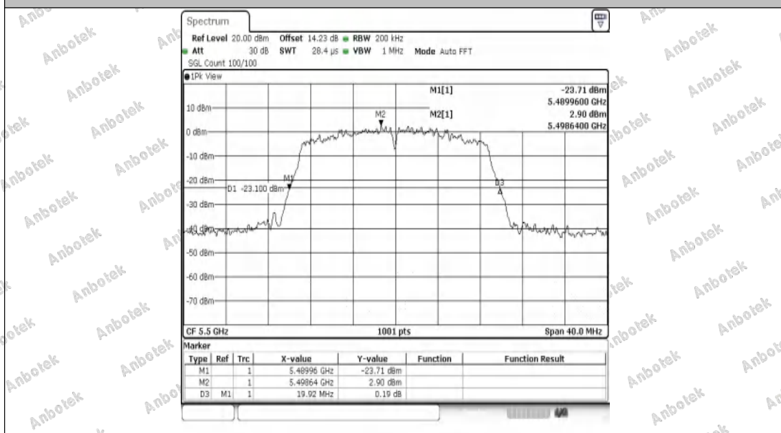
11AC20SISO-Ant1-5500
