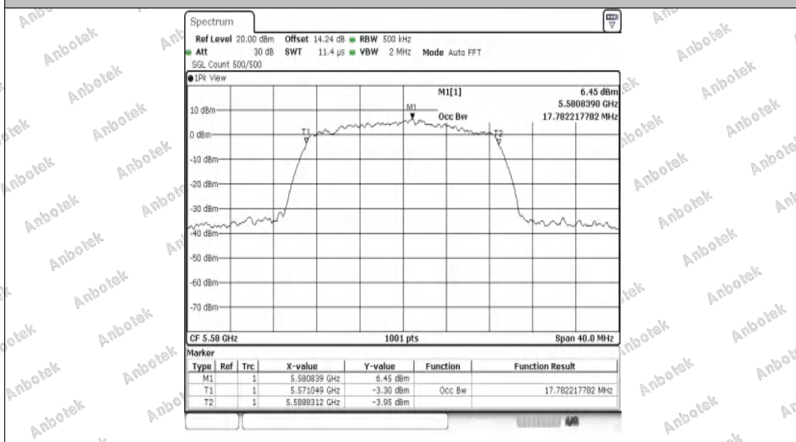
11N20SISO-Ant1-5580
