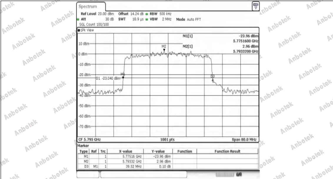
11AX40SISO-Ant1-5795
