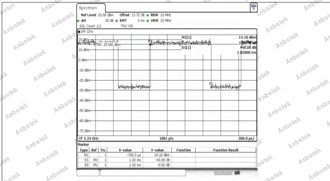
NTVN-11AX20SISO-Ant1-5240
