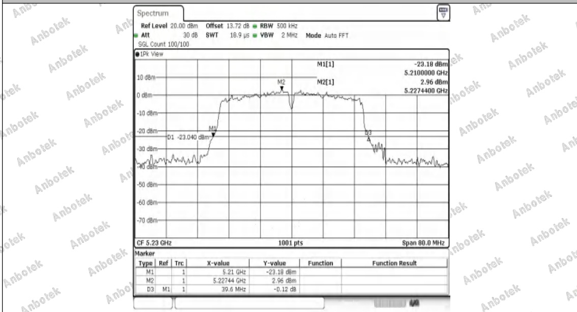
11N40SISO-Ant1-5230
