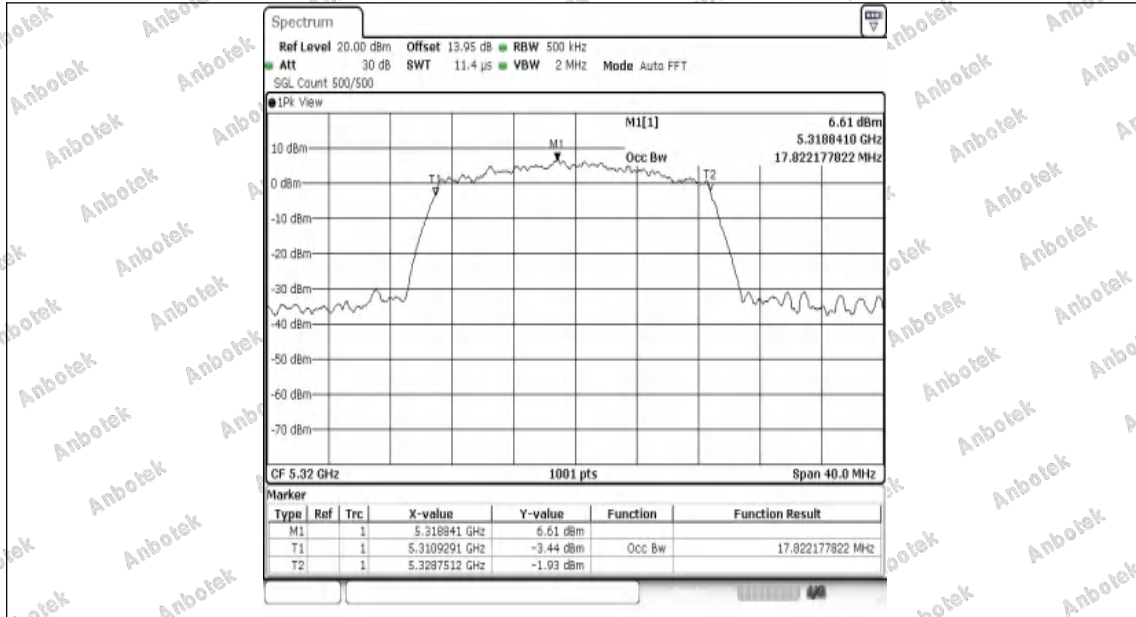
11AC20SISO-Ant1-5320
