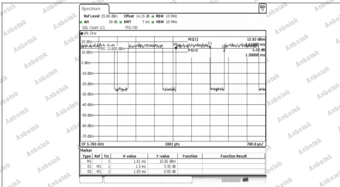
NTNV-11N20SISO-Ant1-5785
