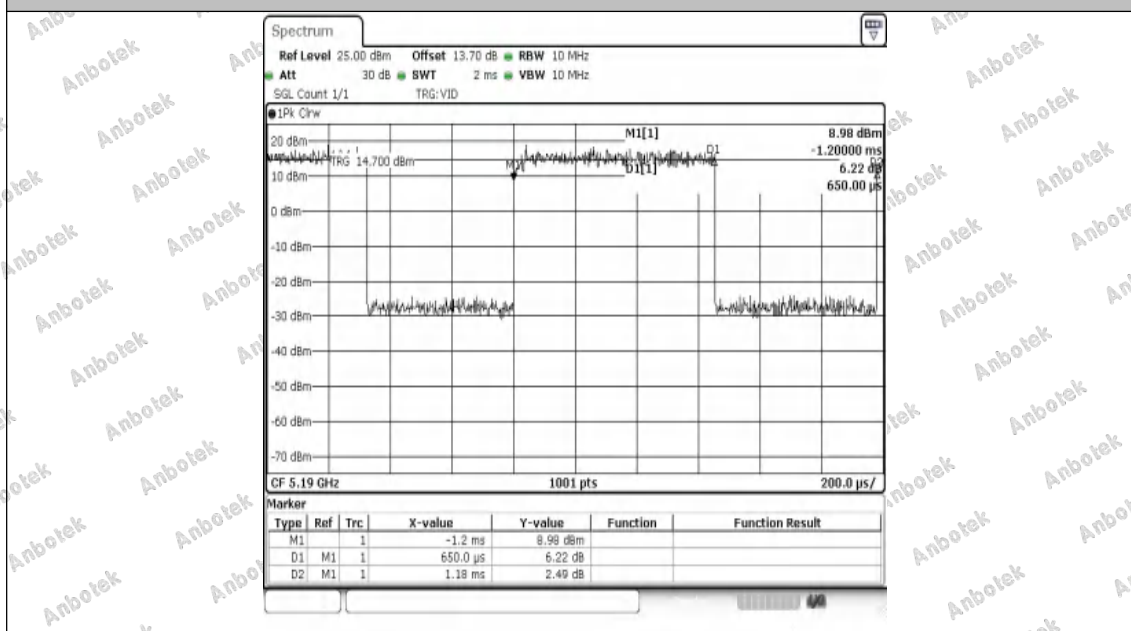
NTNV-11AC40SISO-Ant1-5190
