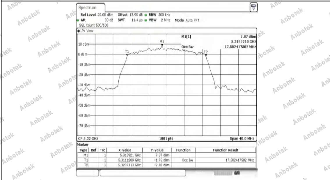
11N20SISO-Ant1-5320
