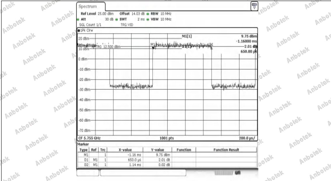
NTNV-11AC40SISO-Ant1-5755
