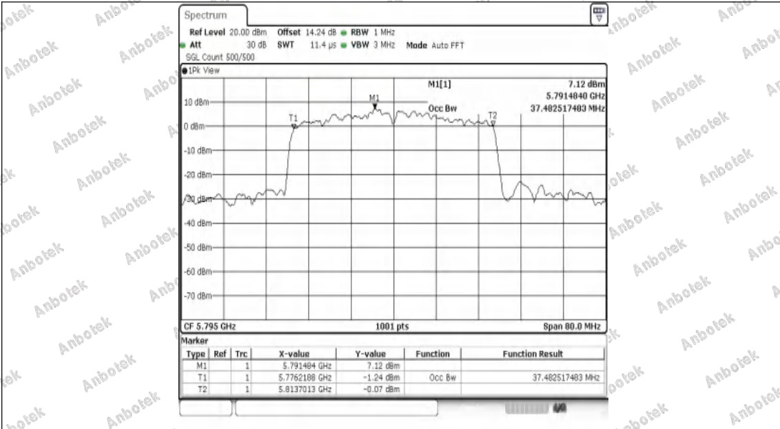
11AX40SISO-Ant1-5795
