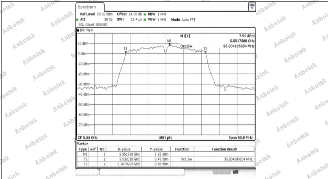
11AC40SISO-Ant1-5550
