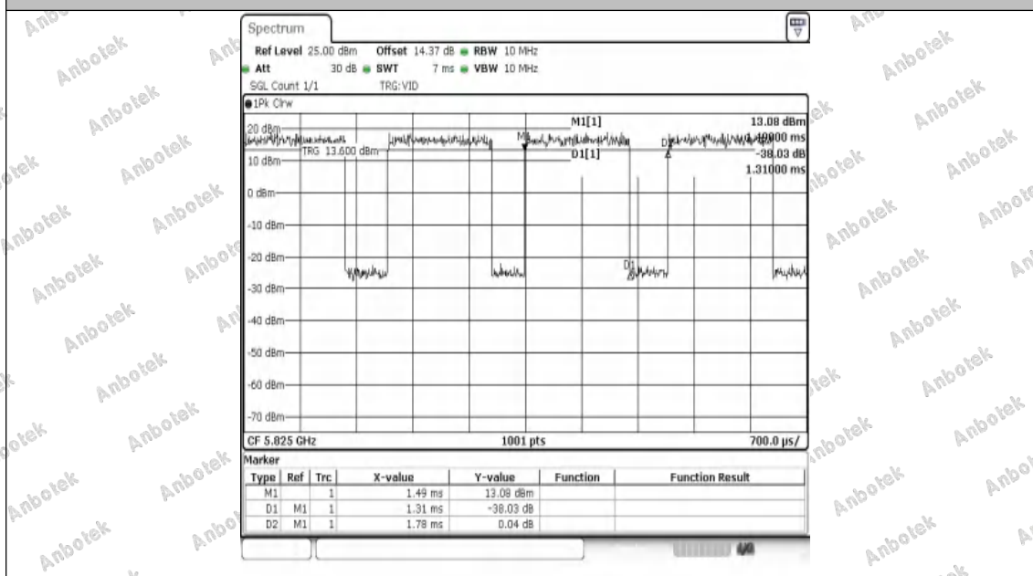
NTNV-11N20SISO-Ant1-5825
