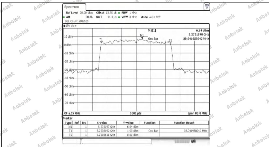
11AX40SISO-Ant1-5270
