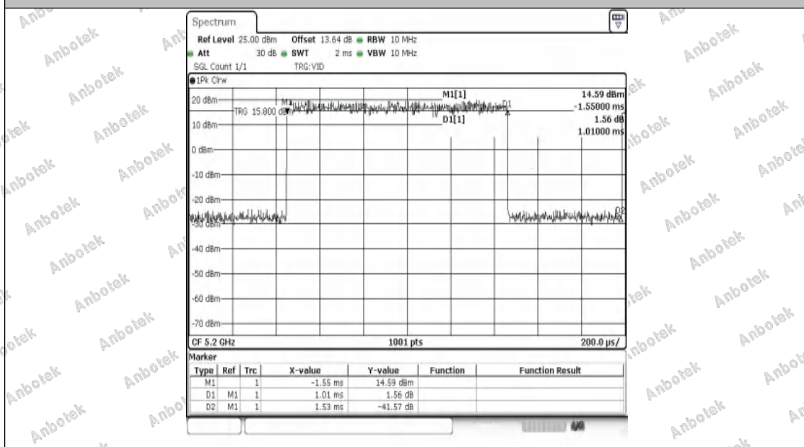
NTNV-11AX20SISO-Ant1-5200
