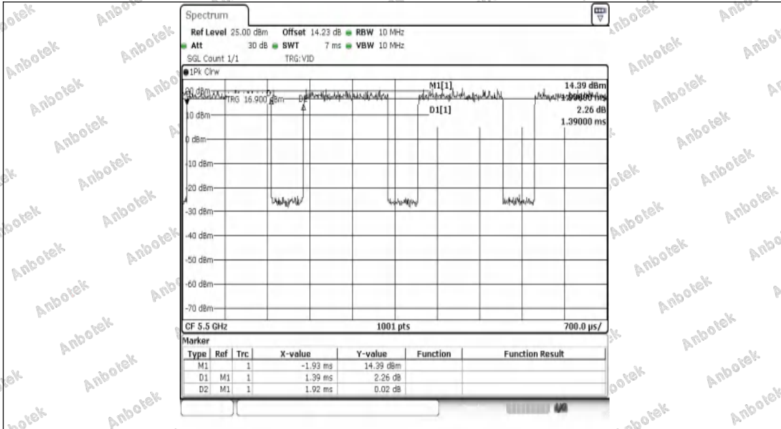
NTVN-11A-Ant1-5500
