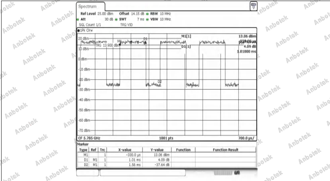
NTVN-11AX20SISO-Ant1-5785
