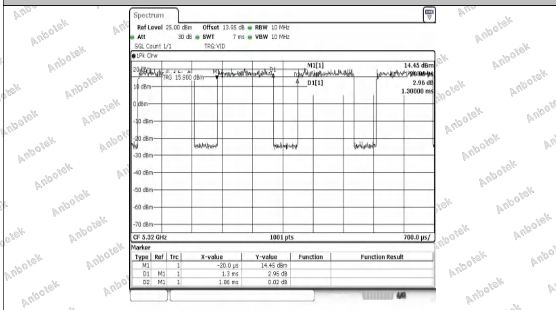
NTNV-11N20SISO-Ant1-5320
