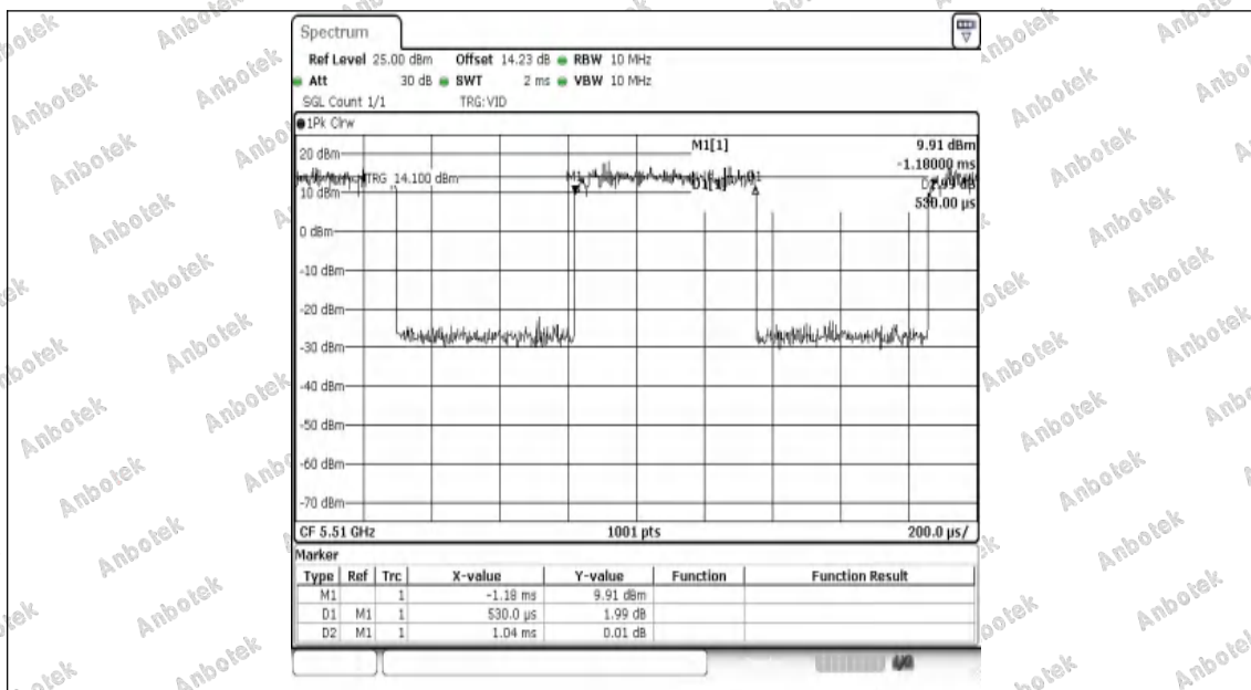
NTNV-11AX40SISO-Ant1-5510
