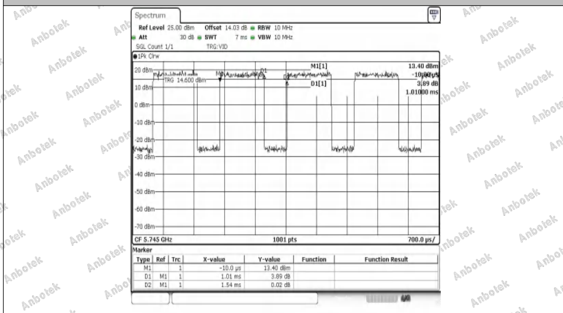
NTNV-11AX20SISO-Ant1-5745
