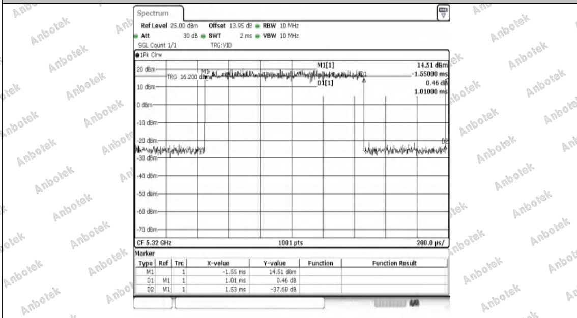
NTVN-11AX20SISO-Ant1-5320
