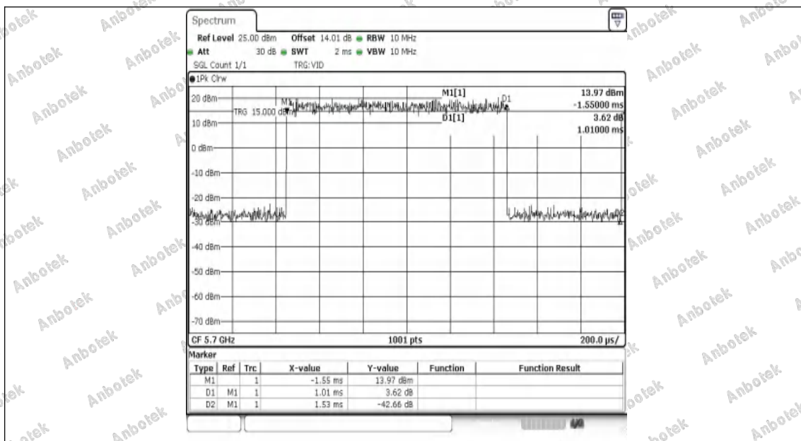
NTNV-11AX20SISO-Ant1-5700
