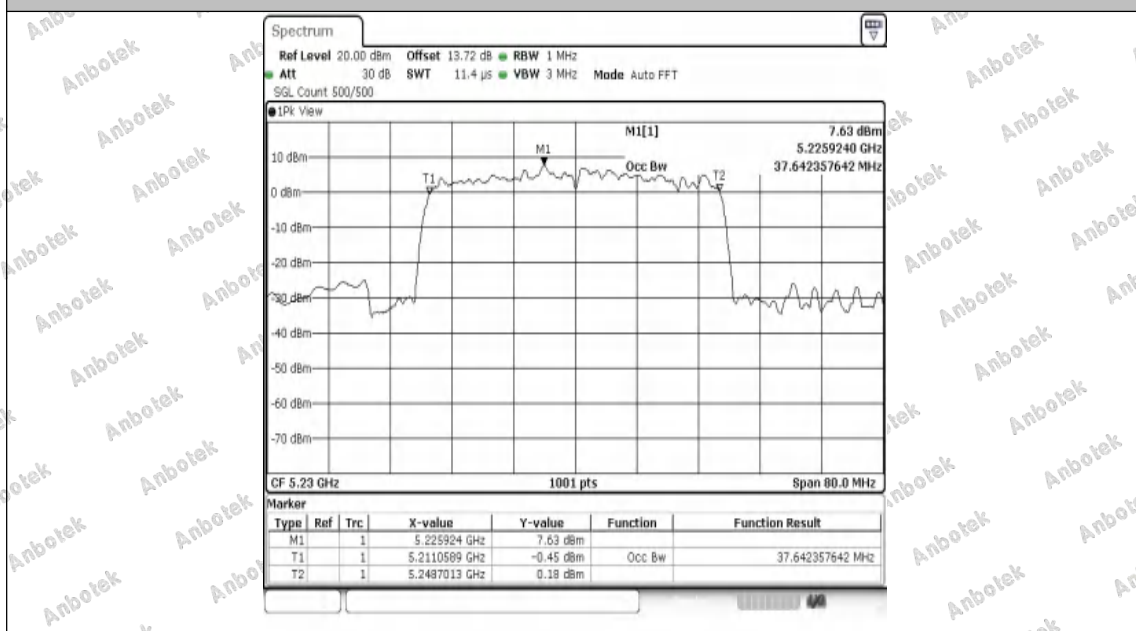
11AX40SISO-Ant1-5230
