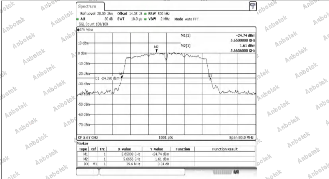
11N40SISO-Ant1-5670
