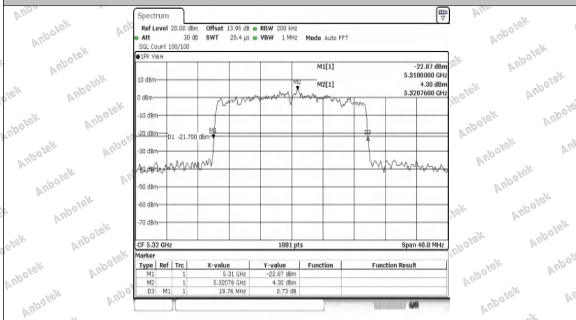
11AX20SISO-Ant1-5320
