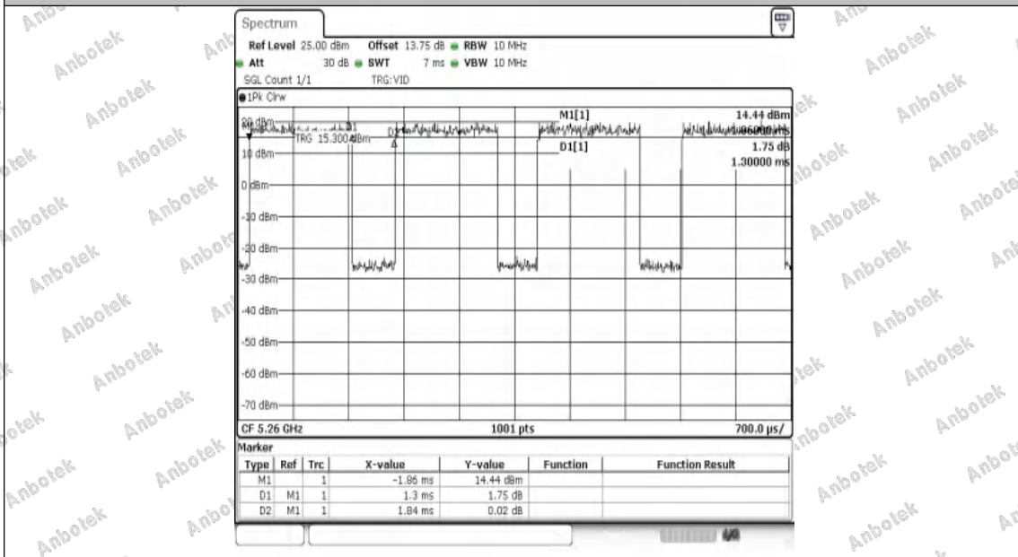
NTVN-11N20SISO-Ant1-5260
