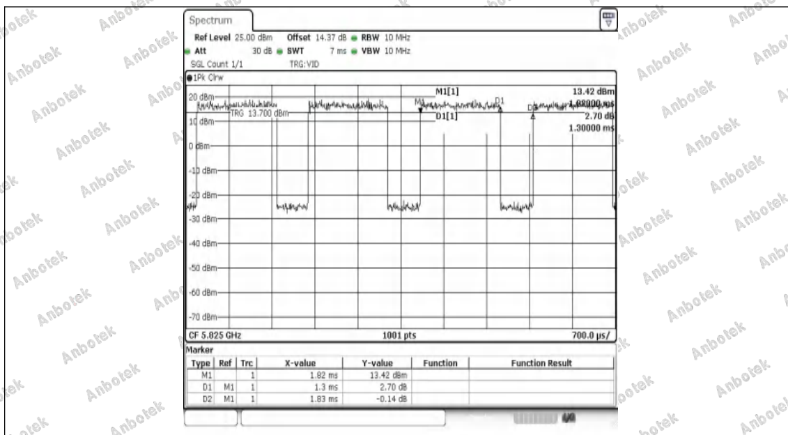
NTNV-11AC20SISO-Ant1-5825
