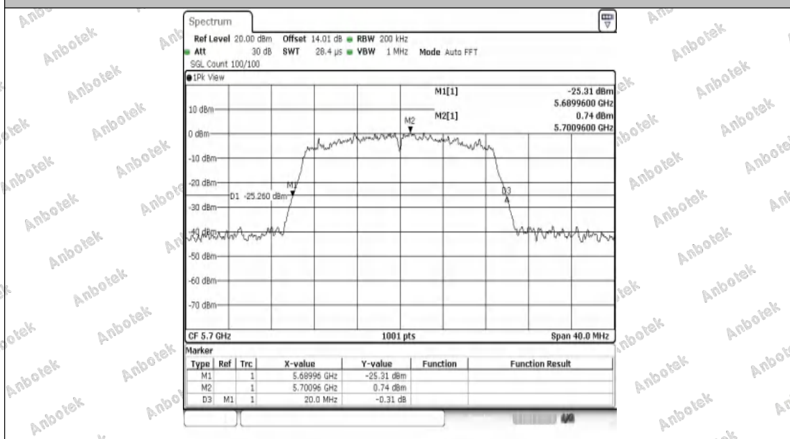
11AC20SISO-Ant1-5700
