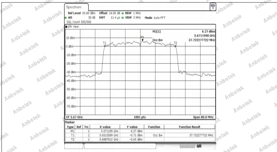
11AX40SISO-Ant1-5670
