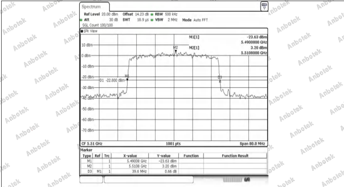
11AX40SISO-Ant1-5510
