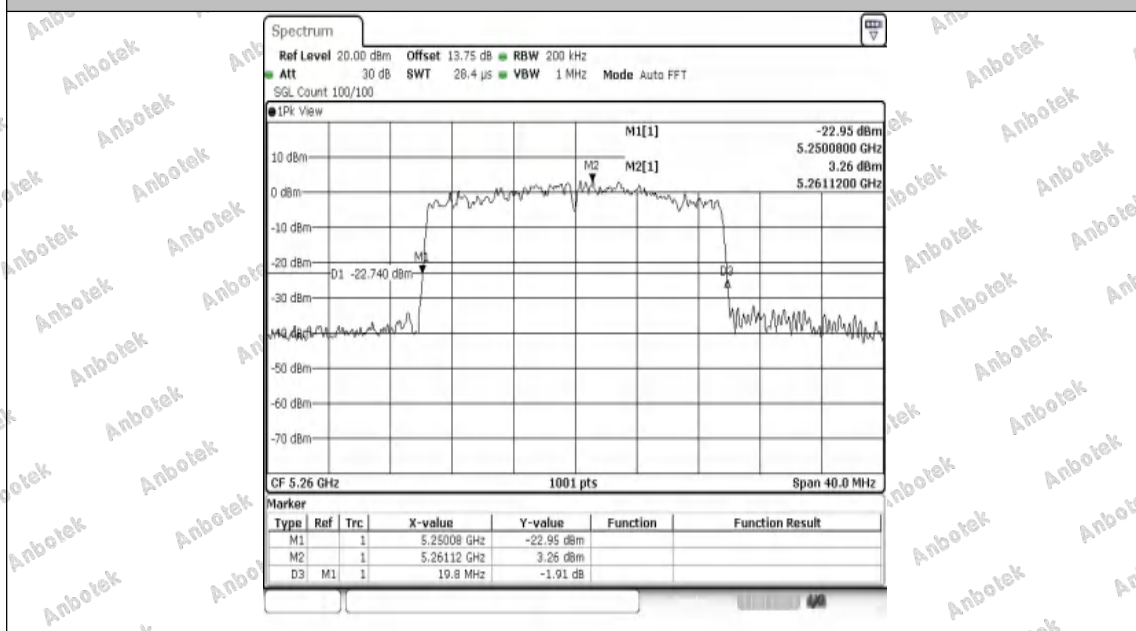
11AX20SISO-Ant1-5260
