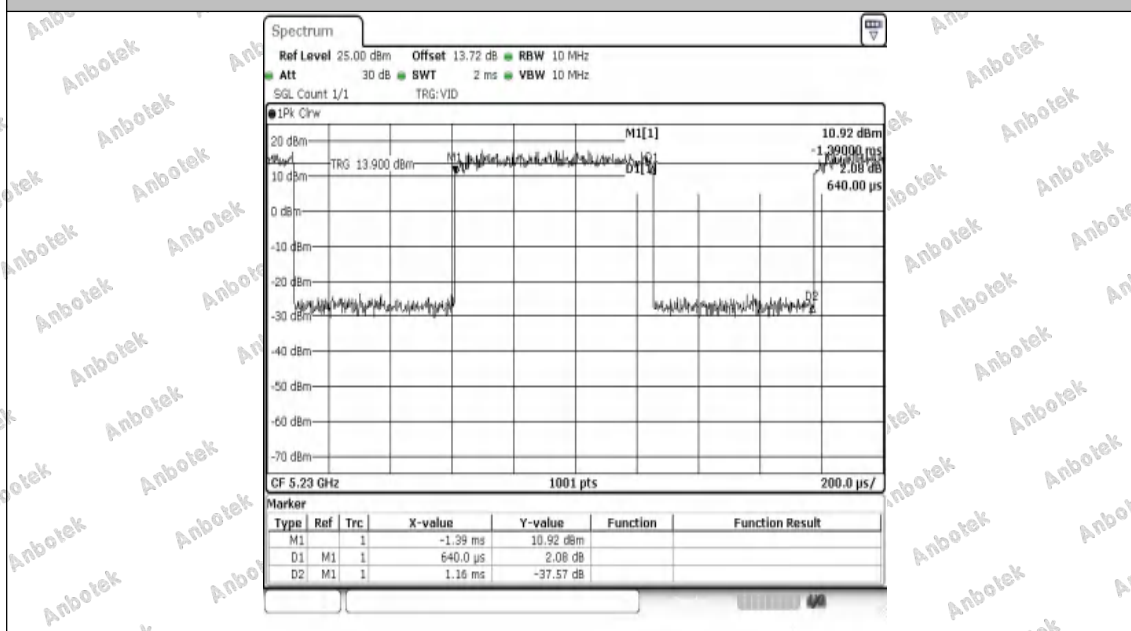
NTNV-11N40SISO-Ant1-5230
