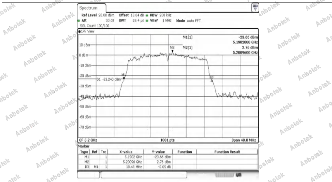
11AC20SISO-Ant1-5200
