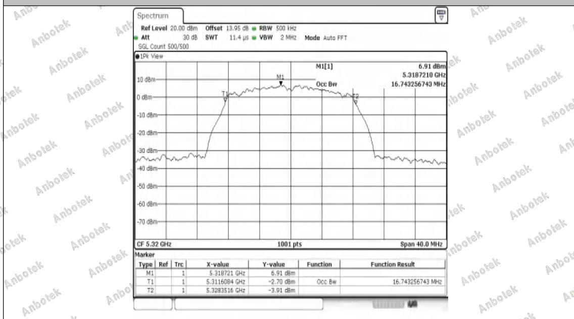
11A-Ant1-5320
