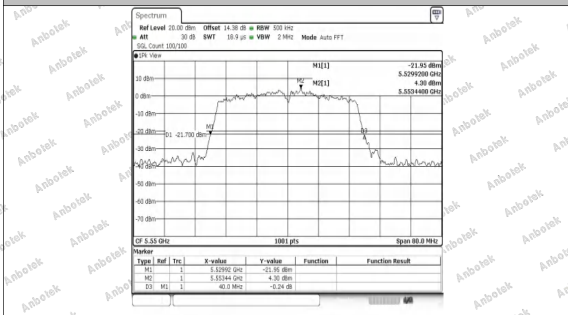
11N40SISO-Ant1-5550
