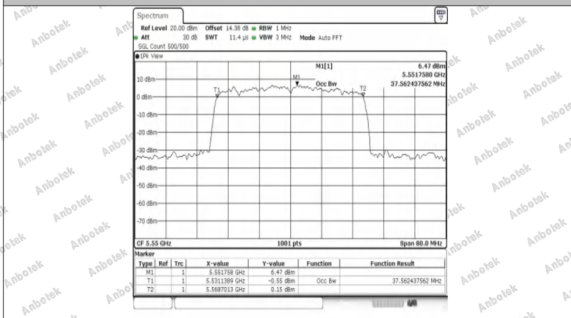
11AX40SISO-Ant1-5550
