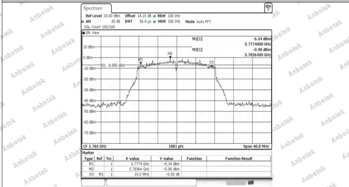
11A-Ant1-5785-PASS
