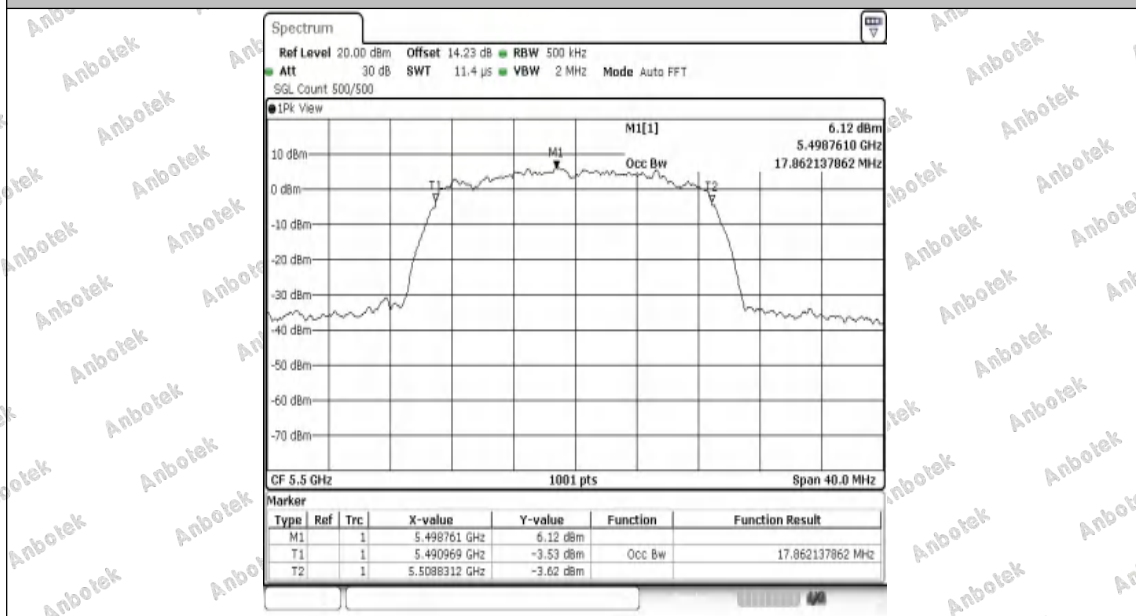
11AC20SISO-Ant1-5500
