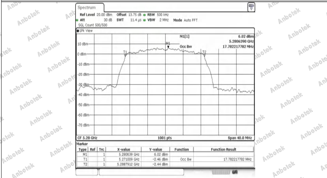
11AC20SISO-Ant1-5280
