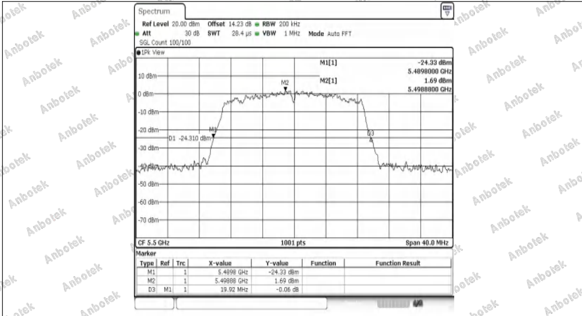
11N20SISO-Ant1-5500
