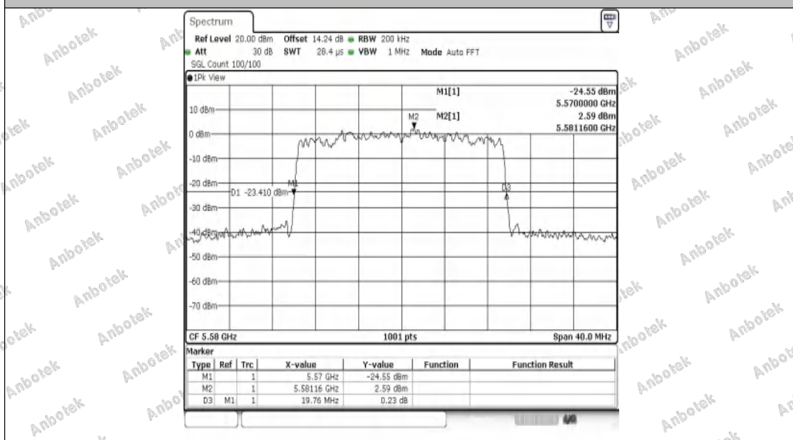
11AX20SISO-Ant1-5580
