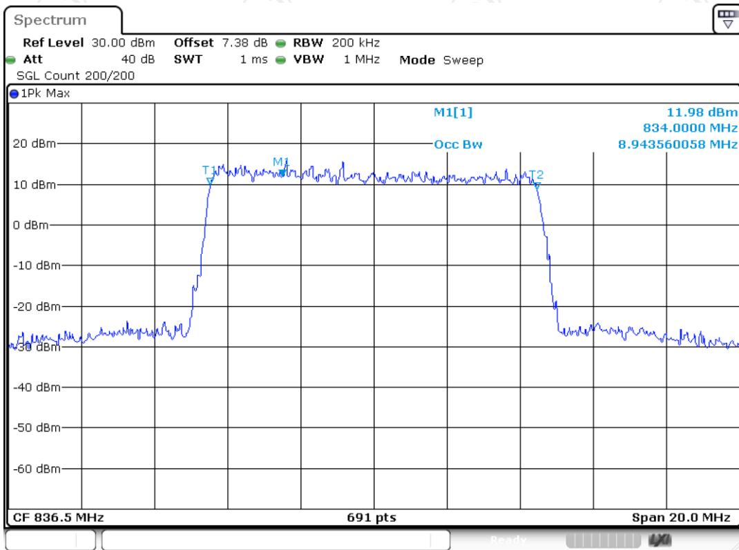
Band5 QAM16 BW=10MHz Channel=20525 RB Size=50 Position=#0
