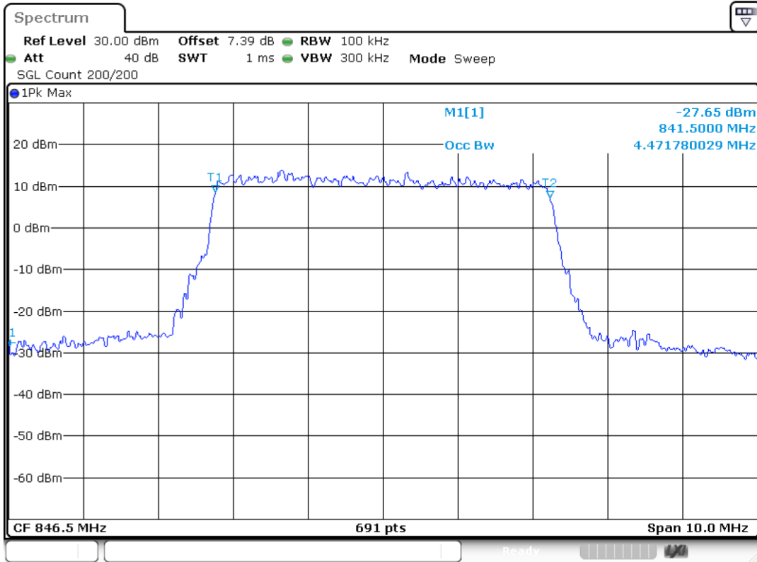
Band5 QAM16 BW=5MHz Channel=20625 RB Size=25 Position=#0
