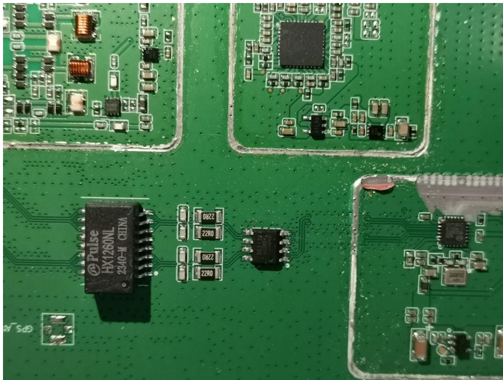
INTERNAL VIEW OF EUT (FIGURE 28)
