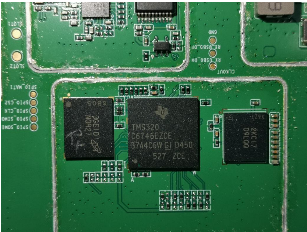
INTERNAL VIEW OF EUT (FIGURE 32)
