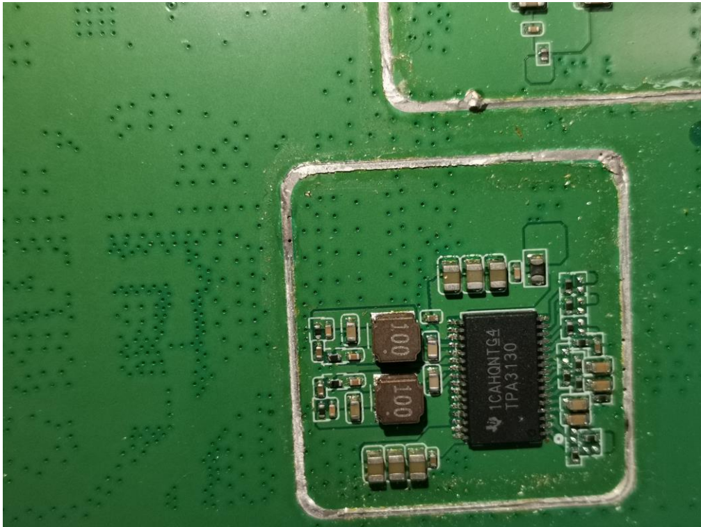
INTERNAL VIEW OF EUT (FIGURE 36)
