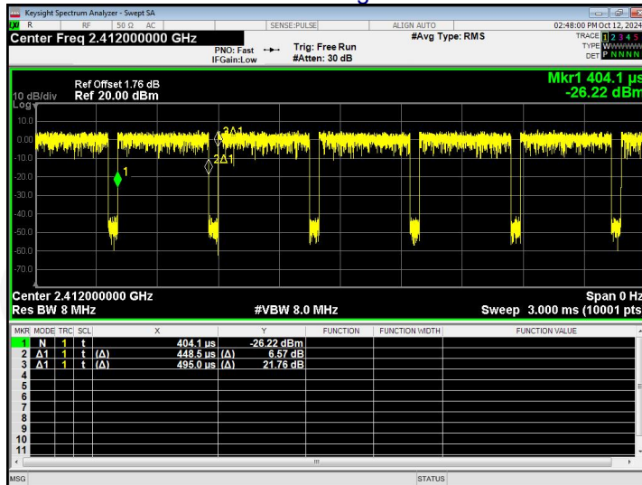
802.11g
