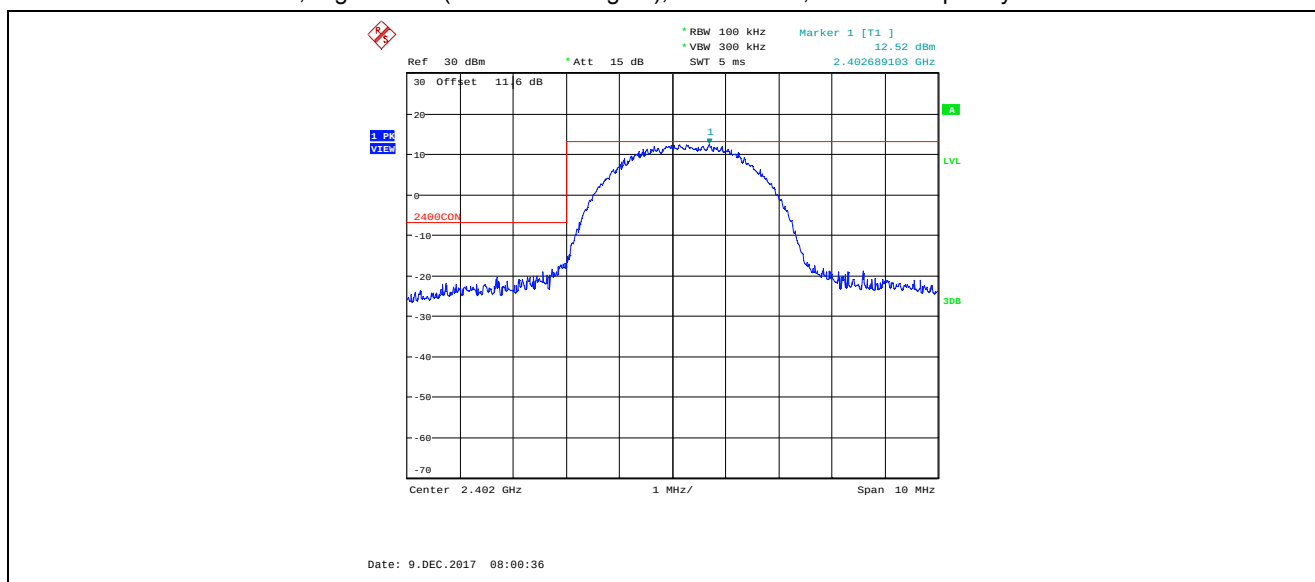
Plot 5.4.4.1.2. Band-Edge RF Conducted Emissions, Antenna 2 4 MHz Bandwidth, High Power (TX Gain Setting 22), Data Rate 3, Lowest Frequency Channel 2402 MHz
