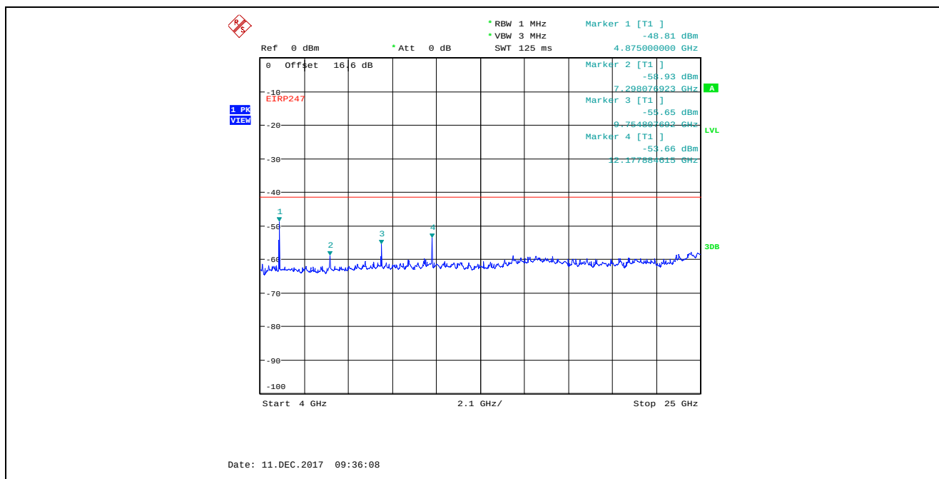
Plot 5.4.4.3.49. Conducted Spurious Emissions in Restricted Frequency Bands, Chain 1 8 MHz Bandwidth, TX Gain Setting 22, Data Rate 3, 2437 MHz, 4 GHz - 25 GHz, Peak Detector
