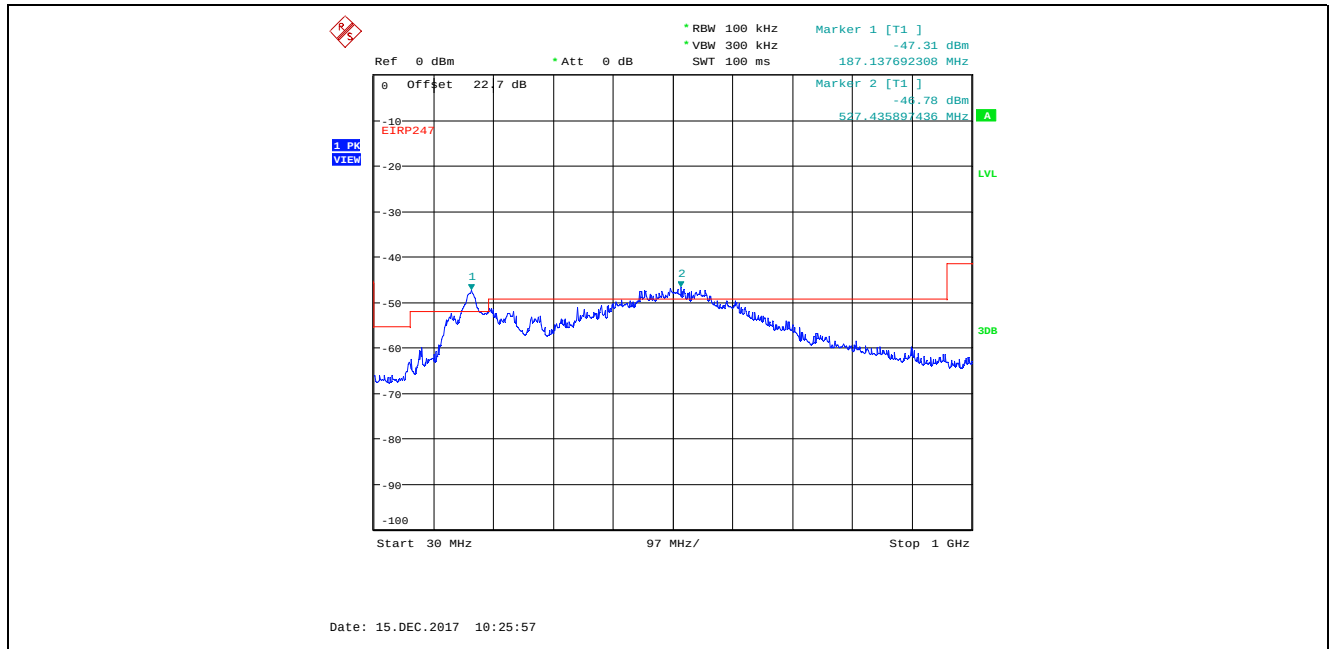
Plot 5.4.4.534. Conducted Spurious Emissions in Restricted Frequency Bands, Chain 1 4 MHz Bandwidth, TX Gain Setting 8, Data Rate 3, 2477 MHz, 30 MHz - 1 GHz, Peak Detector Emissions Above the Limit Line are Outside of the Restricted Bands
