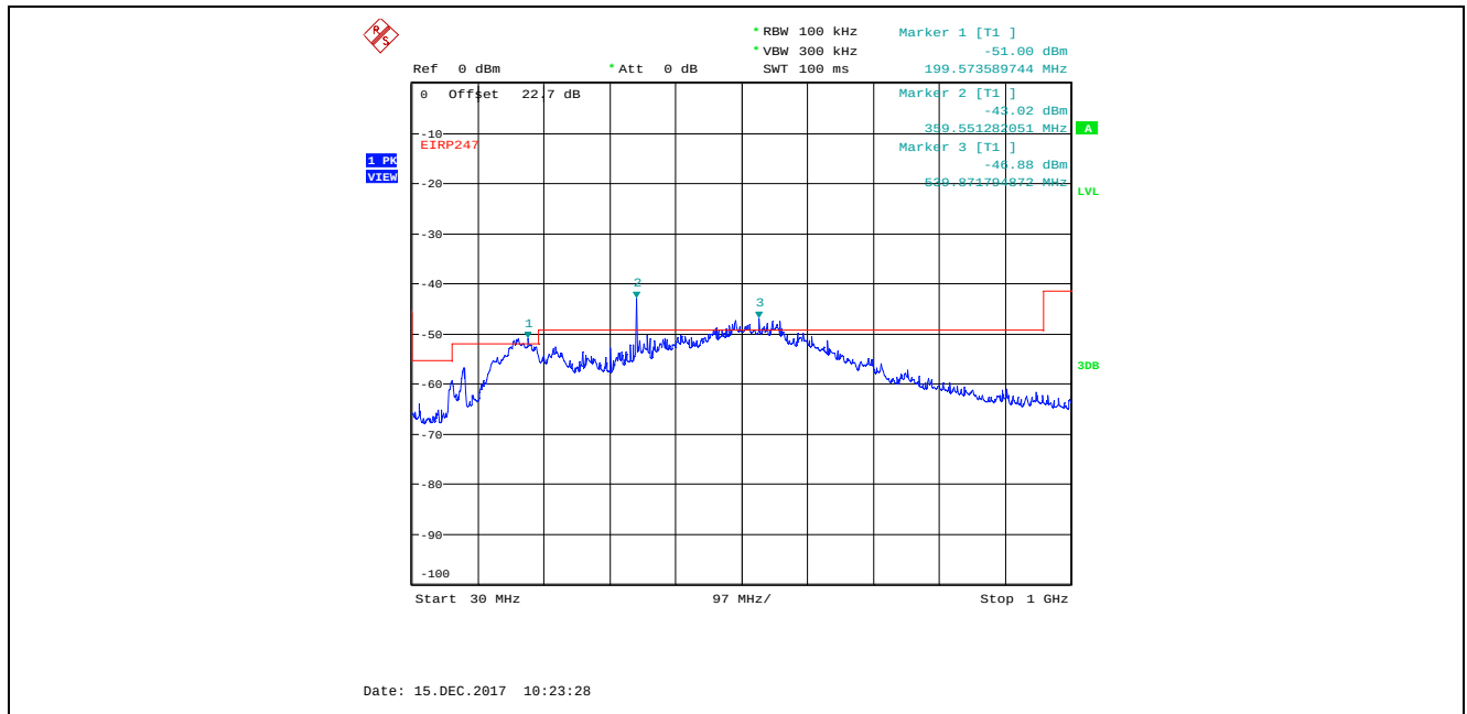
Plot 5.4.4.535. Conducted Spurious Emissions in Restricted Frequency Bands, Chain 2 4 MHz Bandwidth, TX Gain Setting 8, Data Rate 3, 2477 MHz, 30 MHz - 1 GHz, Peak Detector Emissions Above the Limit Line are Outside of the Restricted Bands
