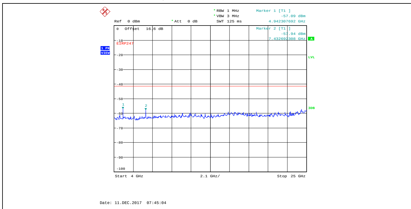
Plot 5.4.4.3.30. Conducted Spurious Emissions in Restricted Frequency Bands, Chain 2 4 MHz Bandwidth, TX Gain Setting 22, Data Rate 3, 2477 MHz, 4 GHz - 25 GHz, Peak Detector
