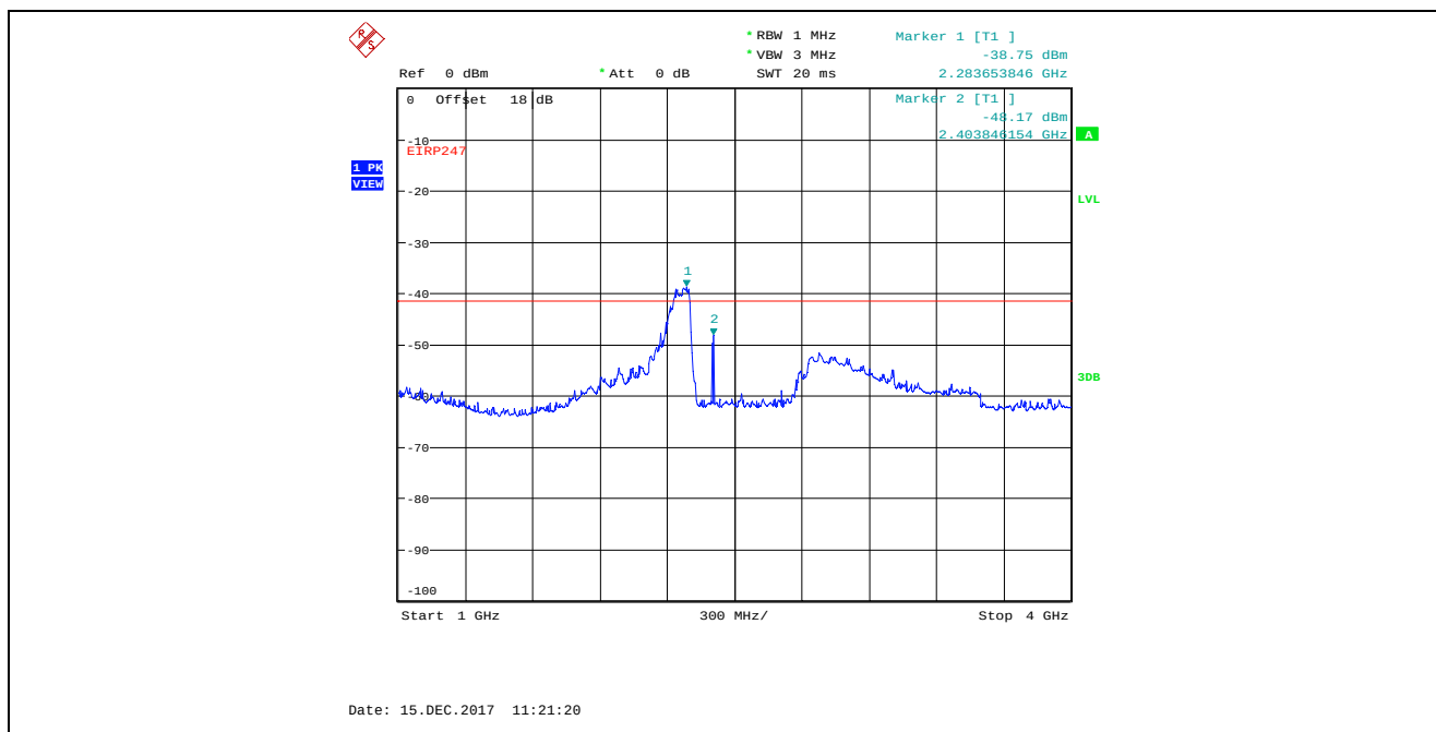
Plot 5.4.4.5.15. Conducted Spurious Emissions in Restricted Frequency Bands, Chain 2 4 MHz Bandwidth, TX Gain Setting 8, Data Rate 3, 2402 MHz, 1 GHz – 4 GHz, Peak Detector
