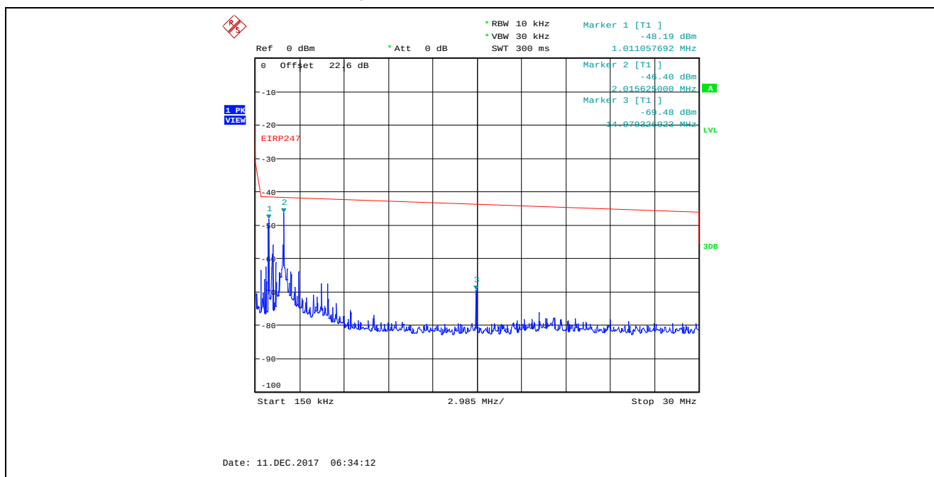
Plot 5.4.4.3.14. Conducted Spurious Emissions in Restricted Frequency Bands, Chain 2 4 MHz Bandwidth, TX Gain Setting 22, Data Rate 3, 2437 MHz, 150 kHz – 30 MHz, Peak Detector
