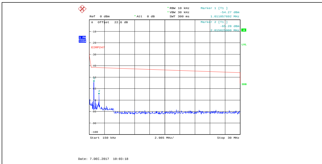
Plot 5.4.4.4.13. Conducted Spurious Emissions in Restricted Frequency Bands, Chain 1 4 MHz Bandwidth, TX Gain Setting 24, Data Rate 7, 2437 MHz, 150 kHz – 30 MHz, Peak Detector
