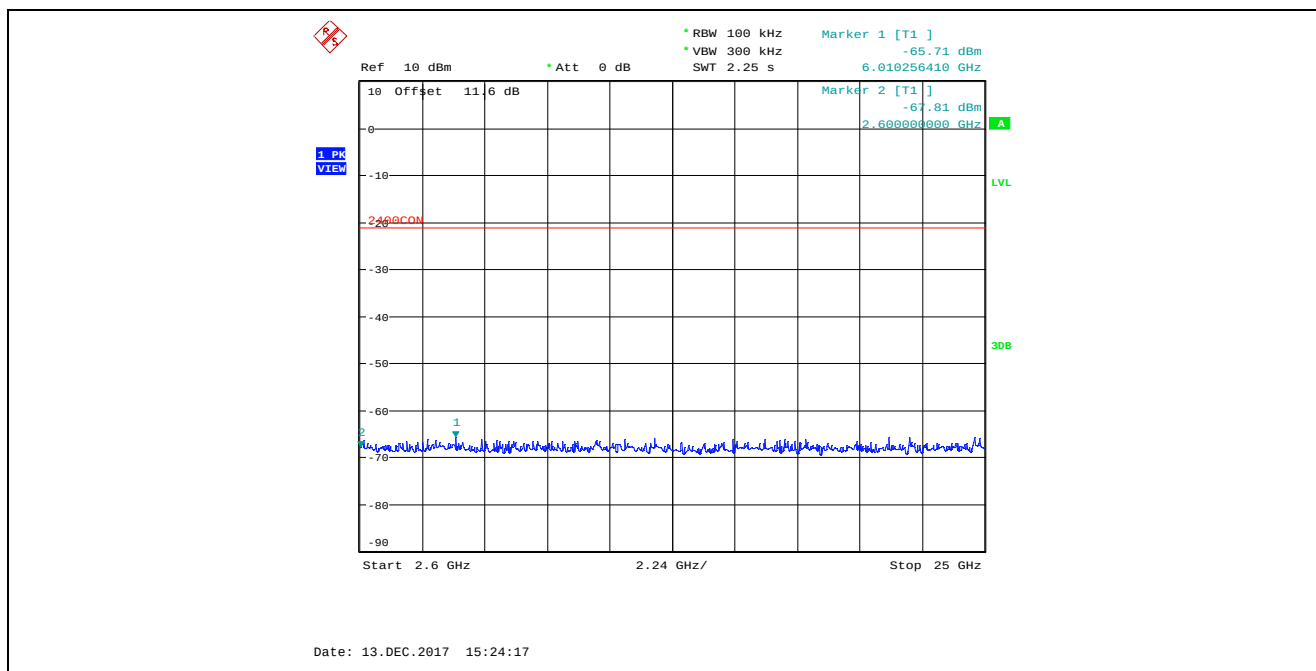
Plot 5.4.4.2.62. Conducted Spurious Emissions in Non-restricted Frequency Bands, Antenna 1 4 MHz Bandwidth, Low Power (TX Gain Setting 0), Data Rate 7, 2407 MHz, 2.6 GHz – 25 GHz
