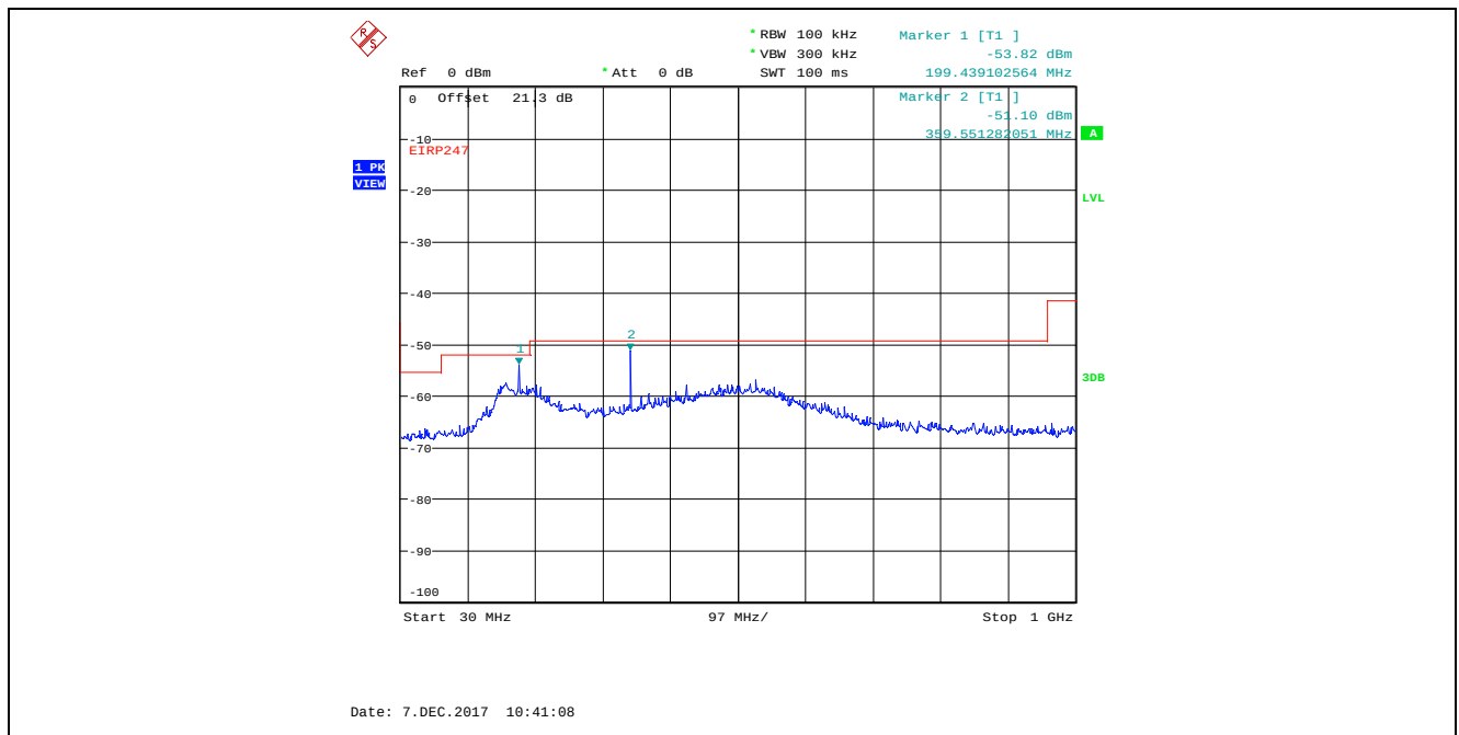
Plot 5.4.4.4.16. Conducted Spurious Emissions in Restricted Frequency Bands, Chain 2 4 MHz Bandwidth, TX Gain Setting 24, Data Rate 7, 2437 MHz, 30 MHz - 1 GHz, Peak Detector
