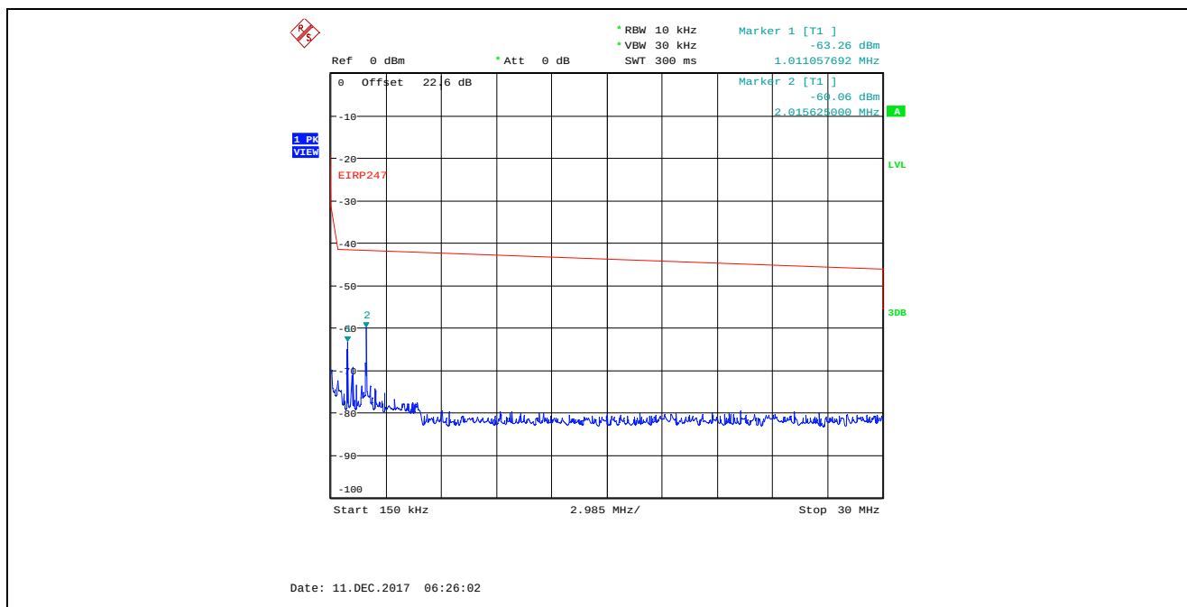
Plot 5.4.4.3.13. Conducted Spurious Emissions in Restricted Frequency Bands, Chain 1 4 MHz Bandwidth, TX Gain Setting 22, Data Rate 3, 2437 MHz, 150 kHz – 30 MHz, Peak Detector
