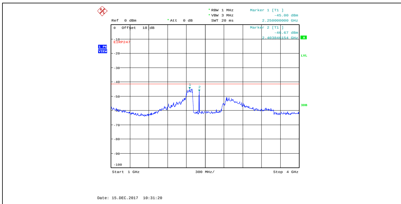
Plot 5.4.4.5.14. Conducted Spurious Emissions in Restricted Frequency Bands, Chain 1 4 MHz Bandwidth, TX Gain Setting 8, Data Rate 3, 2402 MHz, 1 GHz – 4 GHz, Peak Detector
