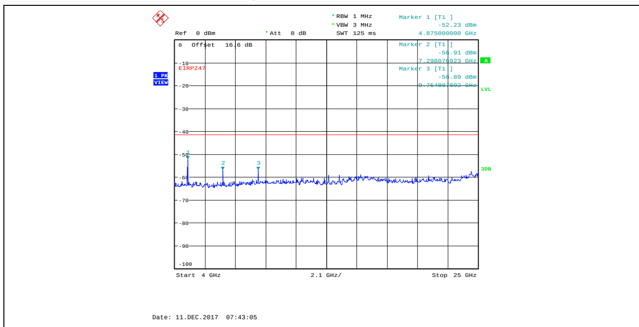
Plot 5.4.4.3.20. Conducted Spurious Emissions in Restricted Frequency Bands, Chain 2 4 MHz Bandwidth, TX Gain Setting 22, Data Rate 3, 2437 MHz, 4 GHz - 25 GHz, Peak Detector
