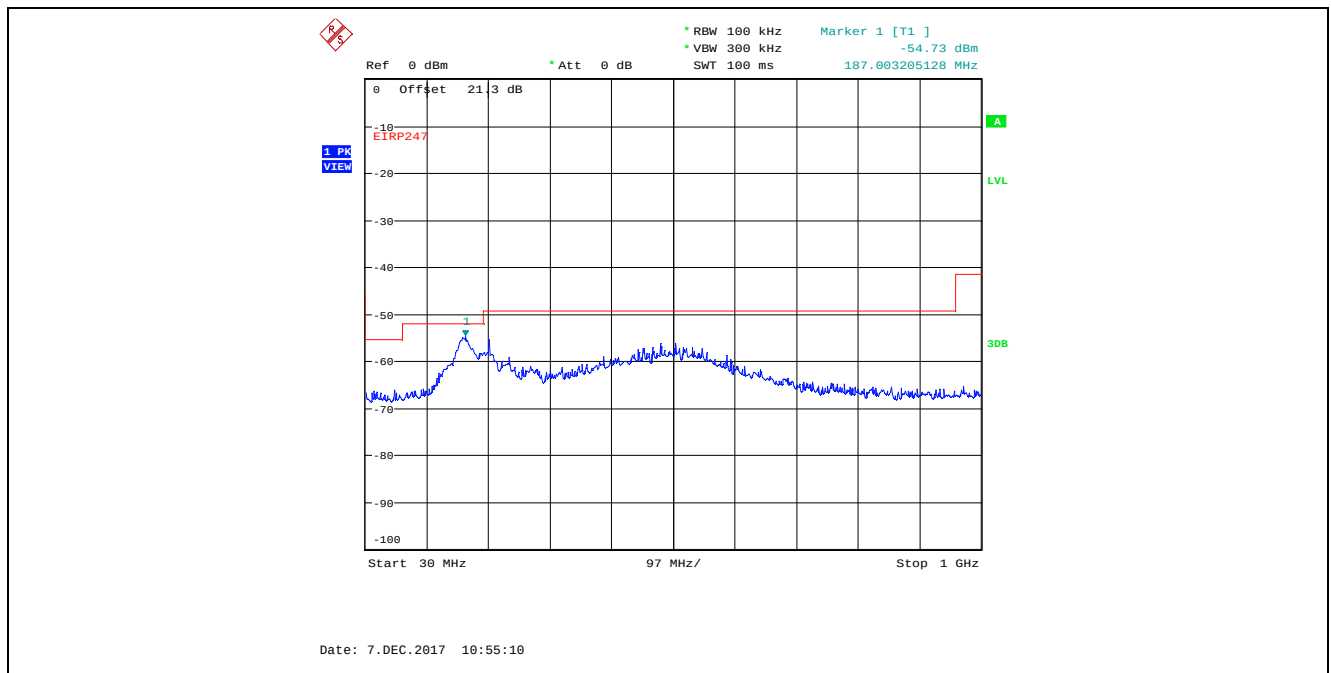
Plot 5.4.4.4.15. Conducted Spurious Emissions in Restricted Frequency Bands, Chain 1 4 MHz Bandwidth, TX Gain Setting 24, Data Rate 7, 2437 MHz, 30 MHz - 1 GHz, Peak Detector
