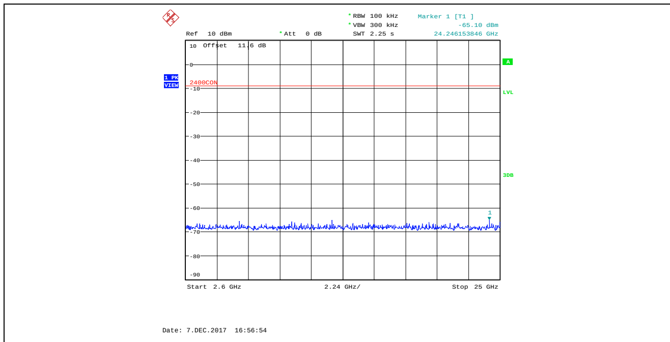
Plot 5.4.4.2.16. Conducted Spurious Emissions in Non-restricted Frequency Bands, Antenna 2 4 MHz Bandwidth, High Power (TX Gain Setting 24), Data Rate 7, 2407 MHz, 2.6 GHz – 25 GHz
