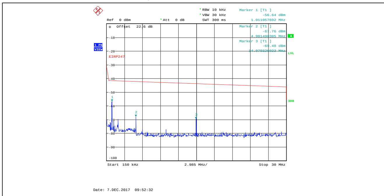
Plot 5.4.4.4.14. Conducted Spurious Emissions in Restricted Frequency Bands, Chain 2 4 MHz Bandwidth, TX Gain Setting 24, Data Rate 7, 2437 MHz, 150 kHz – 30 MHz, Peak Detector
