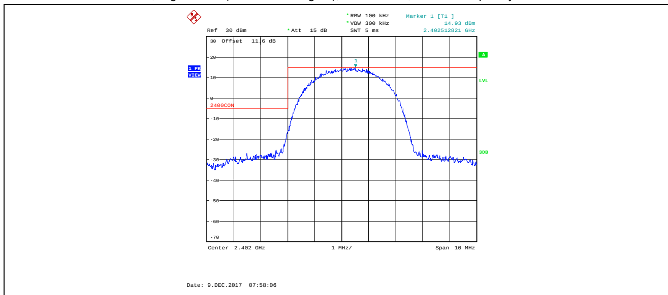
Plot 5.4.4.1.1. Band-Edge RF Conducted Emissions, Antenna 1 4 MHz Bandwidth, High Power (TX Gain Setting 22), Data Rate 3, Lowest Frequency Channel 2402 MHz
