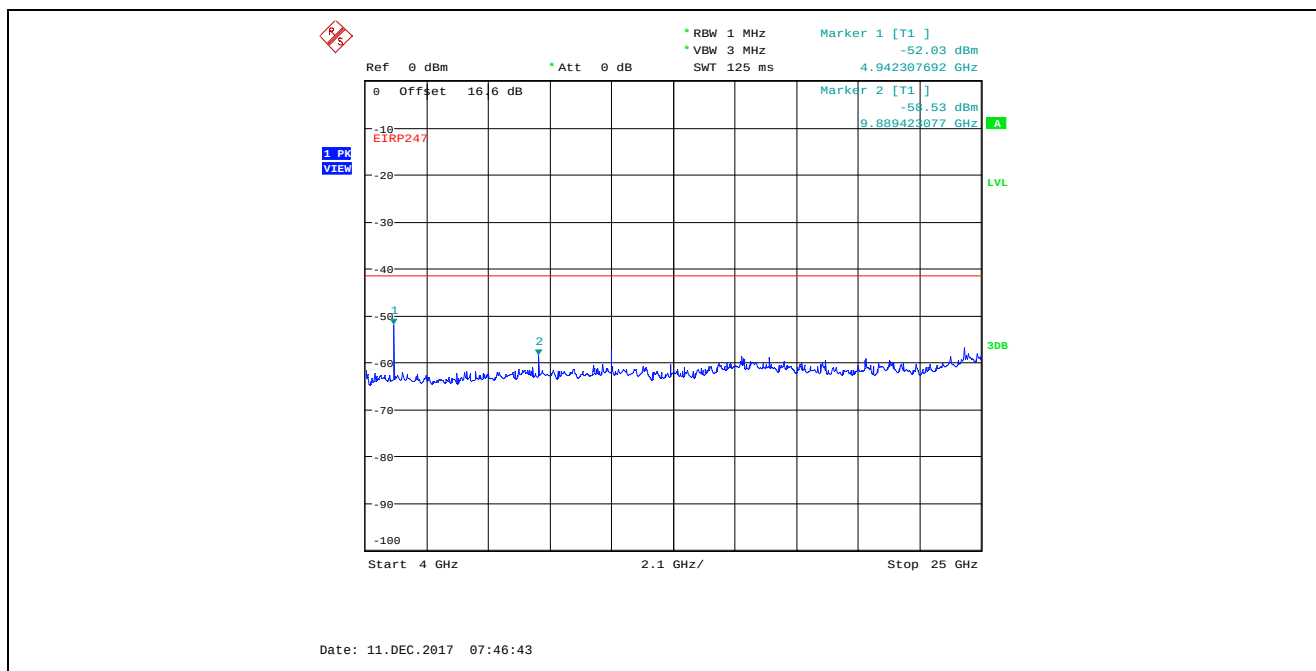
Plot 5.4.4.3.29. Conducted Spurious Emissions in Restricted Frequency Bands, Chain 1 4 MHz Bandwidth, TX Gain Setting 22, Data Rate 3, 2477 MHz, 4 GHz - 25 GHz, Peak Detector
