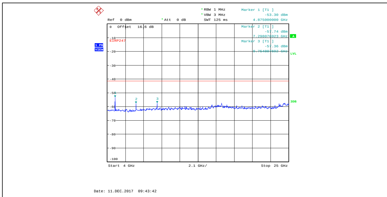
Plot 5.4.4.3.50. Conducted Spurious Emissions in Restricted Frequency Bands, Chain 2 8 MHz Bandwidth, TX Gain Setting 22, Data Rate 3, 2437 MHz, 4 GHz - 25 GHz, Peak Detector
