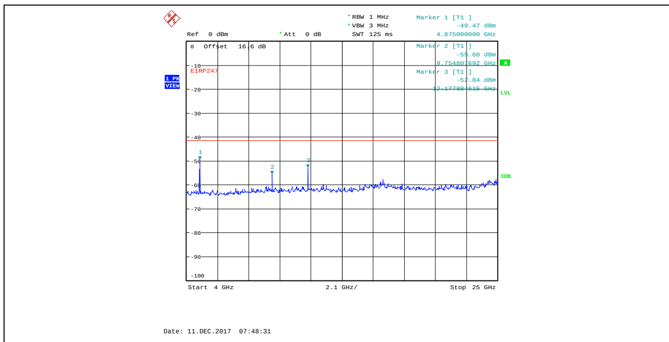
Plot 5.4.4.3.19. Conducted Spurious Emissions in Restricted Frequency Bands, Chain 1 4 MHz Bandwidth, TX Gain Setting 22, Data Rate 3, 2437 MHz, 4 GHz - 25 GHz, Peak Detector
