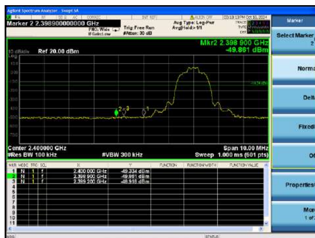
8-DPSK LOW CHANNEL, BAND EDGE
