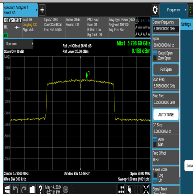
11AX40MIMO-Ant2-5795-PASS
