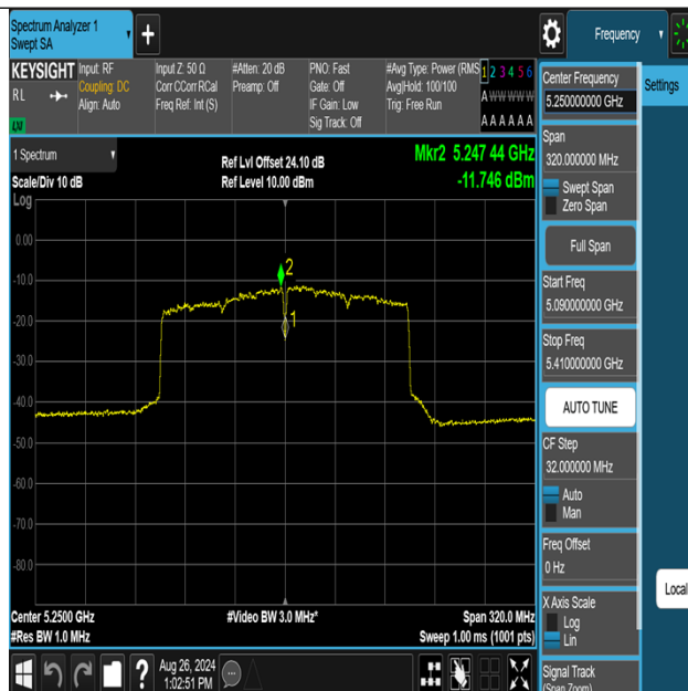
11AX160MIMO-Ant1-5250_UNII-1-PASS
