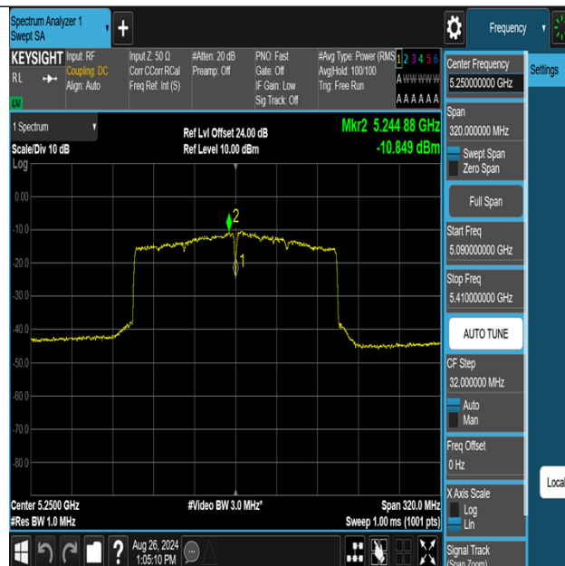
11AX160MIMO-Ant3-5250_UNII-1-PASS
