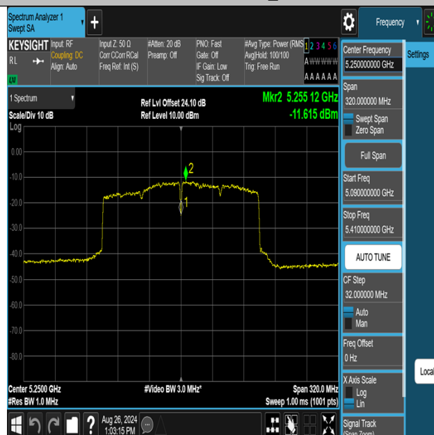
11AX160MIMO-Ant1-5250_UNII-2A-PASS
