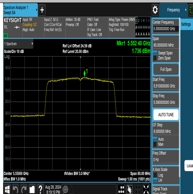
11AX40MIMO-Ant3-5550-PASS
