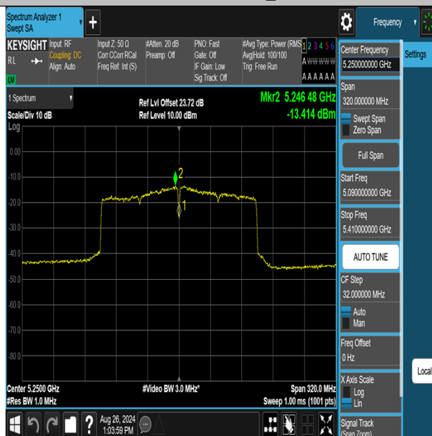
11AX160MIMO-Ant2-5250_UNII-1-PASS
