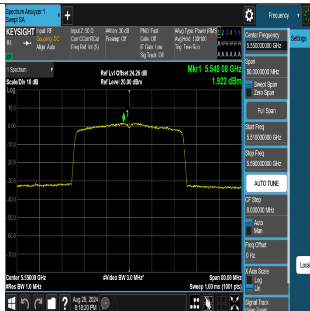
11AX40MIMO-Ant2-5550-PASS
