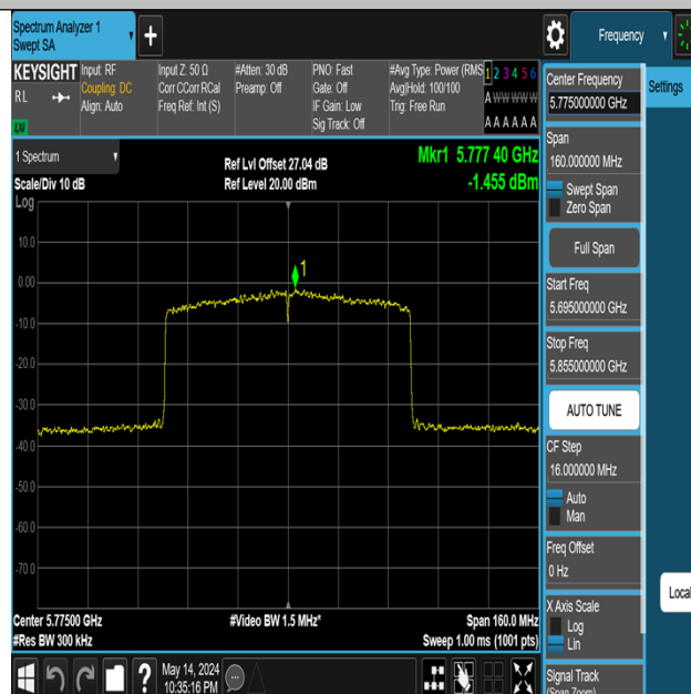
11AX80MIMO-Ant3-5775-PASS
