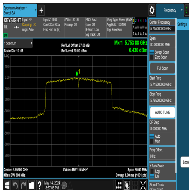
11AX40MIMO-Ant2-5755-PASS
