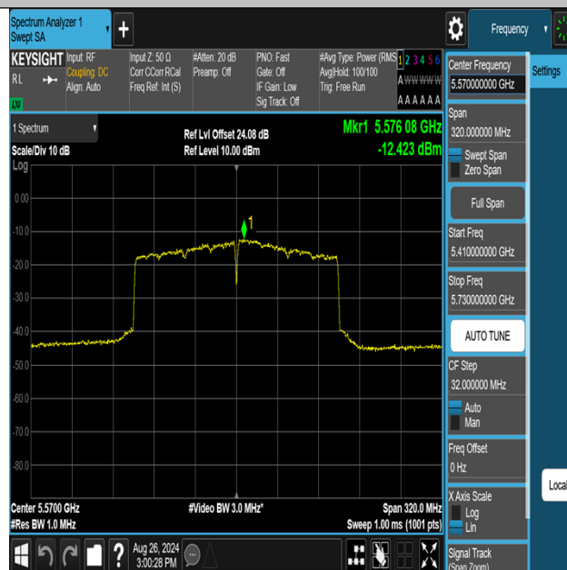
11AX160MIMO-Ant2-5570-PASS
