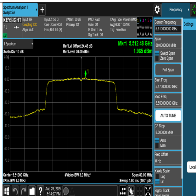
11AX40MIMO-Ant1-5510-PASS
