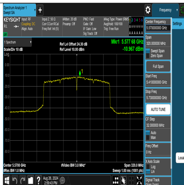
11AX160MIMO-Ant1-5570-PASS
