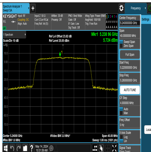
11AX20MIMO-Ant3-5240-PASS
