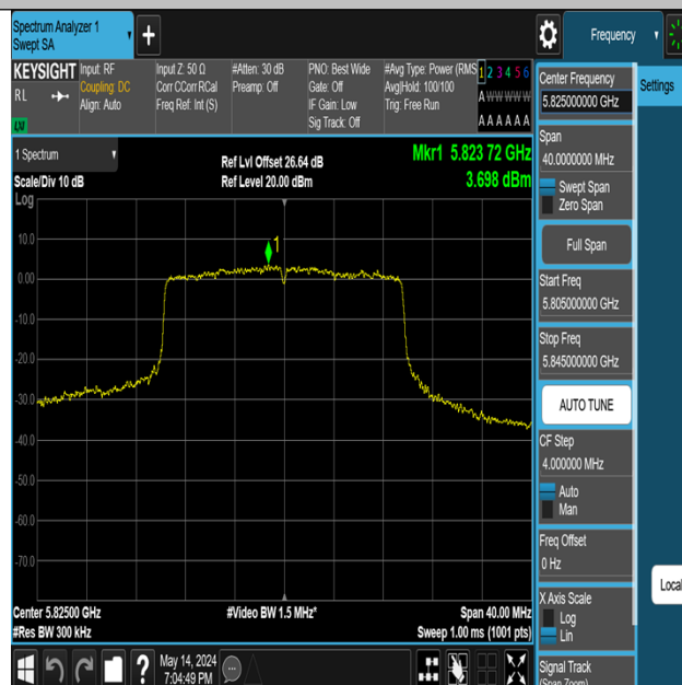
11AX20MIMO-Ant3-5825-PASS
