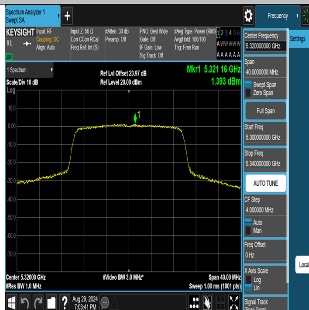
11AX20MIMO-Ant1-5320-PASS
