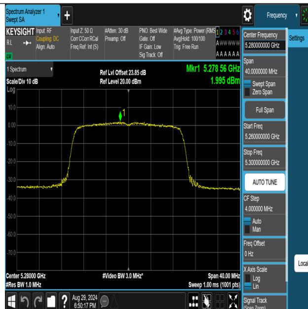
11AX20MIMO-Ant3-5280-PASS
