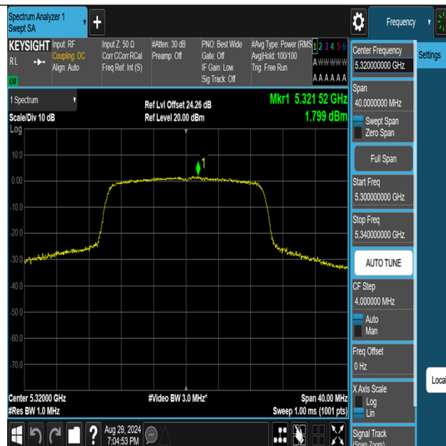
11AX20MIMO-Ant2-5320-PASS
