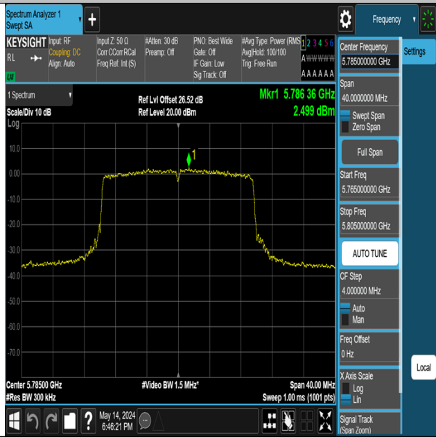
11AX20MIMO-Ant2-5785-PASS
