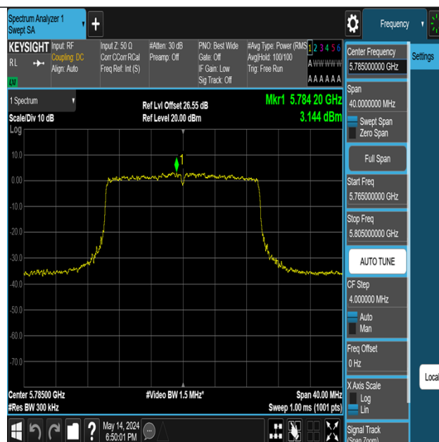
11AX20MIMO-Ant3-5785-PASS
