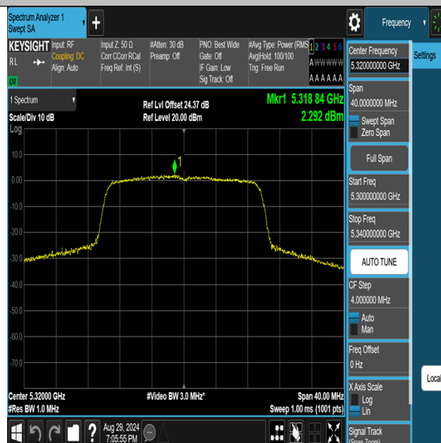
11AX20MIMO-Ant3-5320-PASS
