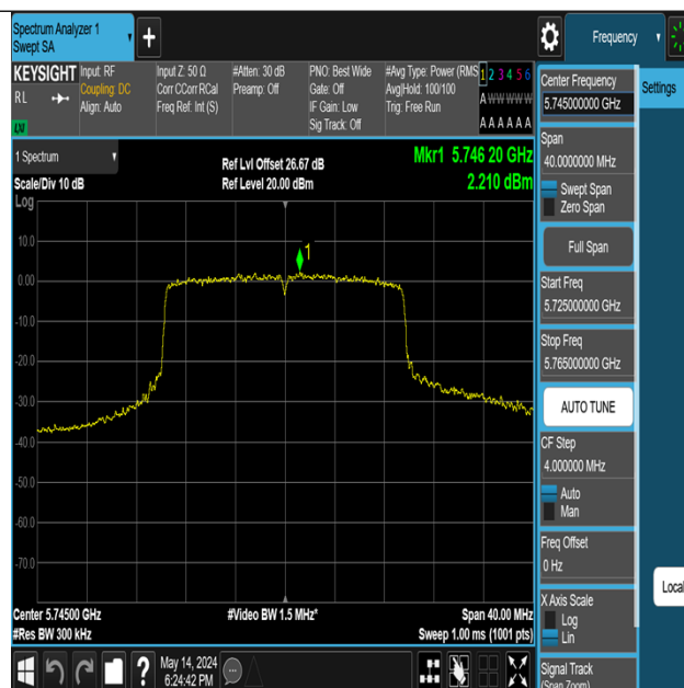
11AX20MIMO-Ant2-5745-PASS
