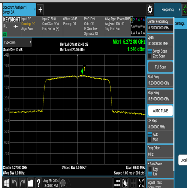
11AX40MIMO-Ant2-5270-PASS
