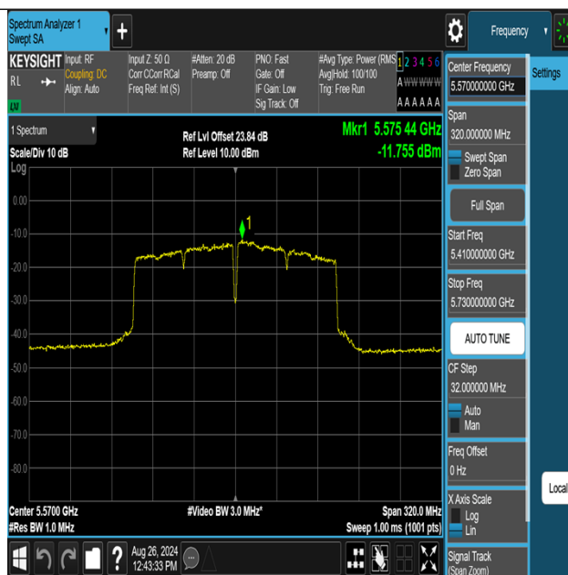
11AC160MIMO-Ant2-5570-PASS
