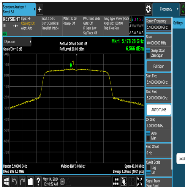
11AX20MIMO-Ant3-5180-PASS
