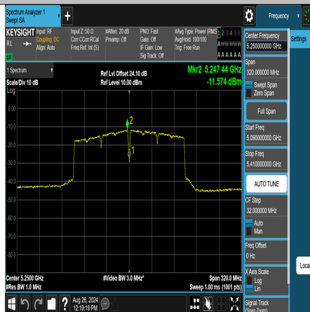
11AC160MIMO-Ant1-5250_UNII-1-PASS
