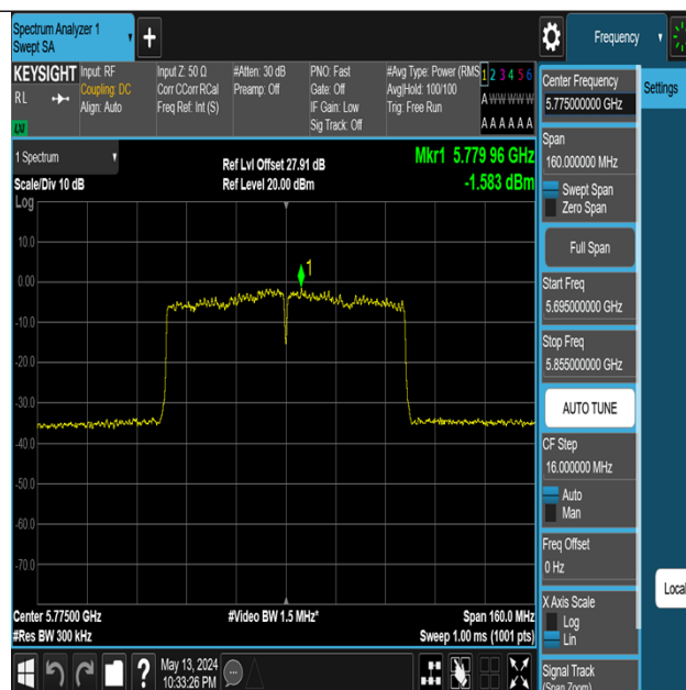
11AC80MIMO-Ant3-5775-PASS
