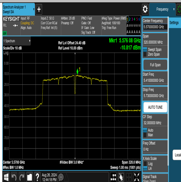
11AC160MIMO-Ant3-5570-PASS
