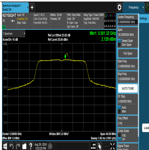
11AC20MIMO-Ant2-5500-PASS
