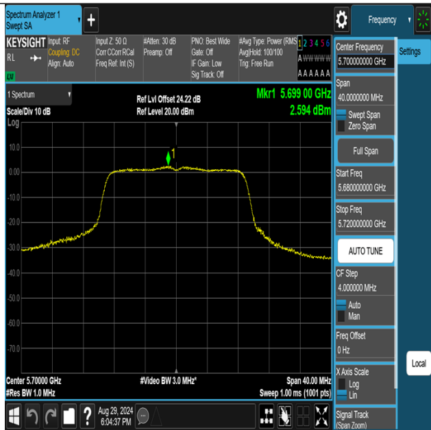
11AC20MIMO-Ant2-5700-PASS
