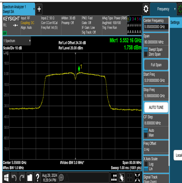
11AC40MIMO-Ant2-5550-PASS
