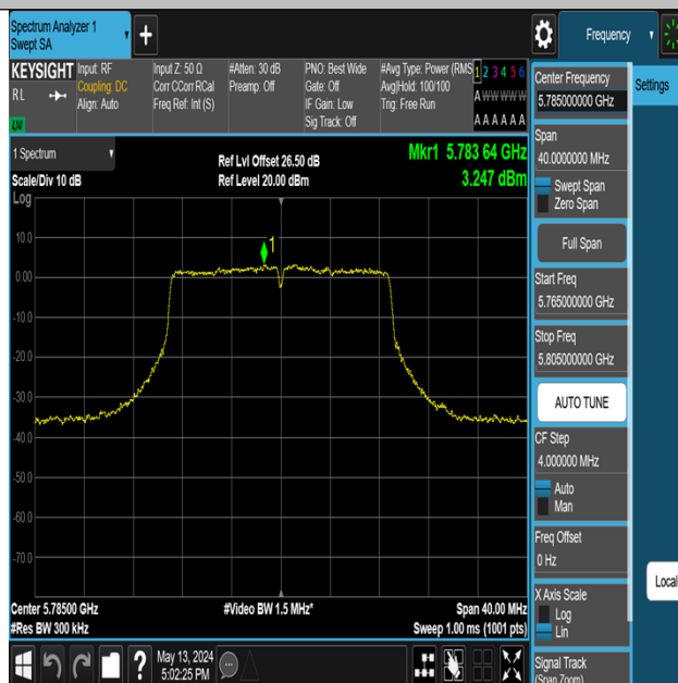
11AC20MIMO-Ant3-5785-PASS
