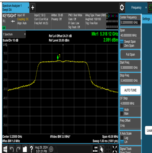
11AC20MIMO-Ant3-5320-PASS
