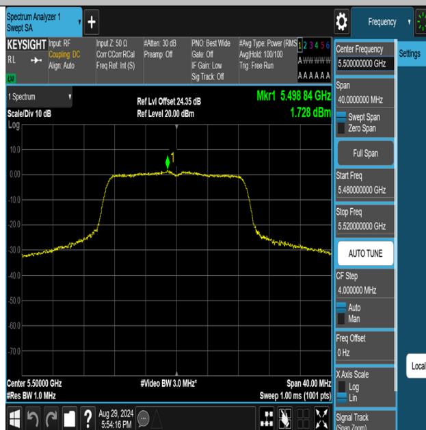
11AC20MIMO-Ant3-5500-PASS
