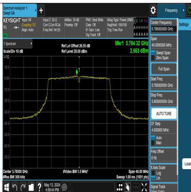
11AC20MIMO-Ant2-5785-PASS
