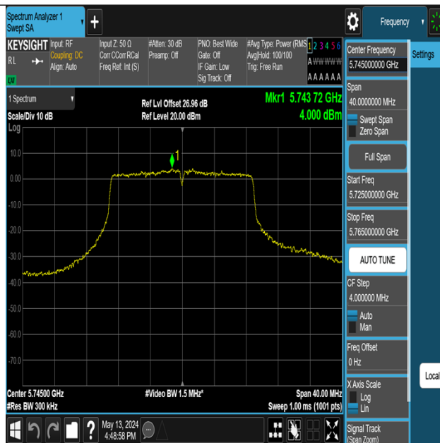
11AC20MIMO-Ant3-5745-PASS
