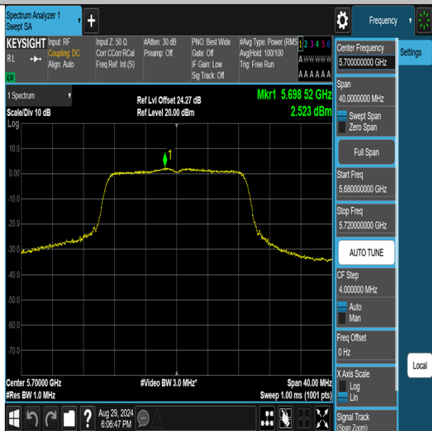
11AC20MIMO-Ant3-5700-PASS
