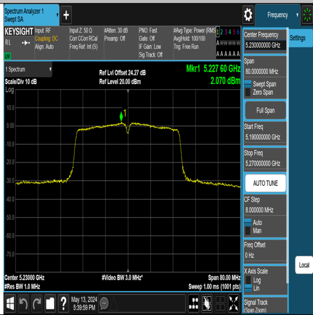
11AC40MIMO-Ant2-5230-PASS
