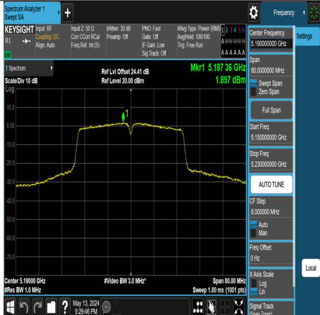
11AC40MIMO-Ant2-5190-PASS
