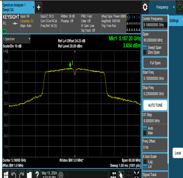
11AC40MIMO-Ant3-5190-PASS
