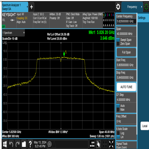
11AC20MIMO-Ant3-5825-PASS
