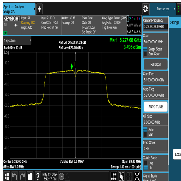
11AC40MIMO-Ant3-5230-PASS
