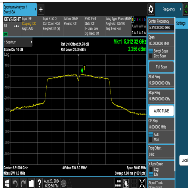
11AC40MIMO-Ant3-5310-PASS
