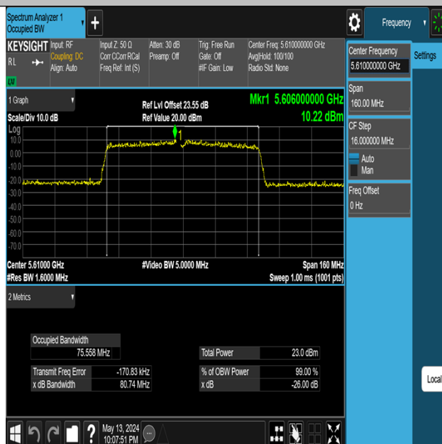
11AC80MIMO-Ant1-5610
