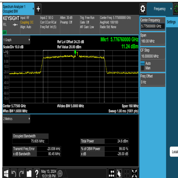
11AC80MIMO-Ant3-5775
