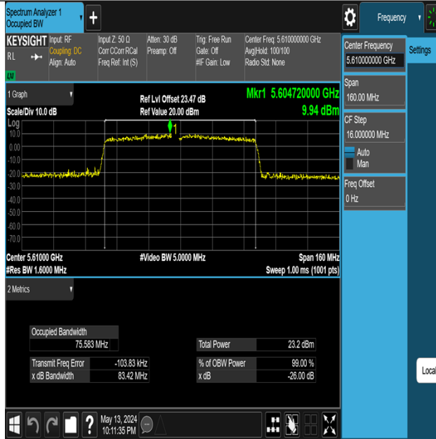
11AC80MIMO-Ant2-5610
