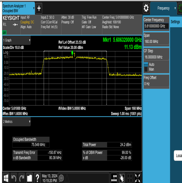
11AC80MIMO-Ant3-5610
