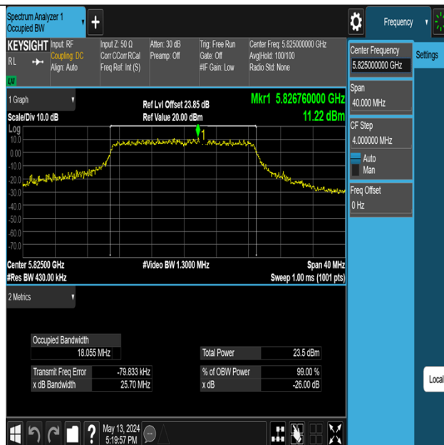
11AC20MIMO-Ant3-5825
