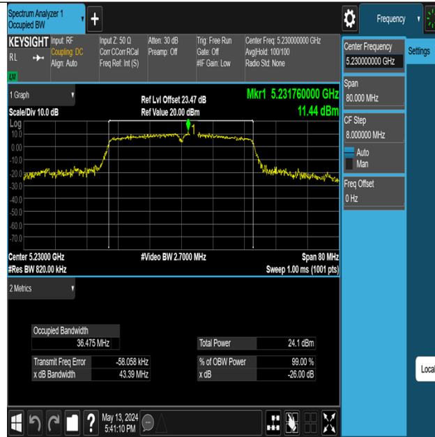
11AC40MIMO-Ant3-5230
