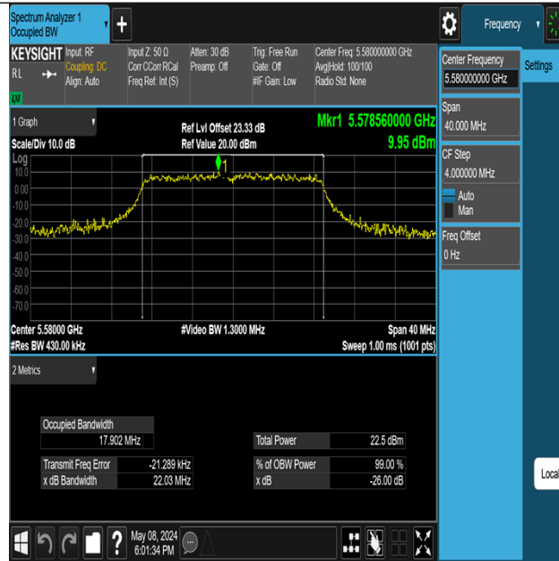
11N20MIMO-Ant2-5580
