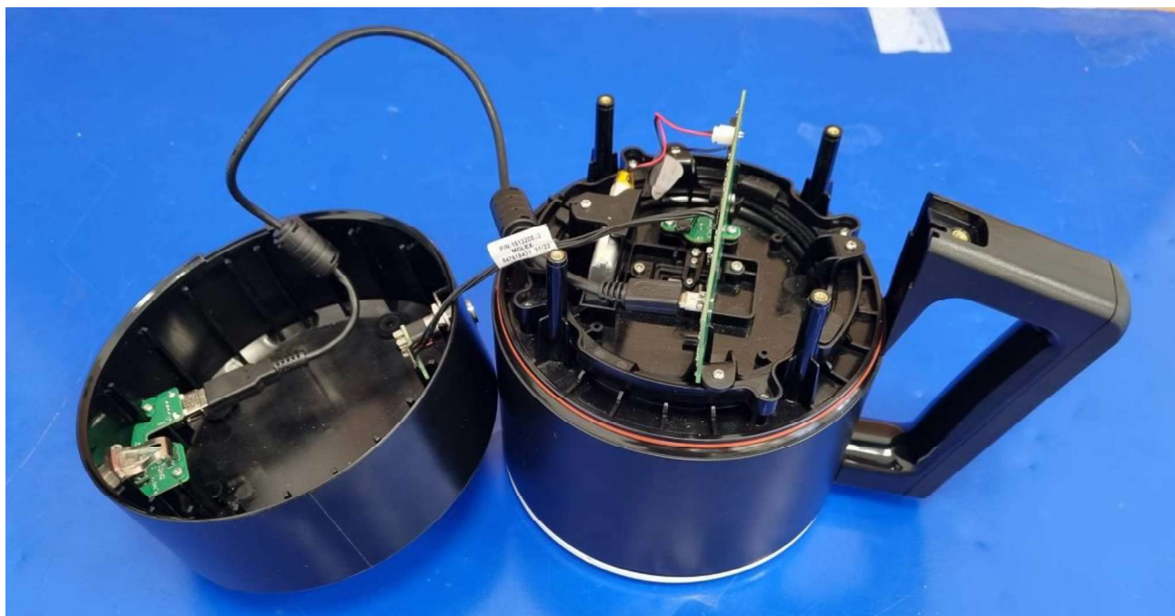
Photograph № 4, 5, 6 SCiOCUP internal view
