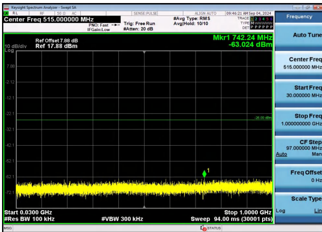
30MHz-1G
