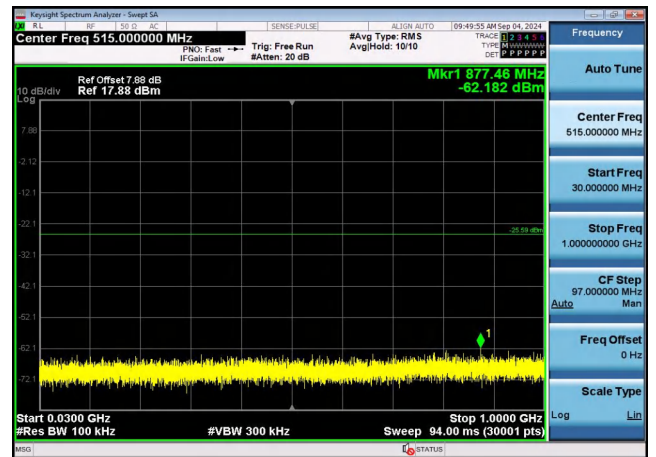
30MHz-1G
