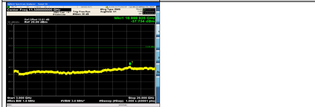
Band66_20MHz_16QAM_132572_1RB#99_300 0~20000_3000~20000
