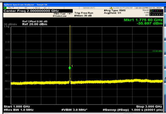
Band66_1.4MHz_QPSK_132665_1RB#0_1000~3000_1000~3000
