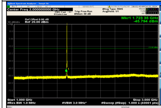
Band4_3MHz_16QAM_20175_1RB#14_1000~3000_1000~3000
