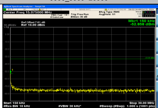
Band4_3MHz_16QAM_20175_15RB#0_0.15~30_0.15~30
