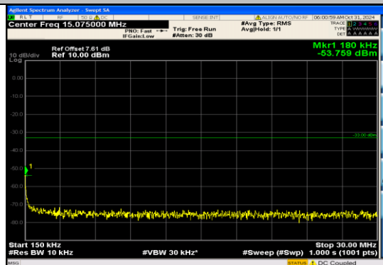
Band4_3MHz_QPSK_20175_1RB#14_0.15~30_0.15~30
