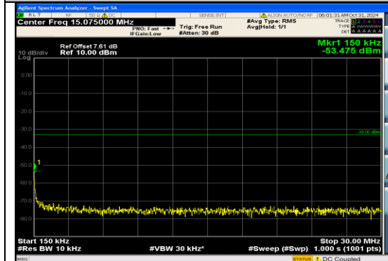
Band4_3MHz_16QAM_20175_1RB#14_0.15~30_0.15~30
