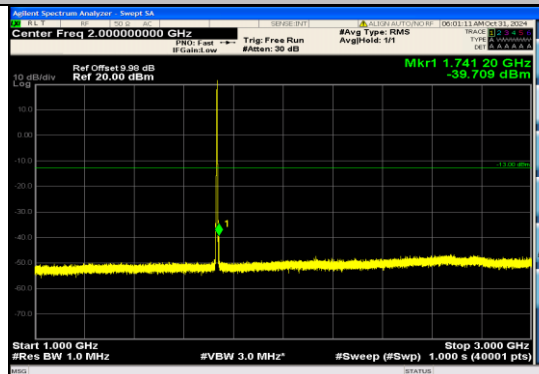
Band4_3MHz_QPSK_20175_1RB#14_1000~3000_00_1000~3000
