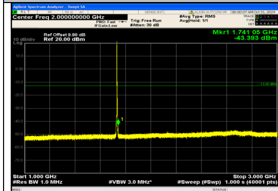
Band4_3MHz_QPSK_20175_1RB#0_1000~3000_0_1000~3000
