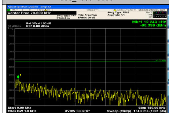
Band4_3MHz_16QAM_20175_15RB#0_0.009~0.15_0.009~0.15
