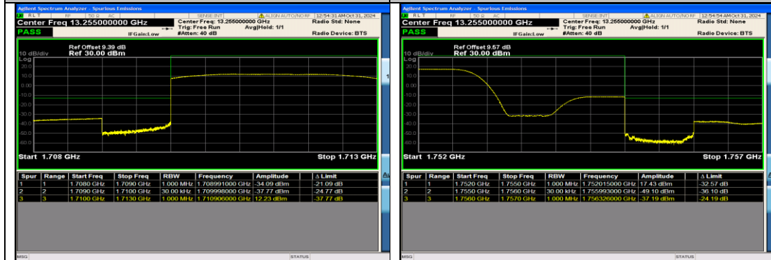
Band4_3MHz_QPSK_19965_15RB#0
