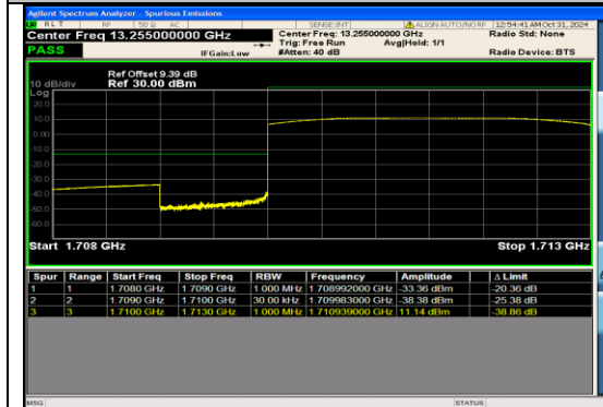
Band4_3MHz_16QAM_19965_15RB#0
