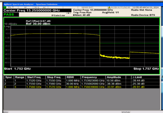
Band4_3MHz_16QAM_20385_15RB#0
