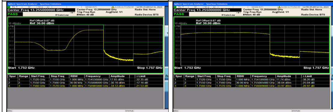
Band4_3MHz_QPSK_20385_1RB#14
