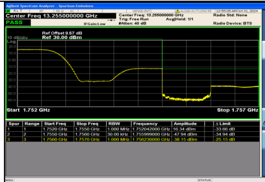
Band4_3MHz_16QAM_20385_1RB#0
