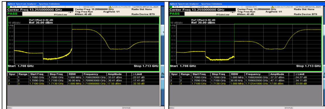
Band4_3MHz_16QAM_19965_1RB#0
