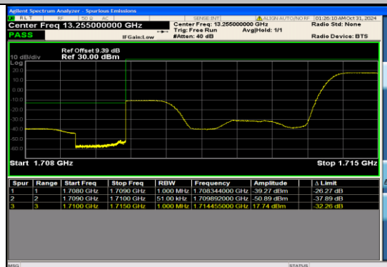
Band4_5MHz_QPSK_19975_1RB#24
