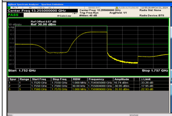
Band4_3MHz_16QAM_20385_1RB#14
