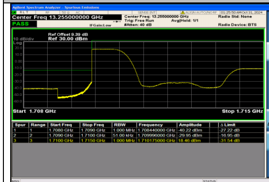
Band4_5MHz_QPSK_19975_1RB#0
