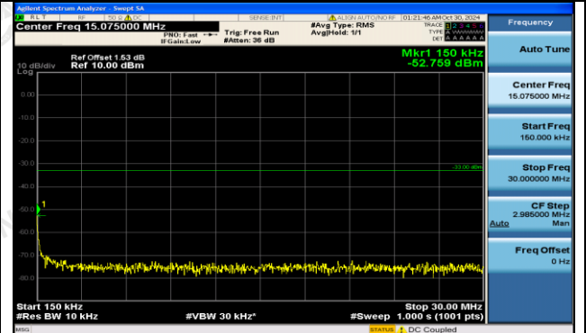
Band2-9400-0.15~30MHz-PASS
