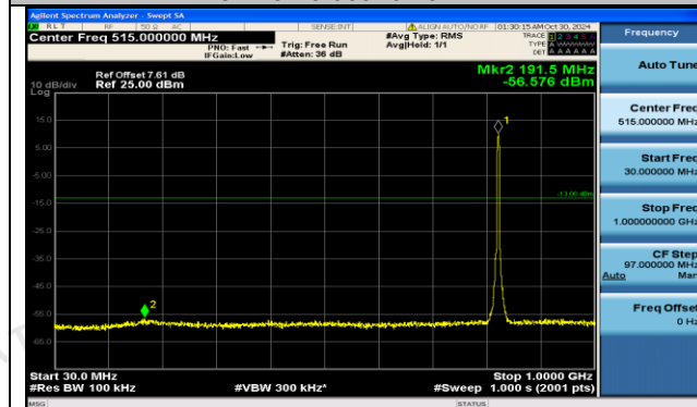
Band5-4132-30~1000MHz-PASS
