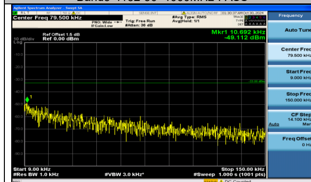
Band5-4182-0.009~0.15MHz-PASS
