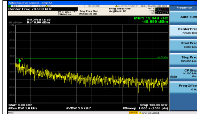
Band2-9400-0.009~0.15MHz-PASS
