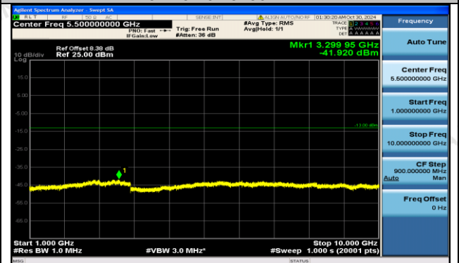
Band5-4132-1000~10000MHz-PASS
