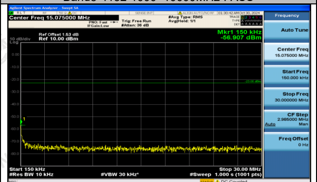
Band5-4182-0.15~30MHz-PASS
