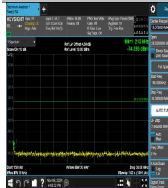
Band2_15MHz_16QAM_19125_1RB#0_0.15~30_0.15~30
