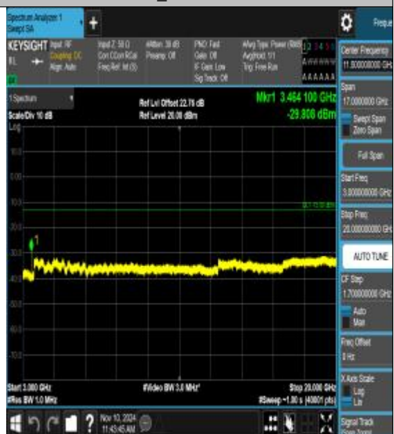
Band4_1.4MHz_16QAM_20175_1RB#0_3000~20 000_3000~20000
