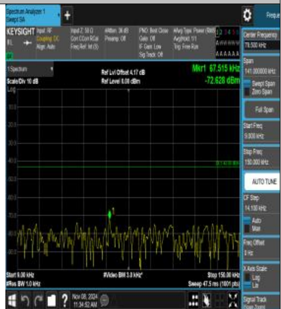
Band2_3MHz_16QAM_19185_1RB#0_0.009~0.15 _0.009~0.15
