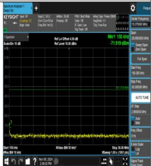
Band2_5MHz_QPSK_18900_1RB#0_0.15~30_0.15~30
