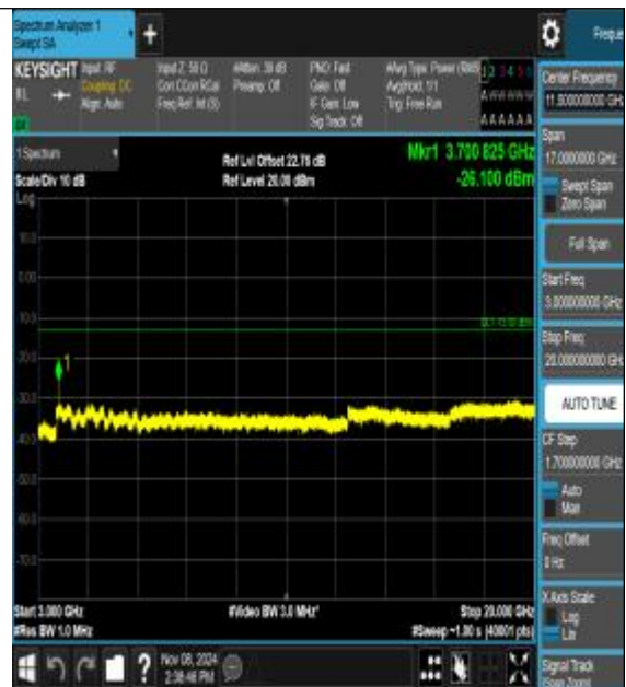
Band2_5MHz_16QAM_18625_1RB#0_3000~20000_3000~20000
