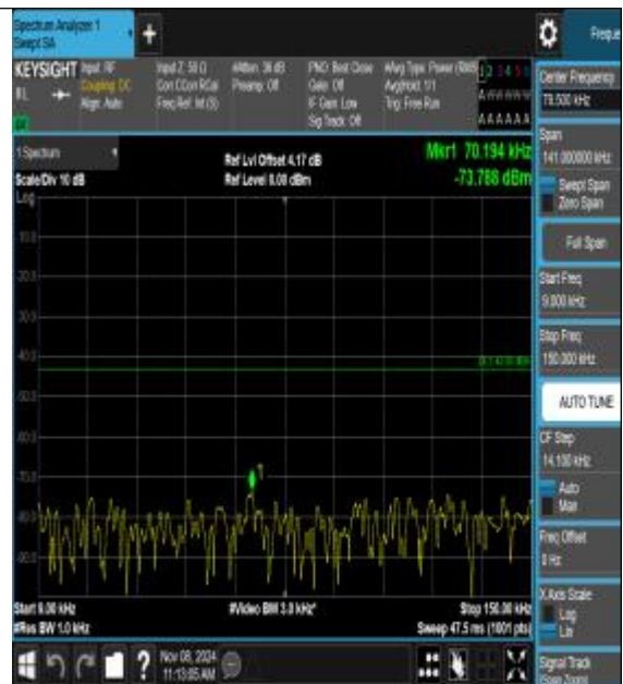
Band2_1.4MHz_16QAM_19193_1RB#0_0.009~0.15_0.009~0.15
