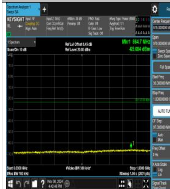
Band2_15MHz_QPSK_19125_1RB#0_30~1000_ 30~1000
