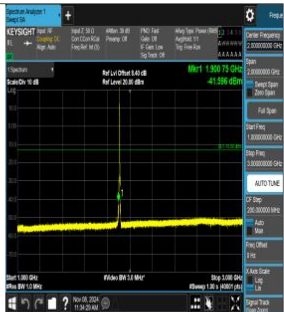
Band2_3MHz_QPSK_19185_1RB#0_1000~3000_ 1000~3000
