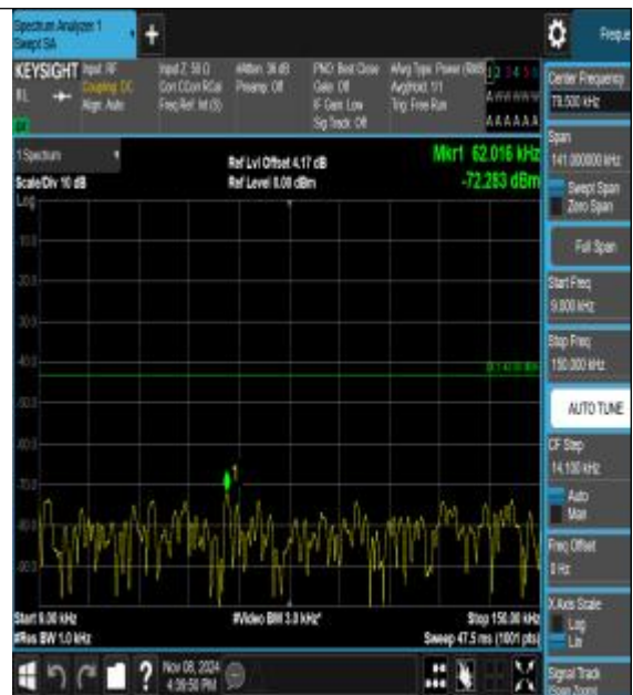
Band2_15MHz_16QAM_18675_1RB#0_0.009~0.1 5_0.009~0.15
