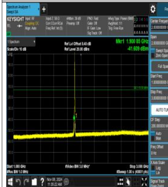
Band2_3MHz_16QAM_19185_1RB#0_1000~3000_0_1000~3000
