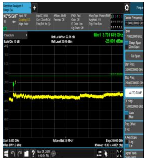
Band2_15MHz_16QAM_18675_1RB#0_3000~20000_3000~20000
