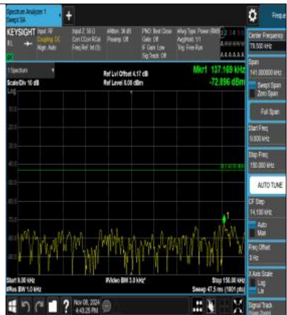
Band2_15MHz_16QAM_19125_1RB#0_0.009~0.15_0.009~0.15
