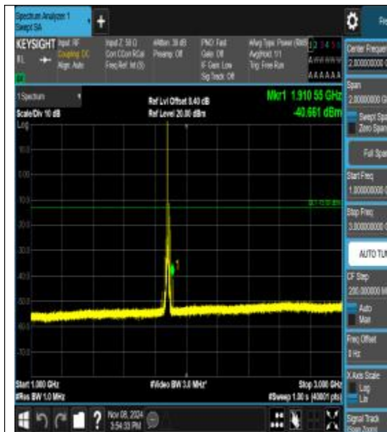
Band2_10MHz_16QAM_18900_1RB#0_1000~3000_1000~3000
