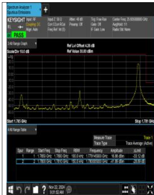
Band66_15MHz_QPSK_132597_1RB#74
