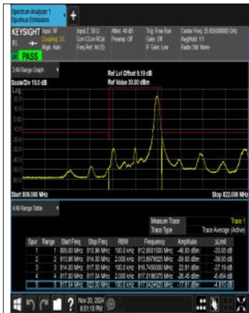
Band26_3MHz_QPSK_26705_1RB#14
