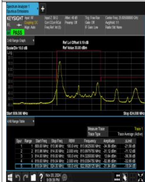
Band26_5MHz_QPSK_26715_1RB#0
