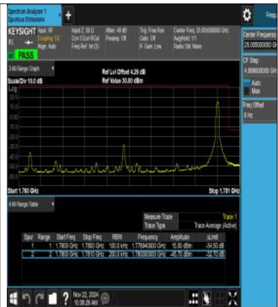
Band66_20MHz_16QAM_132572_1RB#99
