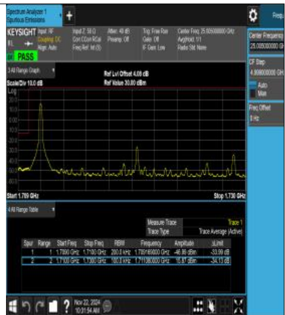
Band66_20MHz_16QAM_132072_1RB#0
