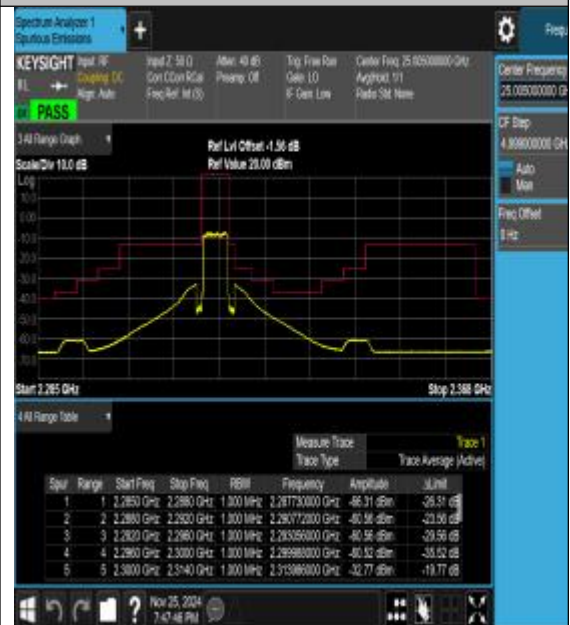
Band40_5MHz_16QAM_38825_25RB#0
