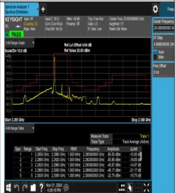
Band40_10MHz_16QAM_38800_1RB#0
