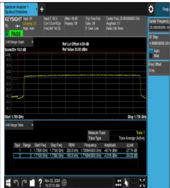
Band66_20MHz_16QAM_132072_100RB#0
