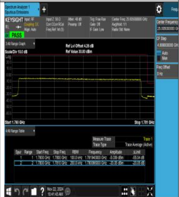
Band66_20MHz_16QAM_132572_100RB#0
