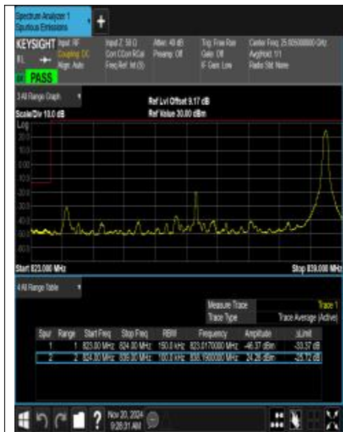
Band26_15MHz_QPSK_26865_1RB#74
