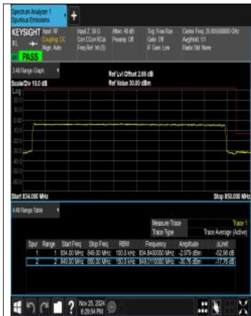
Band26_15MHz_QPSK_26965_75RB#0
