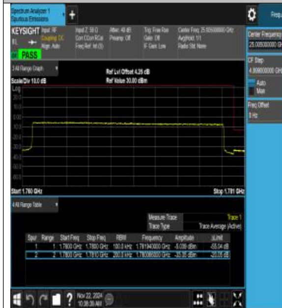
Band66_20MHz_QPSK_132572_100RB#0
