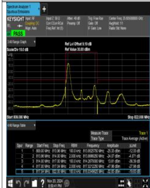
Band26_3MHz_QPSK_26705_1RB#0
