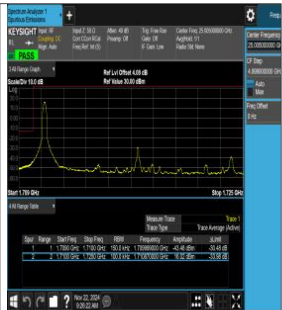
Band66_15MHz_16QAM_132047_1RB#0
