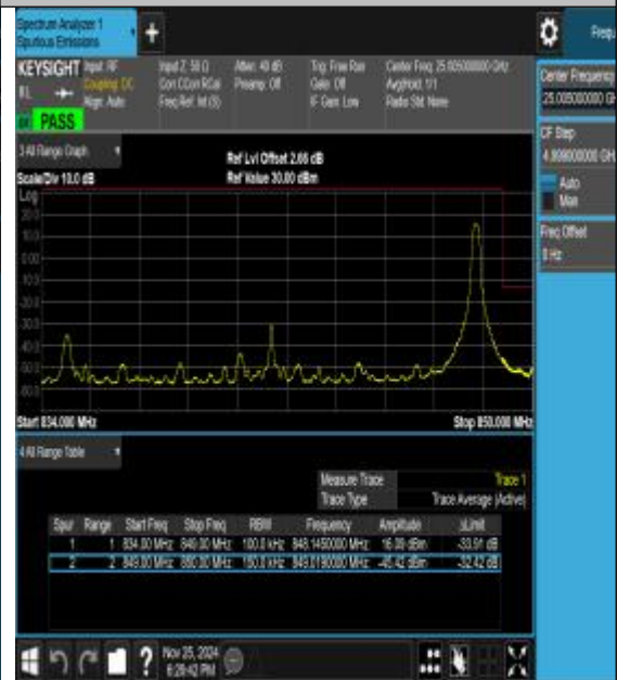
Band26_15MHz_16QAM_26965_1RB#74
