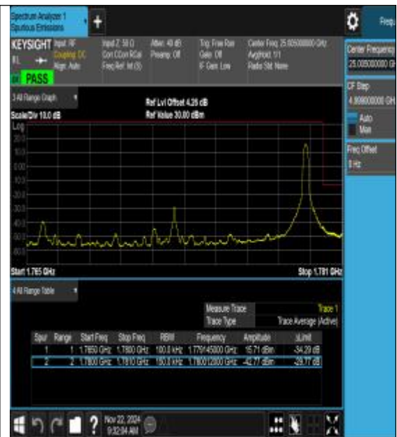
Band66_15MHz_16QAM_132597_1RB#74
