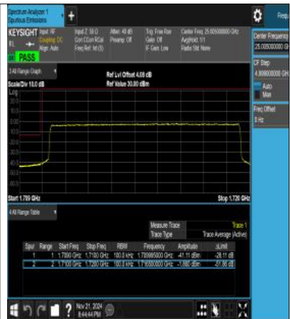
Band66_10MHz_16QAM_132022_50RB#0
