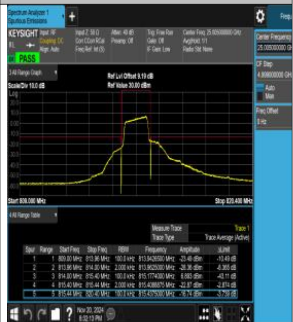
Band26_1.4MHz_16QAM_26697_6RB#0
