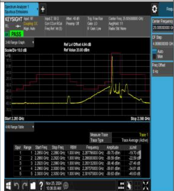
Band40_5MHz_16QAM_39125_1RB#0
