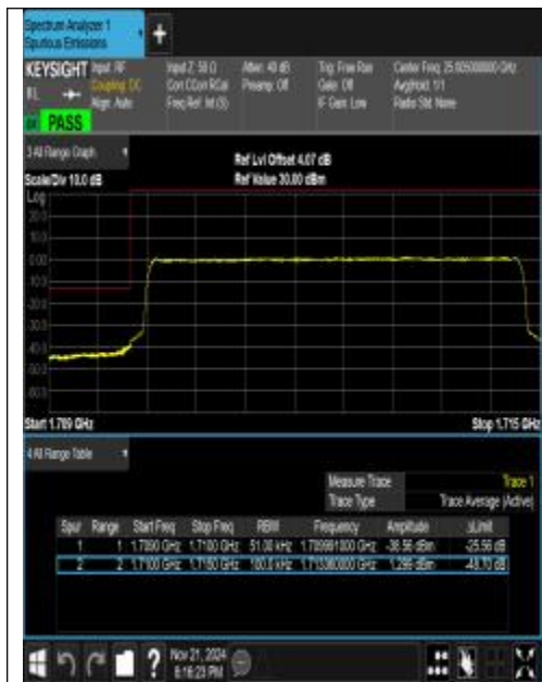
Band66_5MHz_QPSK_131997_25RB#0
