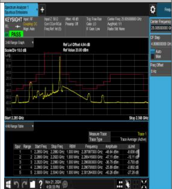
Band40_10MHz_16QAM_38750_1RB#49
