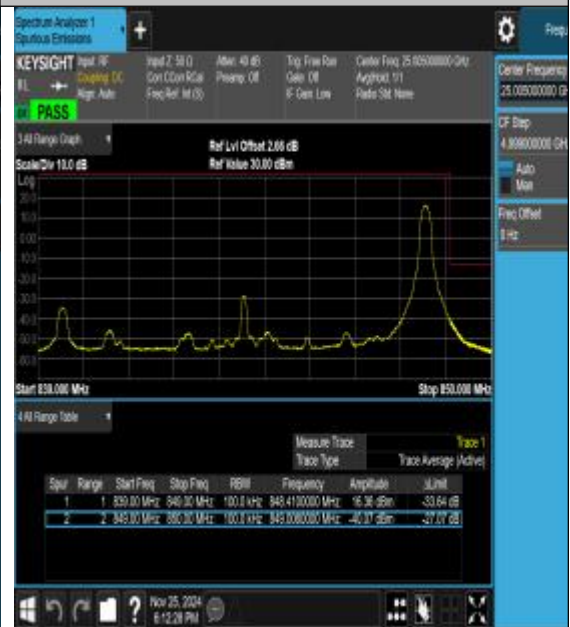
Band26_10MHz_16QAM_26990_1RB#49
