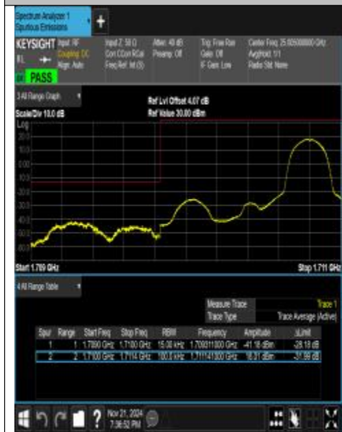
Band66_1.4MHz_QPSK_131979_1RB#5
