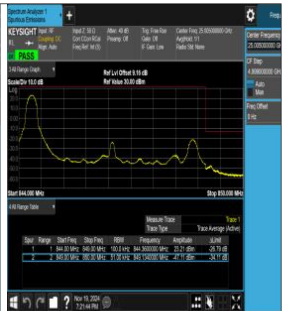
Band26_5MHz_16QAM_27015_1RB#0
