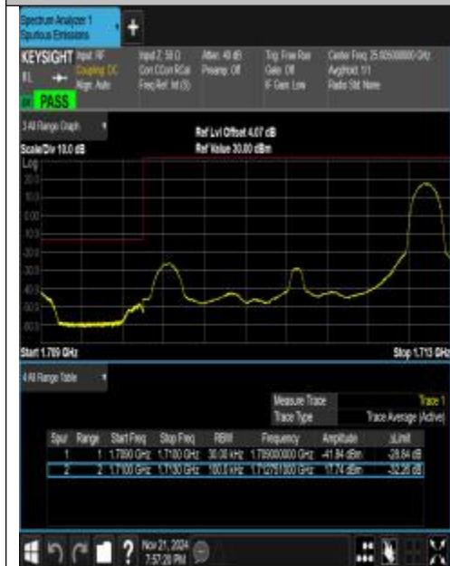
Band66_3MHz_QPSK_131987_1RB#14
