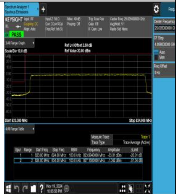
Band26_10MHz_16QAM_26840_50RB#0
