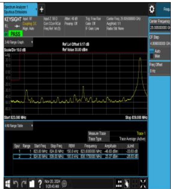
Band26_15MHz_16QAM_26865_1RB#74
