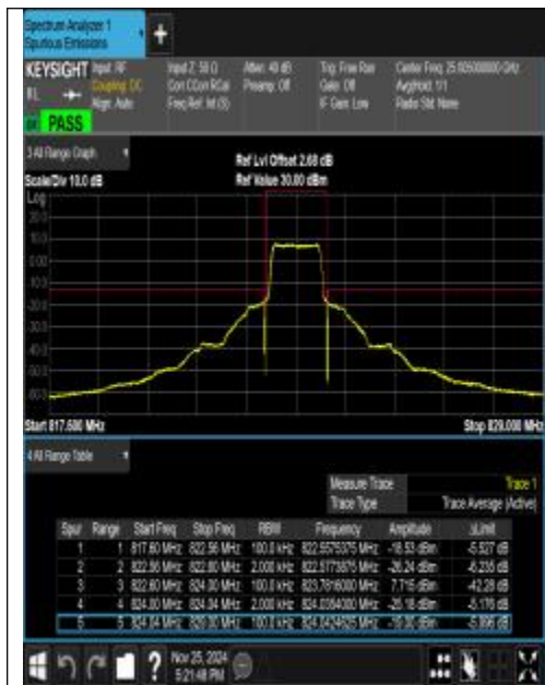
Band26_1.4MHz_QPSK_26783_6RB#0
