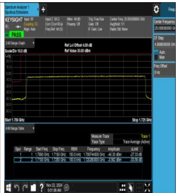
Band66_15MHz_16QAM_132047_75RB#0
