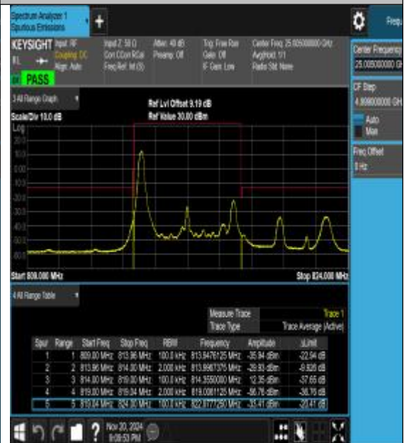
Band26_5MHz_16QAM_26715_1RB#0
