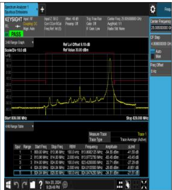
Band26_10MHz_16QAM_26740_1RB#49
