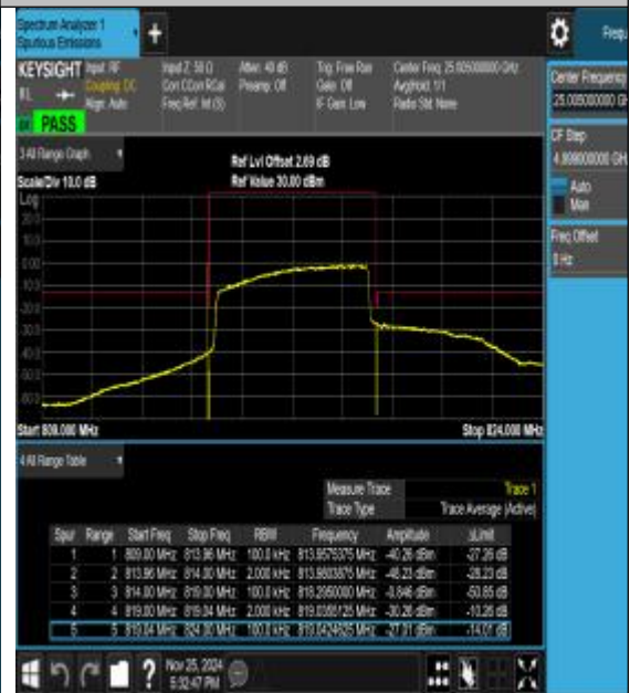
Band26_5MHz_16QAM_26715_25RB#0
