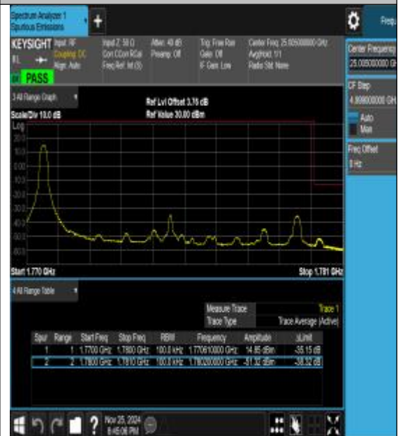
Band66_10MHz_16QAM_132622_1RB#0
