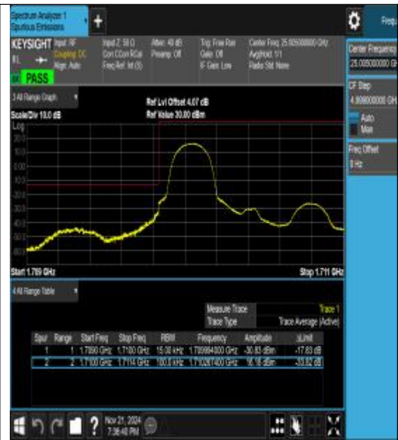
Band66_1.4MHz_16QAM_131979_1RB#0
