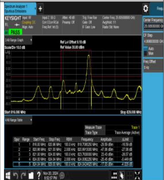
Band26_3MHz_16QAM_26775_1RB#14
