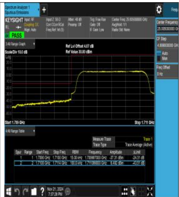
Band66_1.4MHz_16QAM_131979_6RB#0
