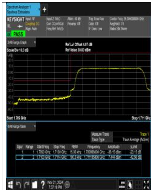
Band66_1.4MHz_QPSK_131979_6RB#0
