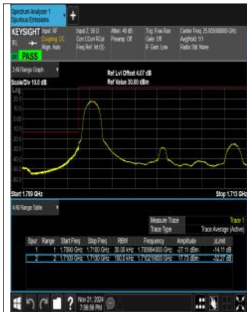
Band66_3MHz_QPSK_131987_1RB#0
