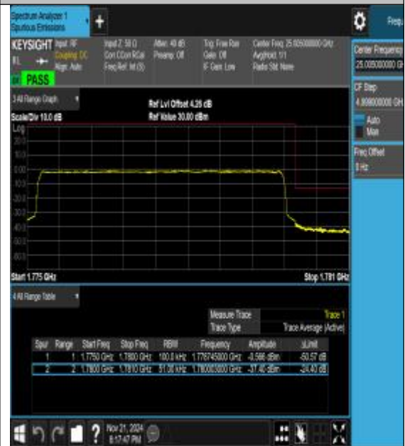
Band66_5MHz_16QAM_132647_25RB#0
