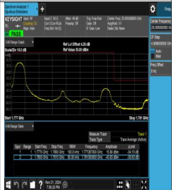
Band66_3MHz_16QAM_132657_1RB#0
