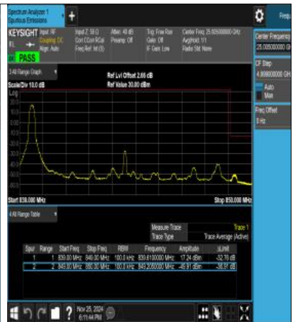
Band26_10MHz_16QAM_26990_1RB#0
