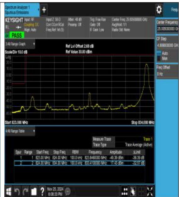
Band26_10MHz_16QAM_26840_1RB#49
