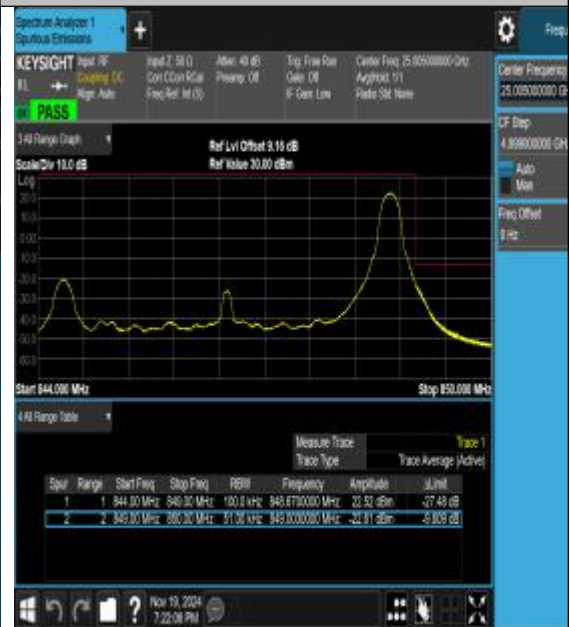
Band26_5MHz_16QAM_27015_1RB#24
