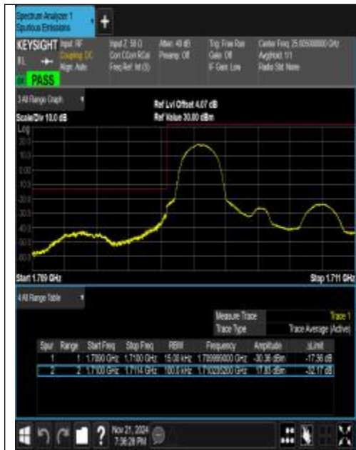
Band66_1.4MHz_QPSK_131979_1RB#0
