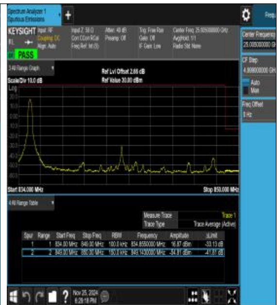
Band26_15MHz_16QAM_26965_1RB#0
