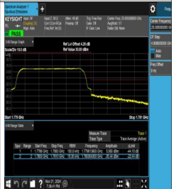
Band66_1.4MHz_16QAM_132665_6RB#0
