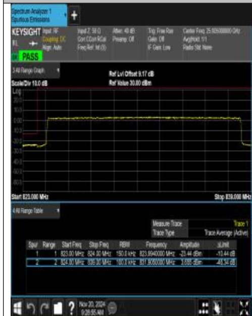
Band26_15MHz_QPSK_26865_75RB#0
