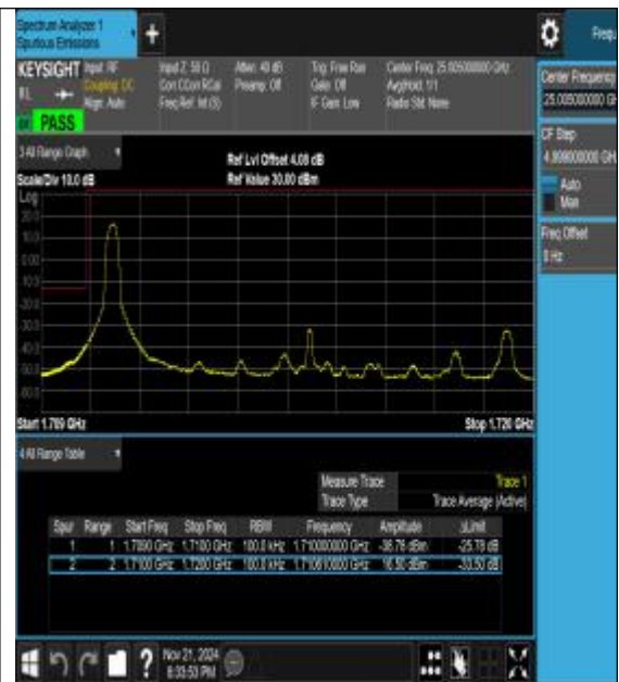
Band66_10MHz_16QAM_132022_1RB#0
