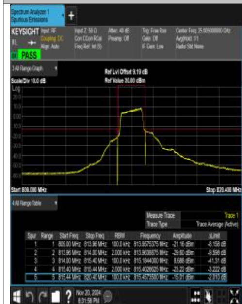
Band26_1.4MHz_QPSK_26697_6RB#0
