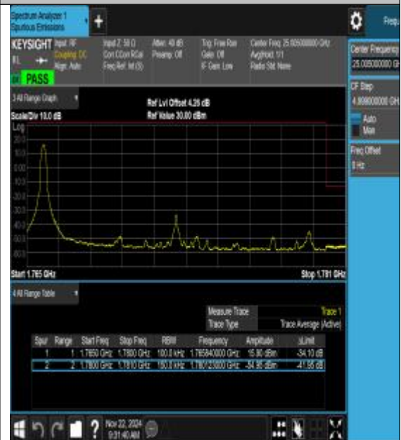
Band66_15MHz_16QAM_132597_1RB#0
