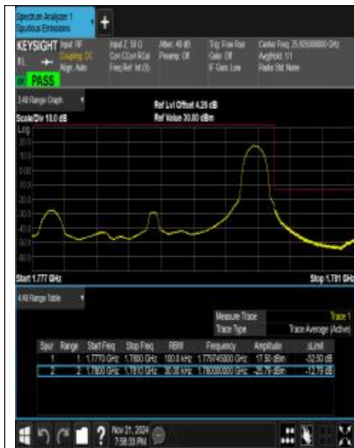
Band66_3MHz_QPSK_132657_1RB#14
