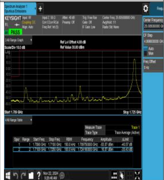
Band66_15MHz_16QAM_132047_1RB#74
