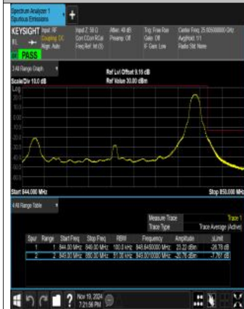
Band26_5MHz_QPSK_27015_1RB#24
