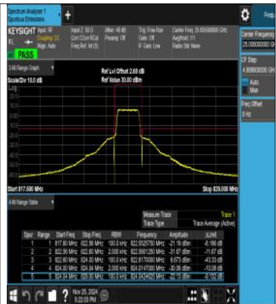
Band26_1.4MHz_16QAM_26783_6RB#0
