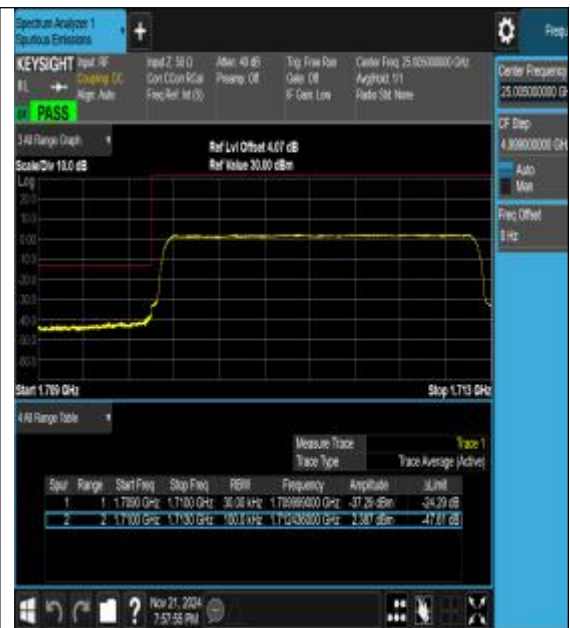
Band66_3MHz_16QAM_131987_15RB#0
