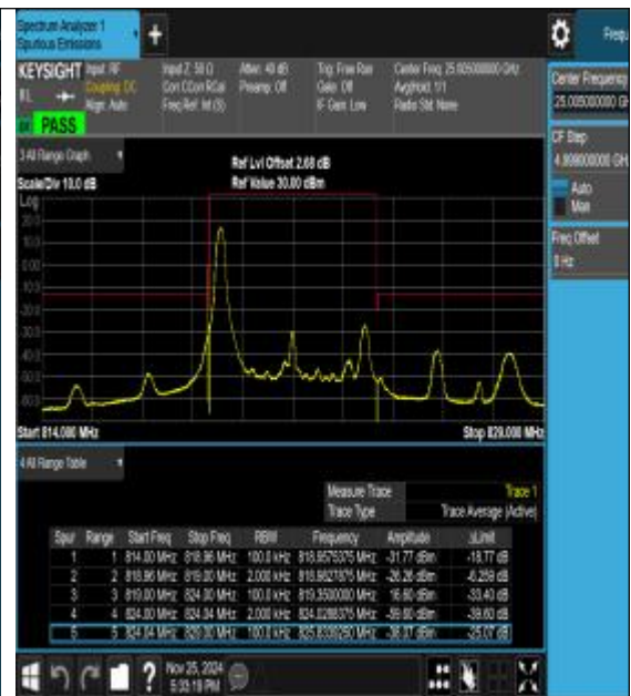
Band26_5MHz_16QAM_26765_1RB#0
