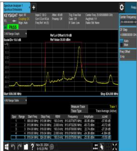
Band26_5MHz_16QAM_26715_1RB#24
