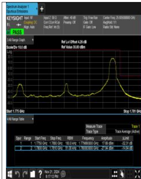
Band66_5MHz_QPSK_132647_1RB#24
