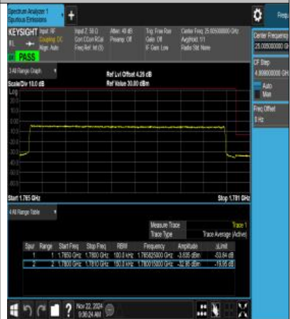
Band66_15MHz_16QAM_132597_75RB#0
