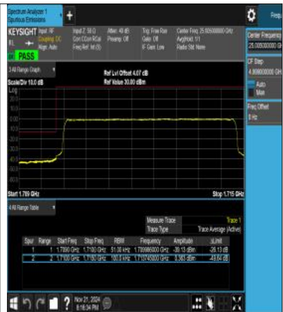
Band66_5MHz_16QAM_131997_25RB#0
