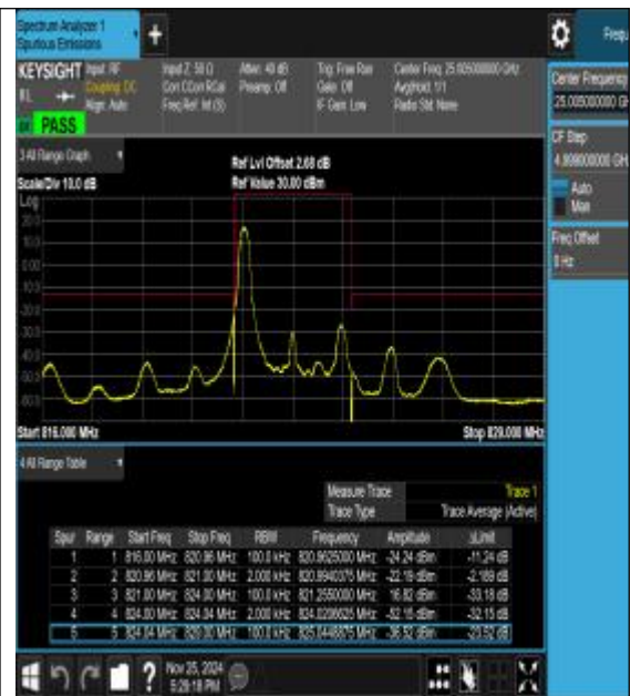
Band26_3MHz_16QAM_26775_1RB#0
