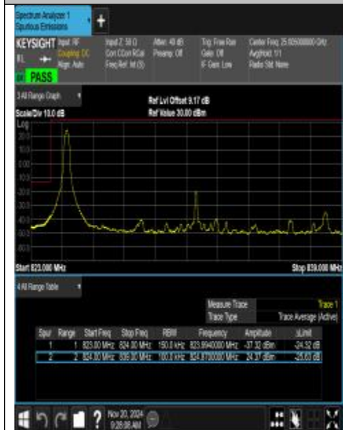
Band26_15MHz_QPSK_26865_1RB#0
