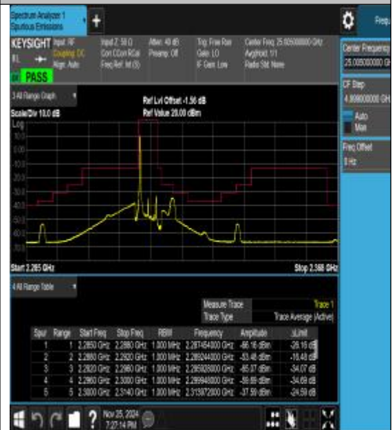
Band40_5MHz_16QAM_38825_1RB#0
