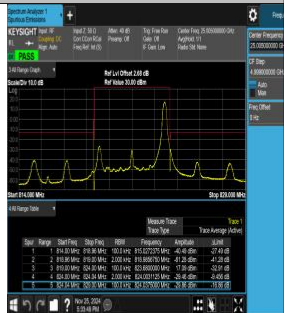
Band26_5MHz_16QAM_26765_1RB#24
