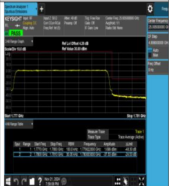
Band66_3MHz_16QAM_132657_15RB#0
