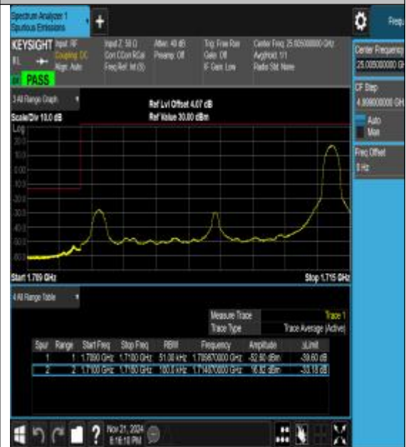
Band66_5MHz_16QAM_131997_1RB#24
