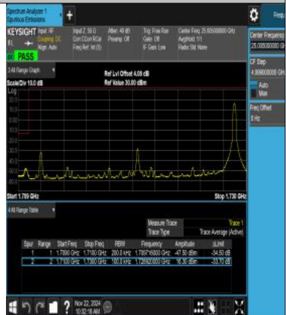
Band66_20MHz_16QAM_132072_1RB#99
