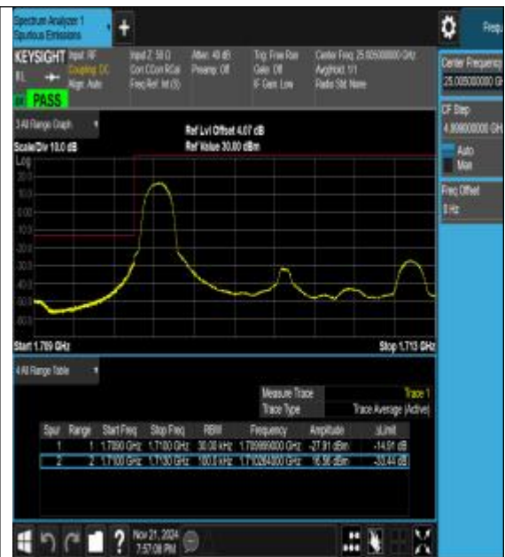
Band66_3MHz_16QAM_131987_1RB#0
