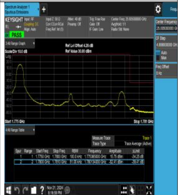
Band66_5MHz_16QAM_132647_1RB#0
