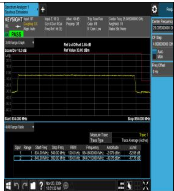
Band26_15MHz_16QAM_26965_75RB#0
