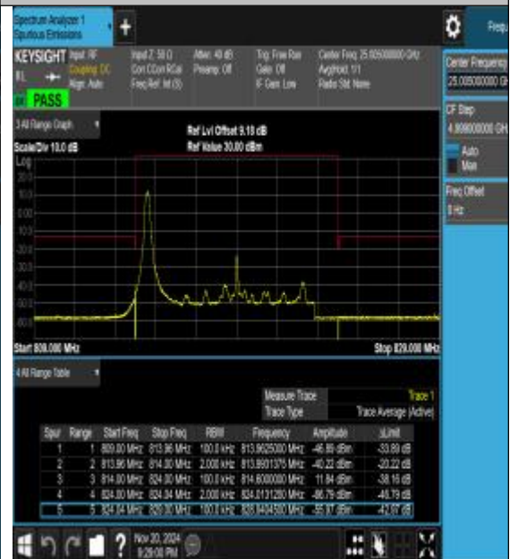
Band26_10MHz_16QAM_26740_1RB#0
