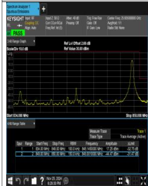
Band26_15MHz_QPSK_26965_1RB#74
