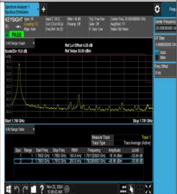
Band66_20MHz_16QAM_132572_1RB#0
