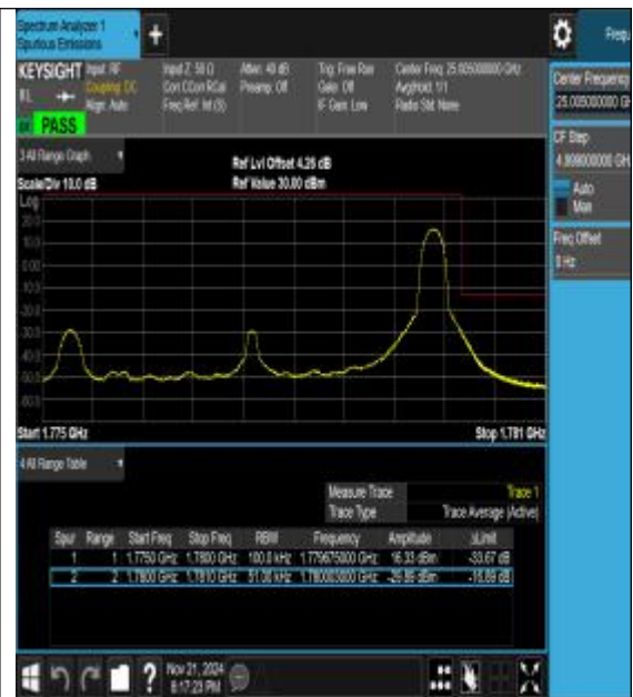
Band66_5MHz_16QAM_132647_1RB#24
