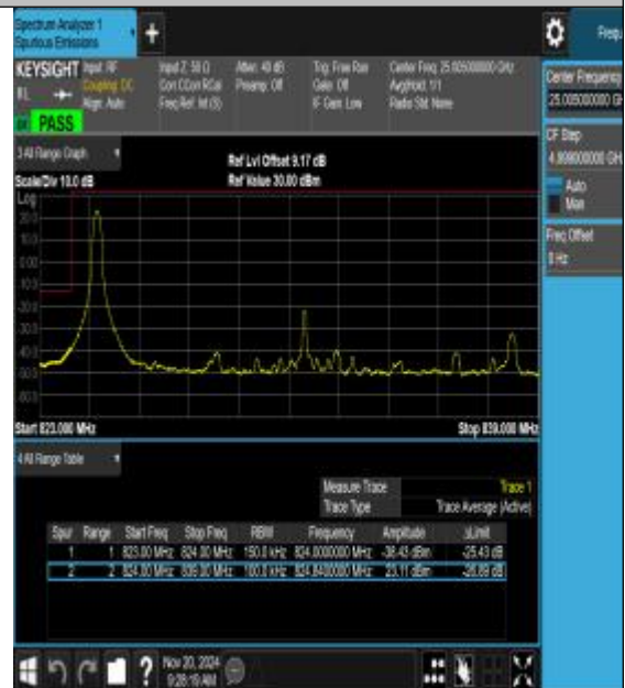
Band26_15MHz_16QAM_26865_1RB#0
