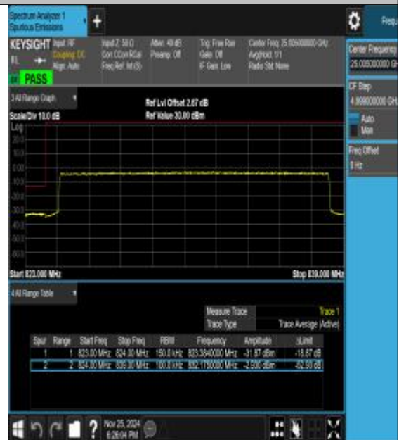
Band26_15MHz_16QAM_26865_75RB#0
