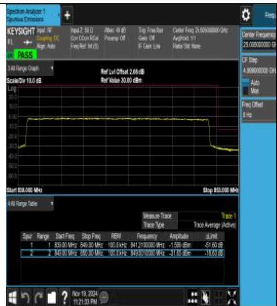
Band26_10MHz_16QAM_26990_50RB#0
