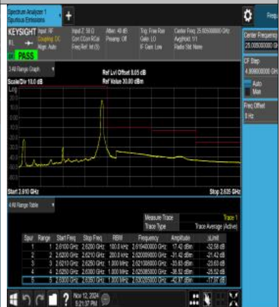
Band38_10MHz_16QAM_38200_1RB#49
