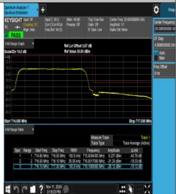
Band12_1.4MHz_16QAM_23173_6RB#0
