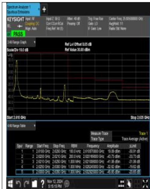
Band38_10MHz_QPSK_38200_1RB#0
