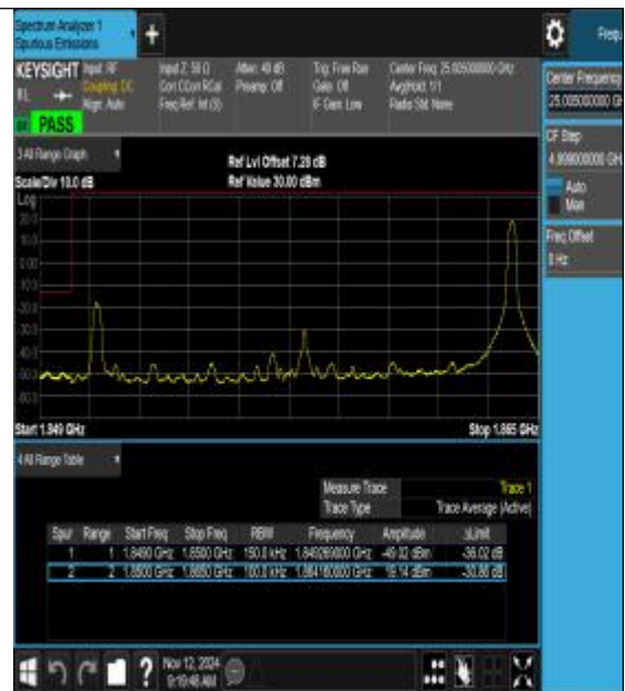
Band25_15MHz_16QAM_26115_1RB#74
