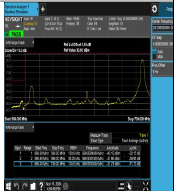
Band12_10MHz_16QAM_23060_1RB#49
