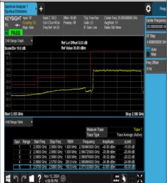
Band38_10MHz_16QAM_37800_1RB#0
