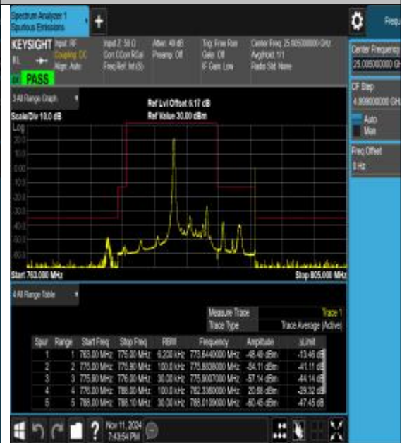
Band13_5MHz_16QAM_23255_1RB#0
