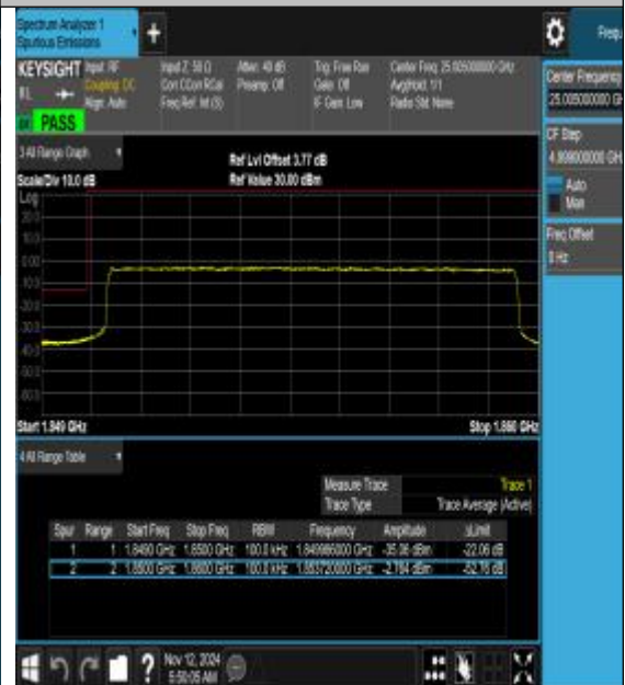
Band25_10MHz_16QAM_26090_50RB#0
