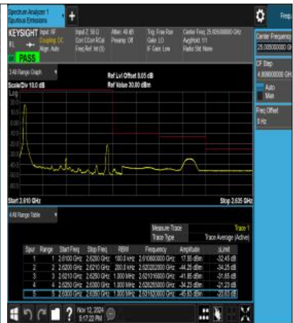
Band38_10MHz_16QAM_38200_1RB#0
