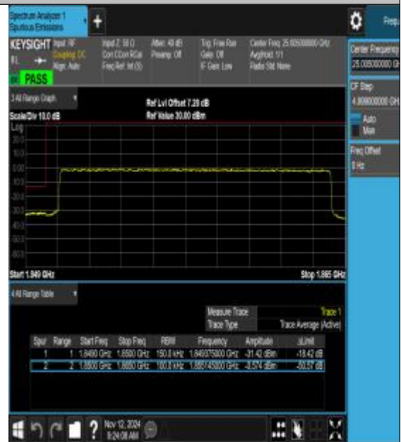
Band25_15MHz_16QAM_26115_75RB#0
