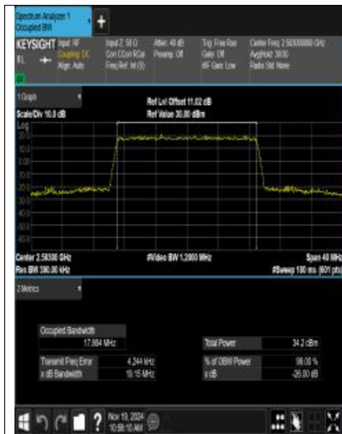
Band41-20MHz-QPSK-40620-100RB#0-PASS
