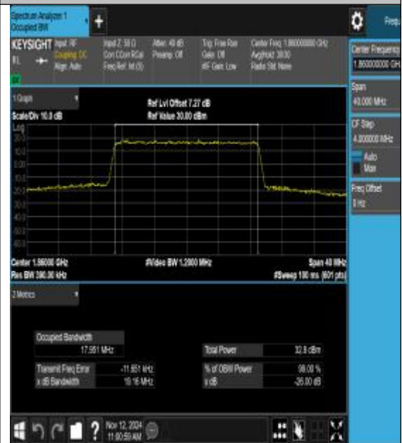
Band25-20MHz-16QAM-26140-100RB#0-PASS
