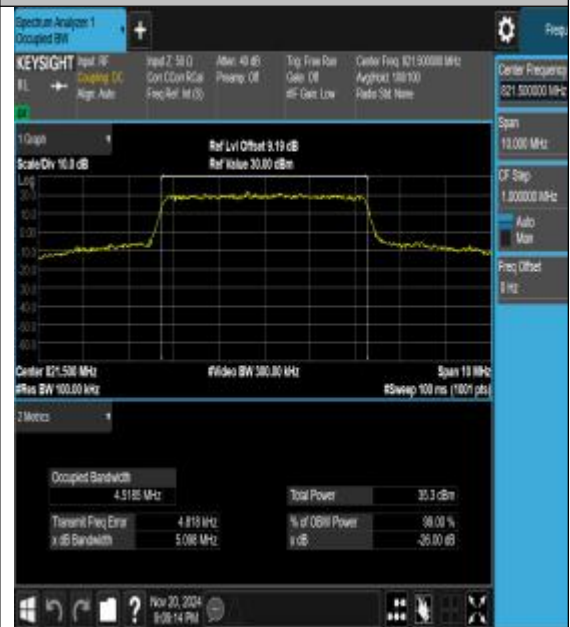
26(814-824)-5MHz-16QAM-26765-25RB#0-PASS
