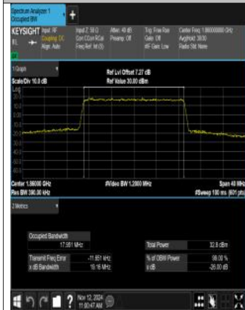
Band25-20MHz-QPSK-26140-100RB#0-PASS
