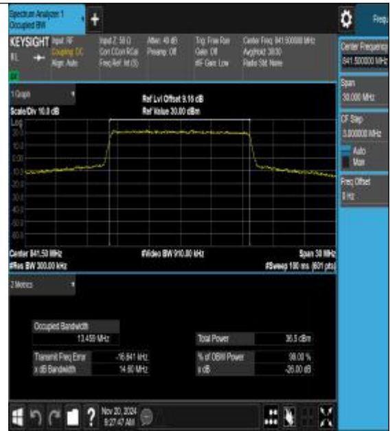
26(824-849)-15MHz-16QAM-26965-75RB#0-PAS
