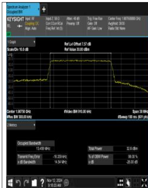
Band25-15MHz-QPSK-26615-75RB#0-PASS
