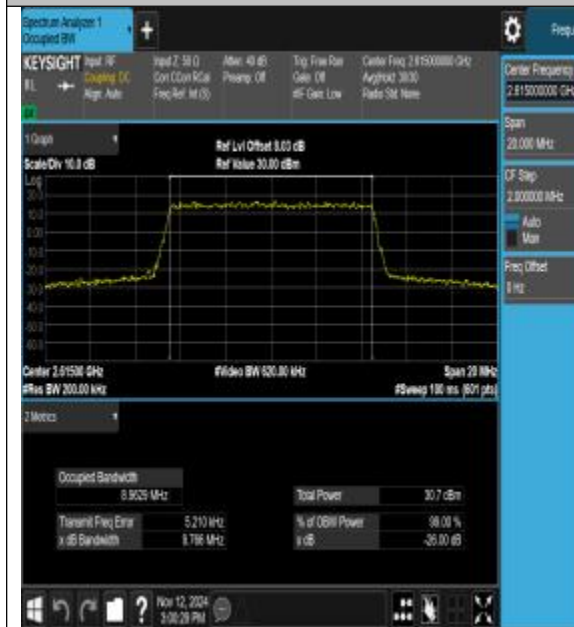
Band38-10MHz-QPSK-38200-50RB#0-PASS
