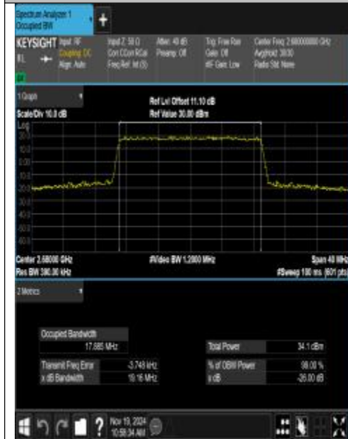
Band41-20MHz-QPSK-41490-100RB#0-PASS
