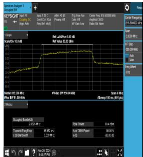
26(814-824)-3MHz-16QAM-26705-15RB#0-PASS
