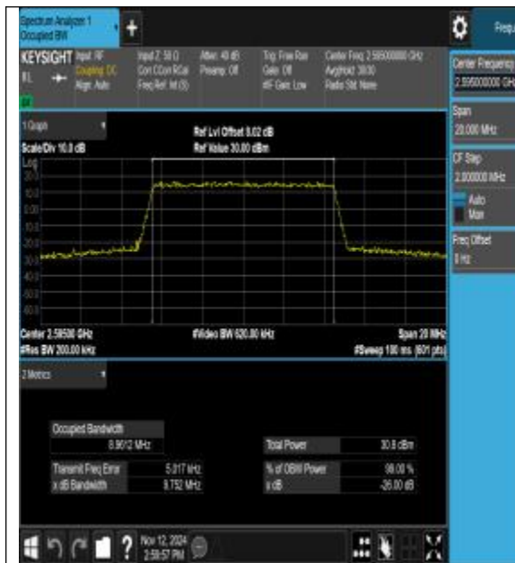
Band38-10MHz-QPSK-38000-50RB#0-PASS
