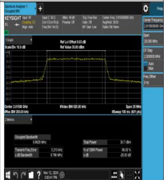
Band38-10MHz-16QAM-38200-50RB#0-PASS
