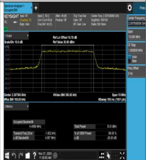
40(2305-2320)-5MHz-16QAM-38725-25RB#0-PA
