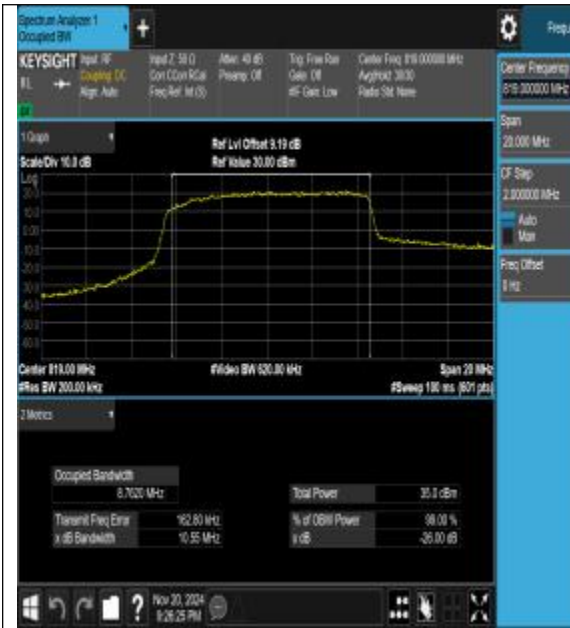
26(814-824)-10MHz-QPSK-26740-50RB#0-PASS
