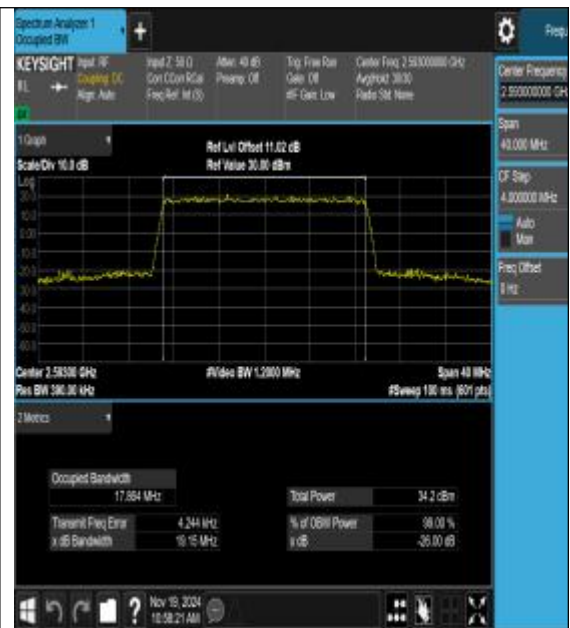
Band41-20MHz-16QAM-40620-100RB#0-PASS
