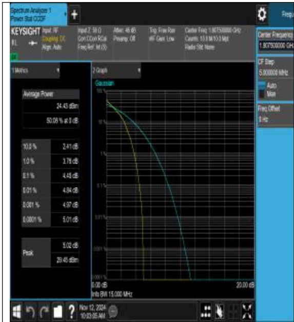
Band25-15MHz-QPSK-26615-1RB#0-PASS
