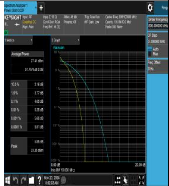
26(824-849)-10MHz-16QAM-26915-50RB#0-PAS
