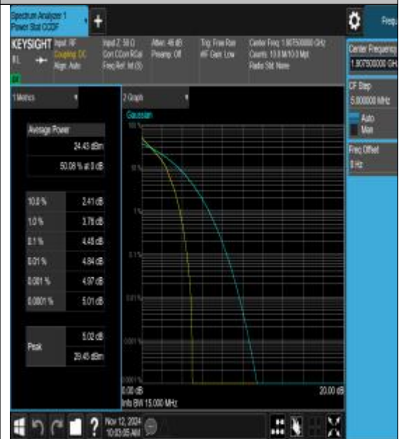
Band25-15MHz-16QAM-26615-75RB#0-PASS
