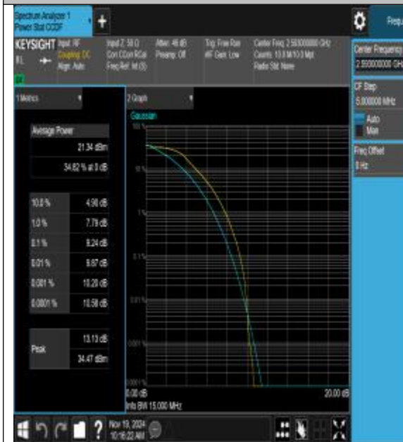
Band41-15MHz-QPSK-40620-75RB#0-PASS
