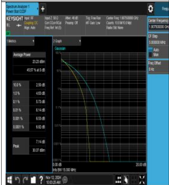
Band25-15MHz-QPSK-26615-75RB#0-PASS
