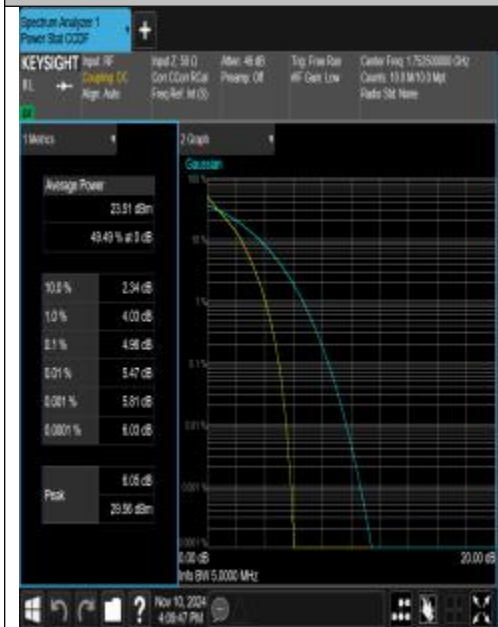
Band4-5MHz-QPSK-20375-25RB#0-PASS
