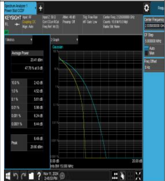
Band7-15MHz-16QAM-20825-75RB#0-PASS
