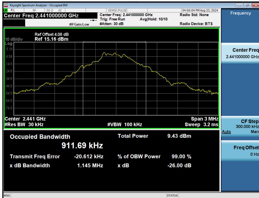
99%_Occupied_Bandwidth_NVNT_ANT1_1-DH1_2441_00
