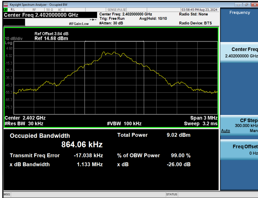
99%_Occupied_Bandwidth_NVNT_ANT1_1-DH1_2402_00
