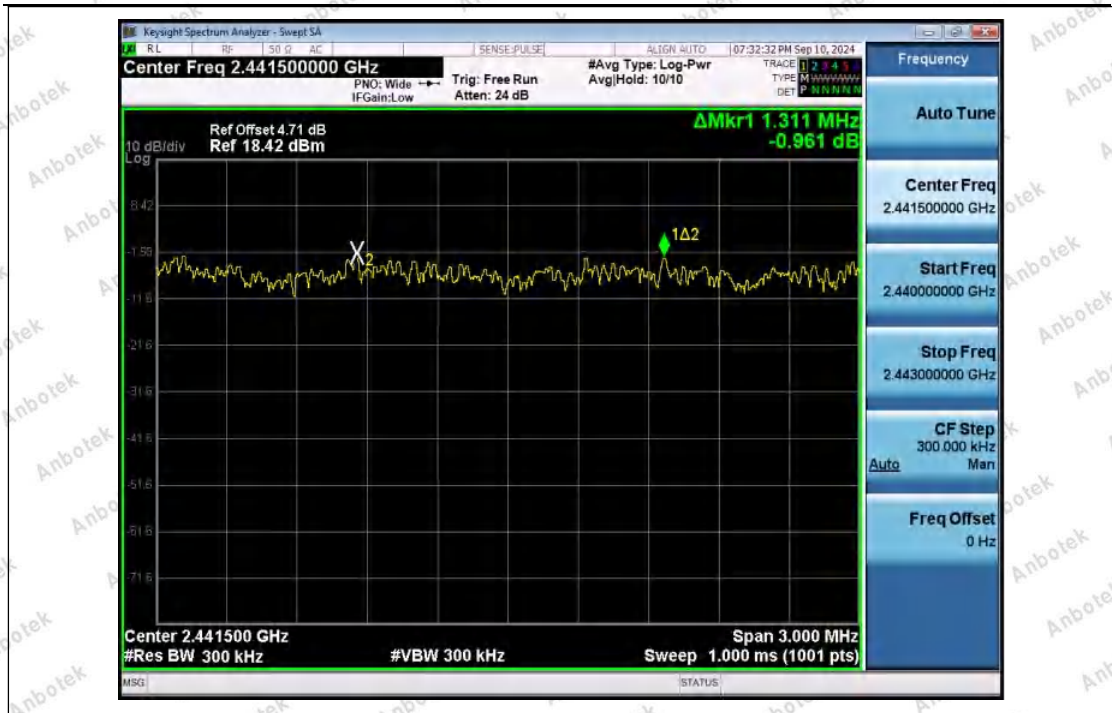
Carrier_Frequencies_Separation_(Hopping)_NVNT_ANT1_3-DH5_Hopping
