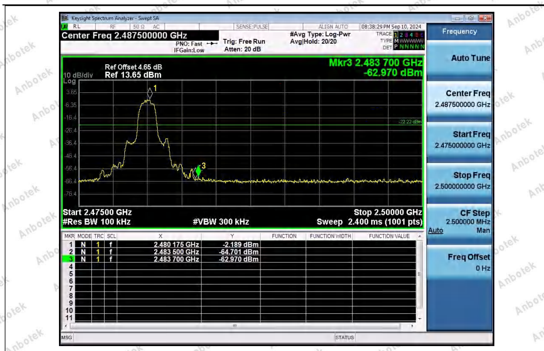
1_Reference_Level_Hopping_NVNT_ANT1_3-DH5_Hopping
