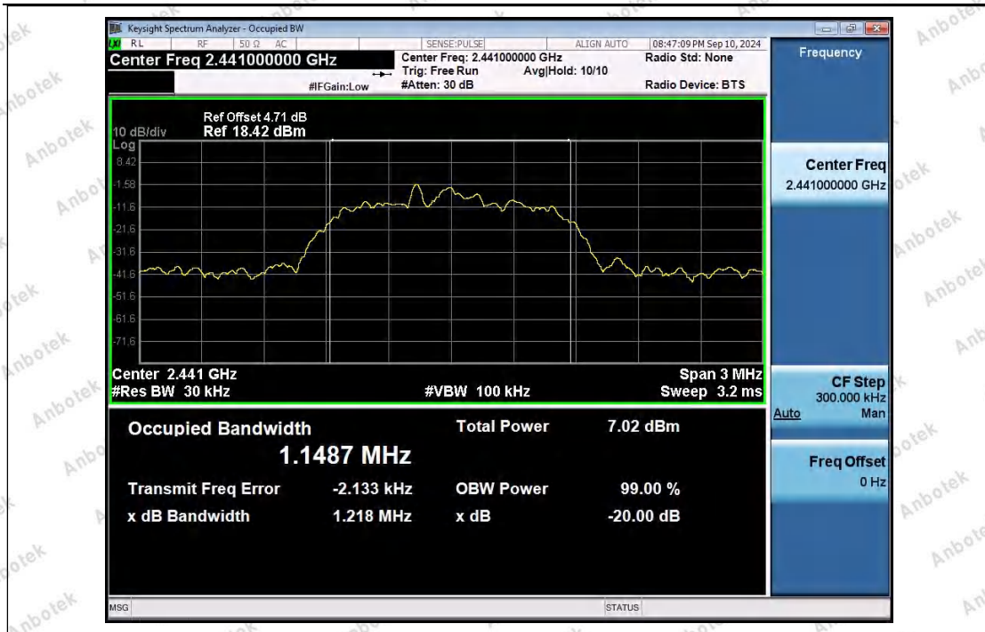
-20dB_Bandwidth_NVNT_ANT1_3-DH3_2441_00
