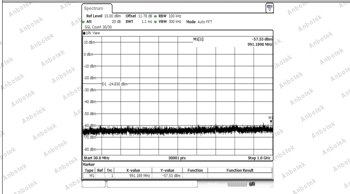
3DH5-Ant1-2402-30~1000-PASS
