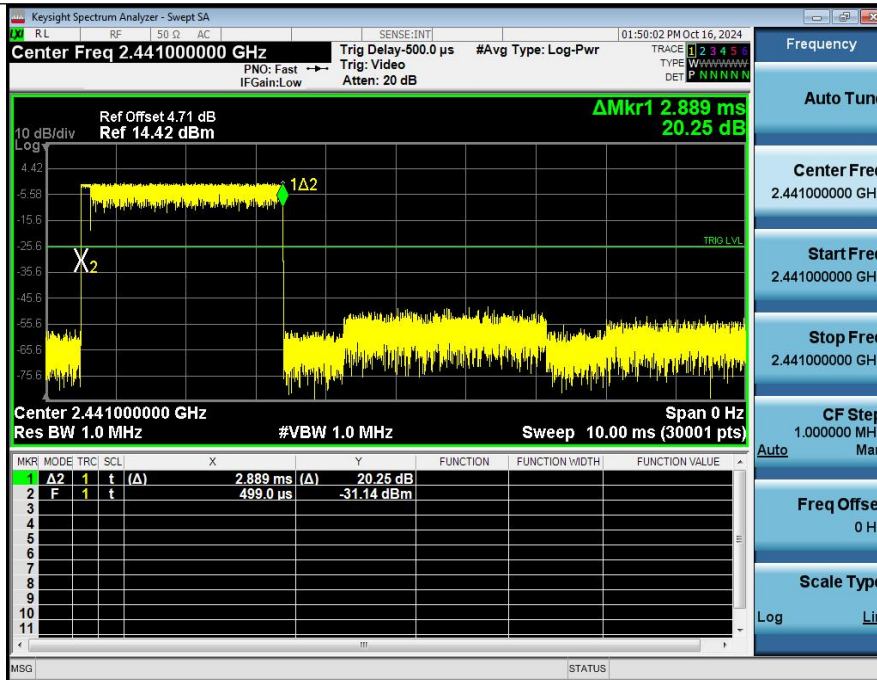
Dwell_Time (Hopping)_NVNT_ANT1_2-DH5_2441_00_Accumulated
