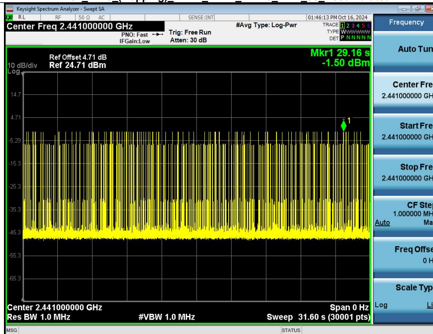
Dwell_Time (Hopping)_NVNT_ANT1_2-DH5_2441_00_Accumulated
