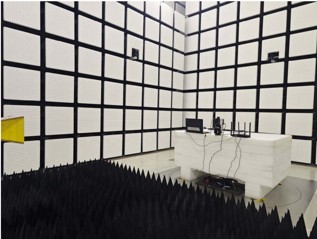
Radiated Emissions Above 1G Rear View-M4 0.5m Cable
