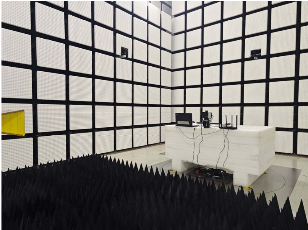
Radiated Emissions Above 1G Rear View-M5 0.5m Cable
