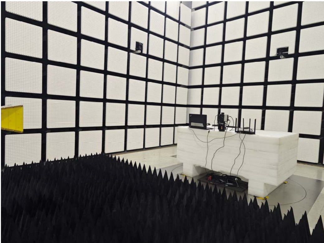
Radiated Emissions Above 1G Rear View-M3 0.5m Cable
