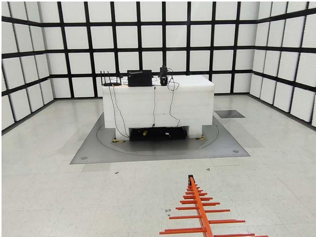
Radiated Emissions Below 1G Rear View-M1 0.5m Cable
