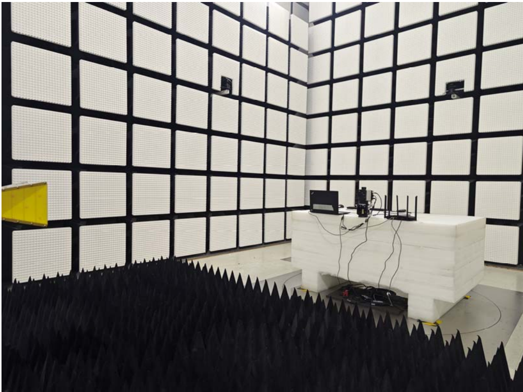
Radiated Emissions Above 1G Rear View-M1 2m Cable
