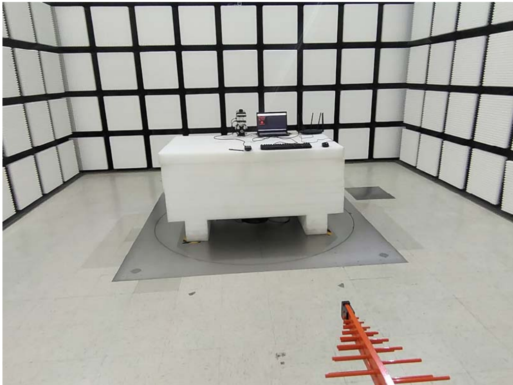
Radiated Emissions Below 1G Rear View-M3 0.5m Cable
