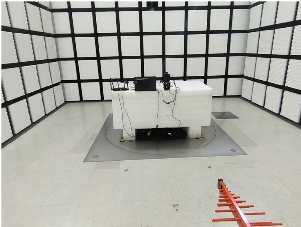
Radiated Emissions Below 1G Rear View-M1 2m Cable
