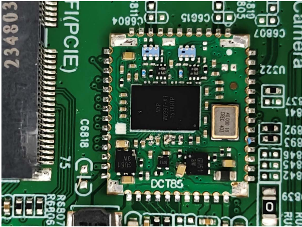
Internal Photos M/N: RK3588.3_004
