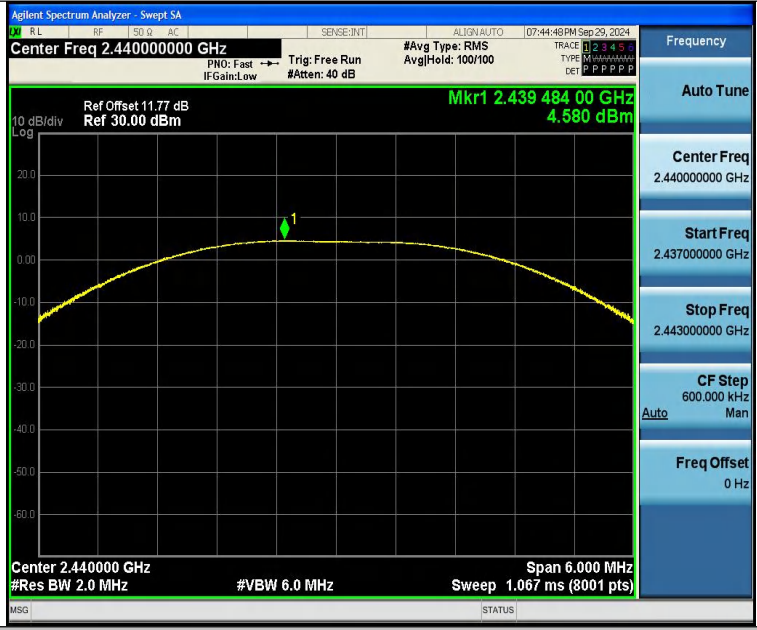
BLE_2M-Ant1-2440-PASS
