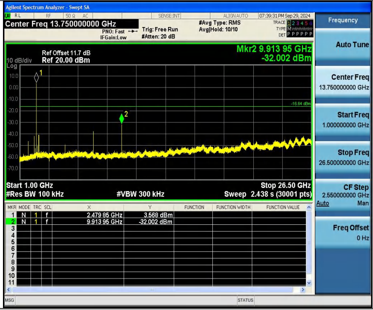
BLE_1M-Ant1-2480-1000~26500-PASS
