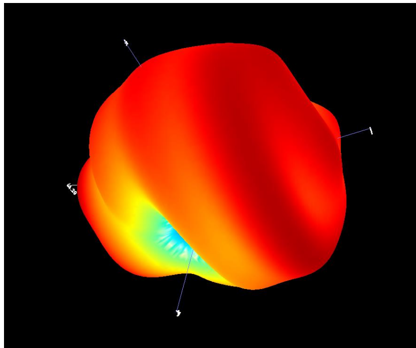
B1.2 3D Pattern for 450MHz
