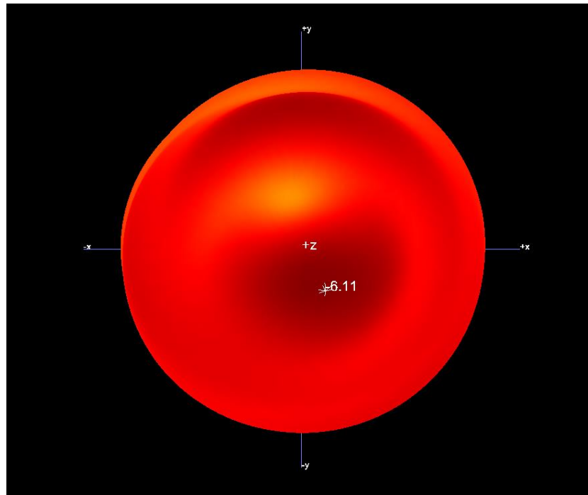
B1.1 3D Pattern for 400MHz
