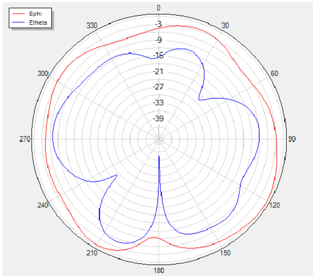
Phi=90 freq=2500MHz
