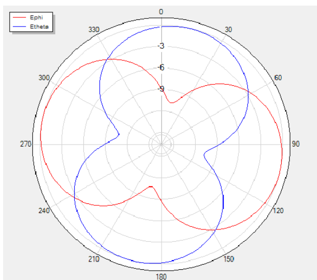
Theta=0 freq=2450MHz
