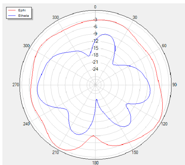
Phi=90 freq=2450MHz
