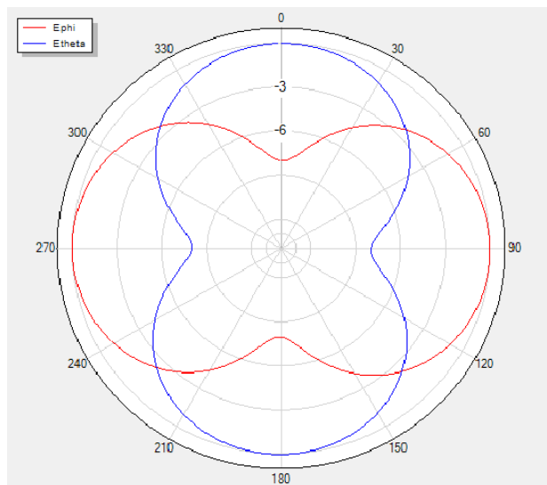
Theta=0 freq=2400MHz
