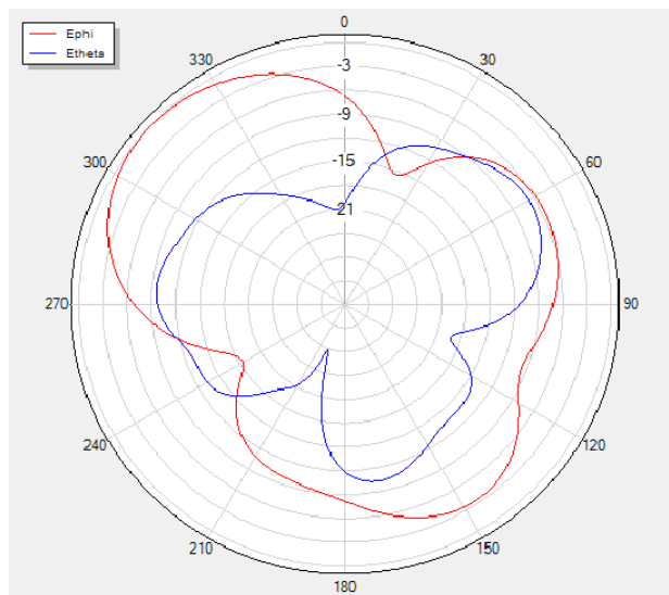
Theta=90 freq=2450MHz
