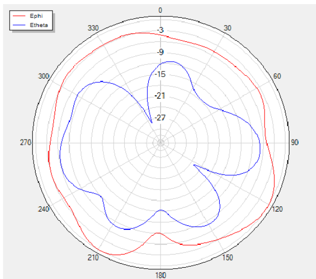
Phi=90 freq=2400MHz
