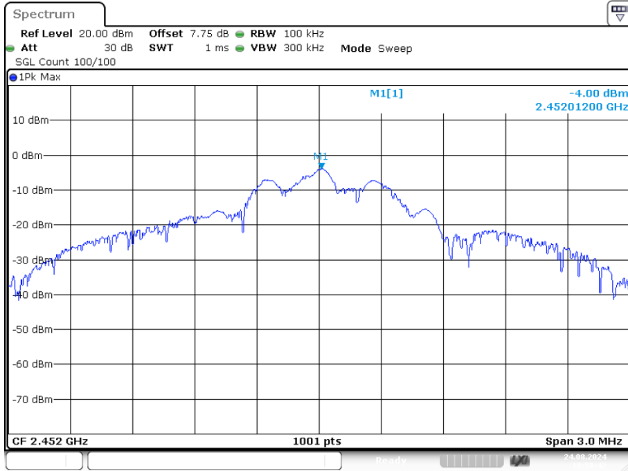
Tx. Spurious NVNT GFSK 2452MHz Ant1 Ref
