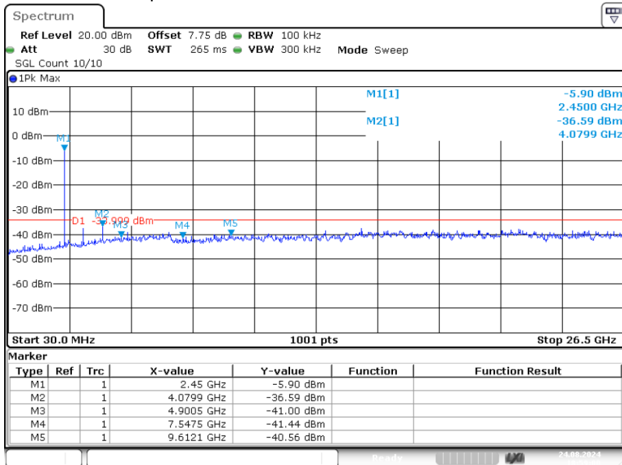
Tx. Spurious NVNT GFSK 2452MHz Ant1 Emission
