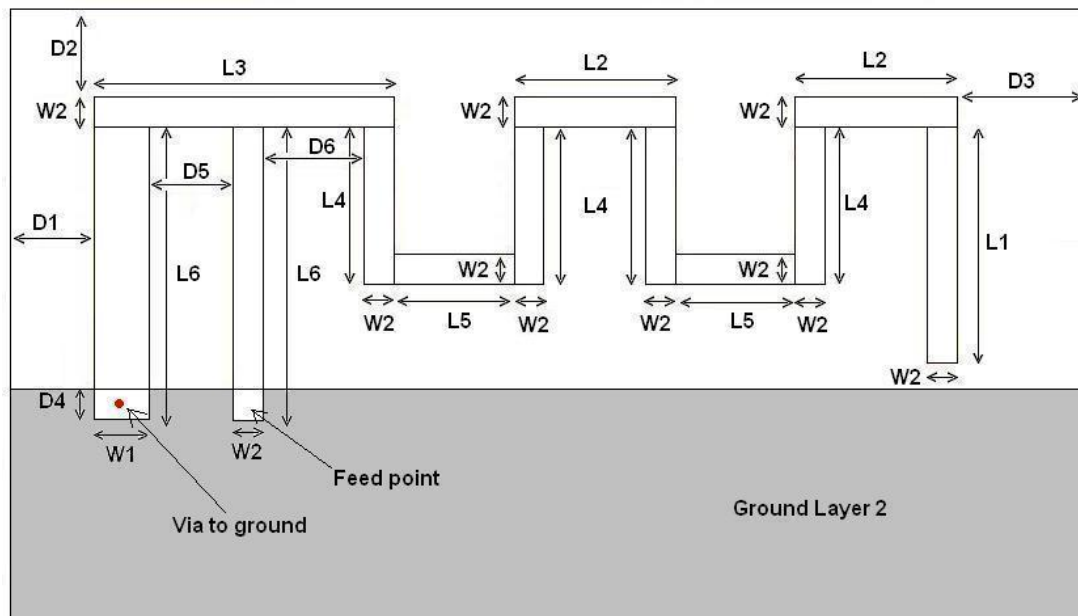
Figure 3: Antenna Dimensions
