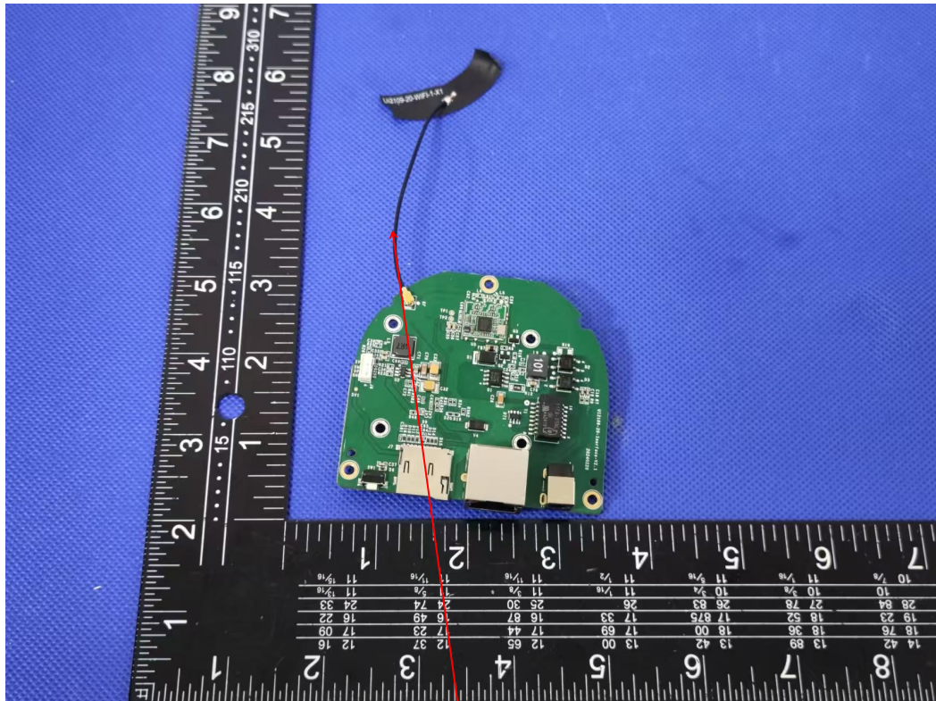
WiFi antenna
