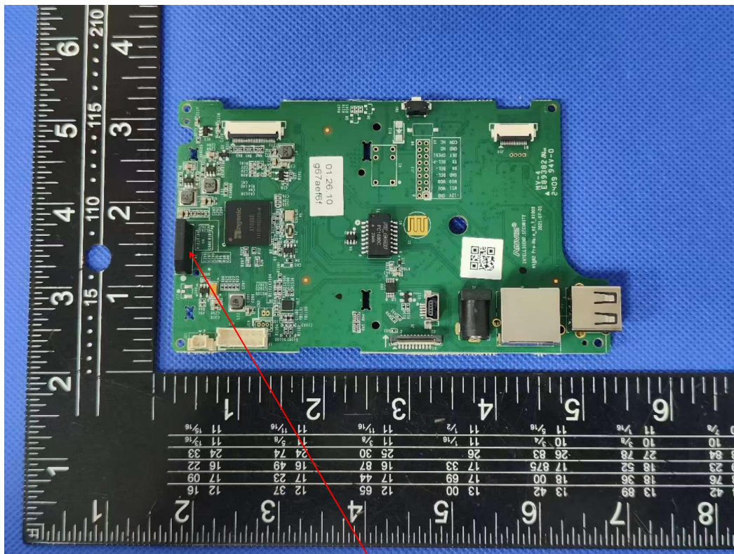
WIFI ANT
