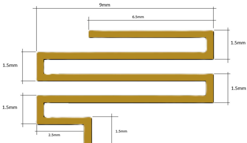
Figure 2 – PCB antenna dimension
