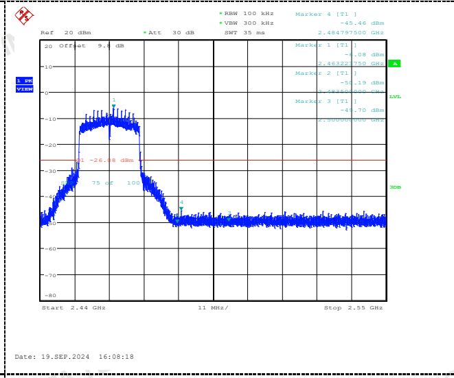
Right bandedge
