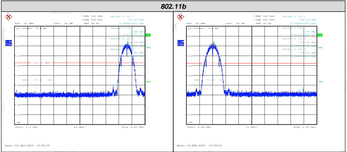
Left bandedge
