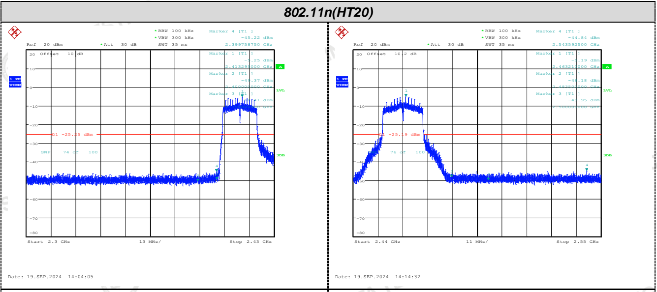
Left bandedge
