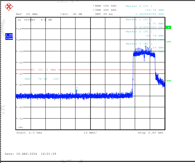
Left bandedge
