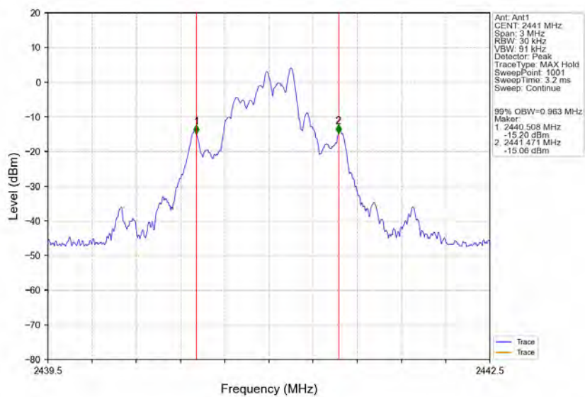
GFSK_DH5_MCH_2441MHz_Ant1_NTNV
