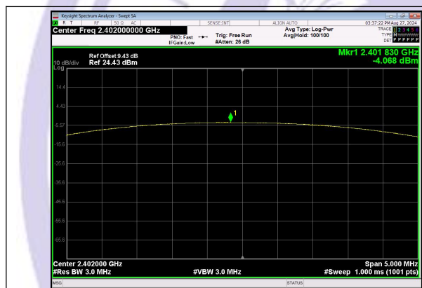
Peak Output Power GFSK_Channel 0
